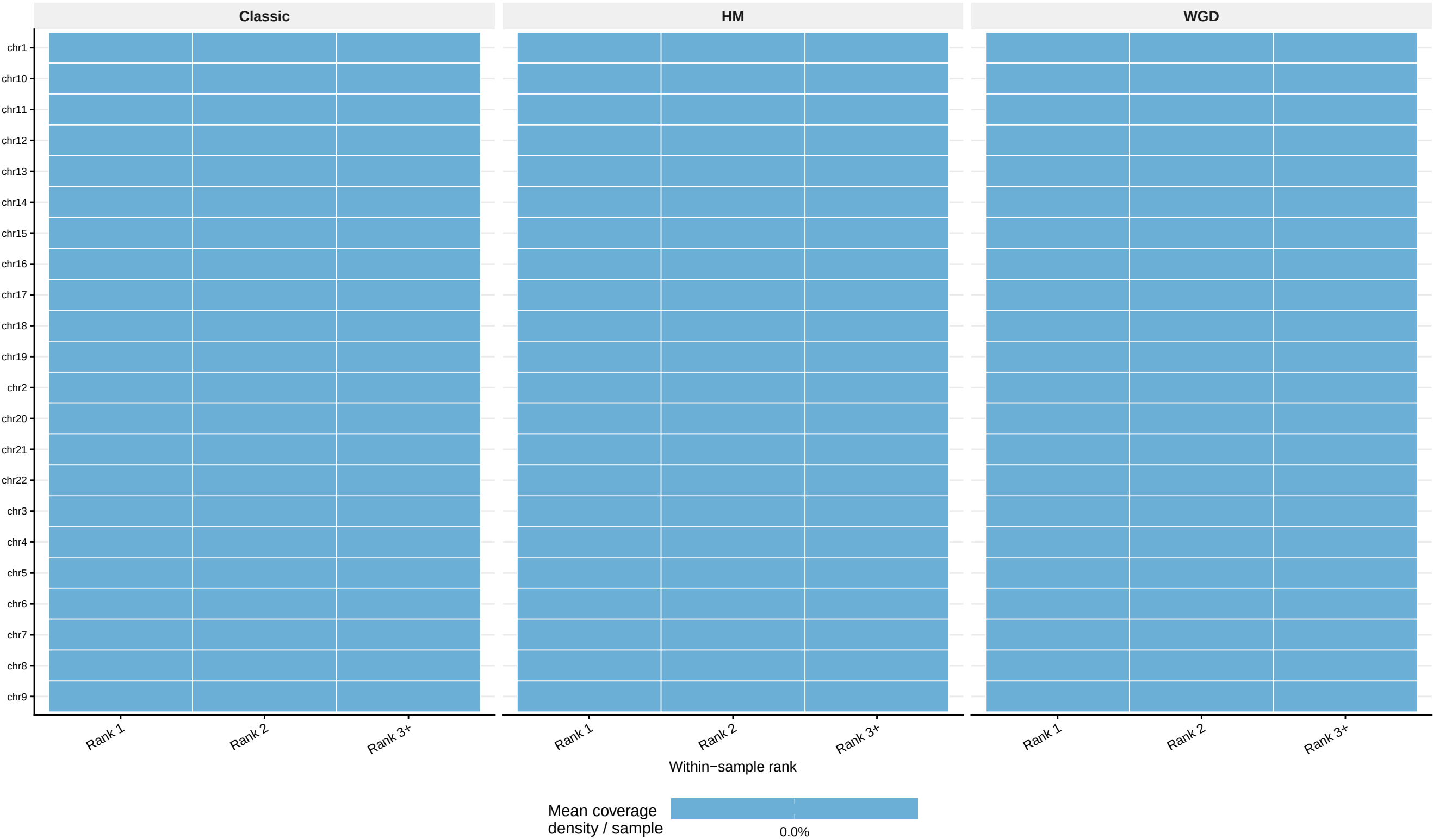
Chromosome coverage density by class × within-sample rank Colour = \text{sum(seg length)} / \text{chr length} / \text{n\_samples} | Stars = Wilcoxon vs row median (BH-corrected): * p<0.05, ** p<0.01, *** p<0.001
