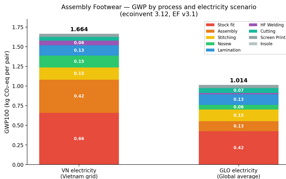
Fig. 1 — GWP100 by process and electricity scenario (ecoinvent 3.12, EF v3.1)
