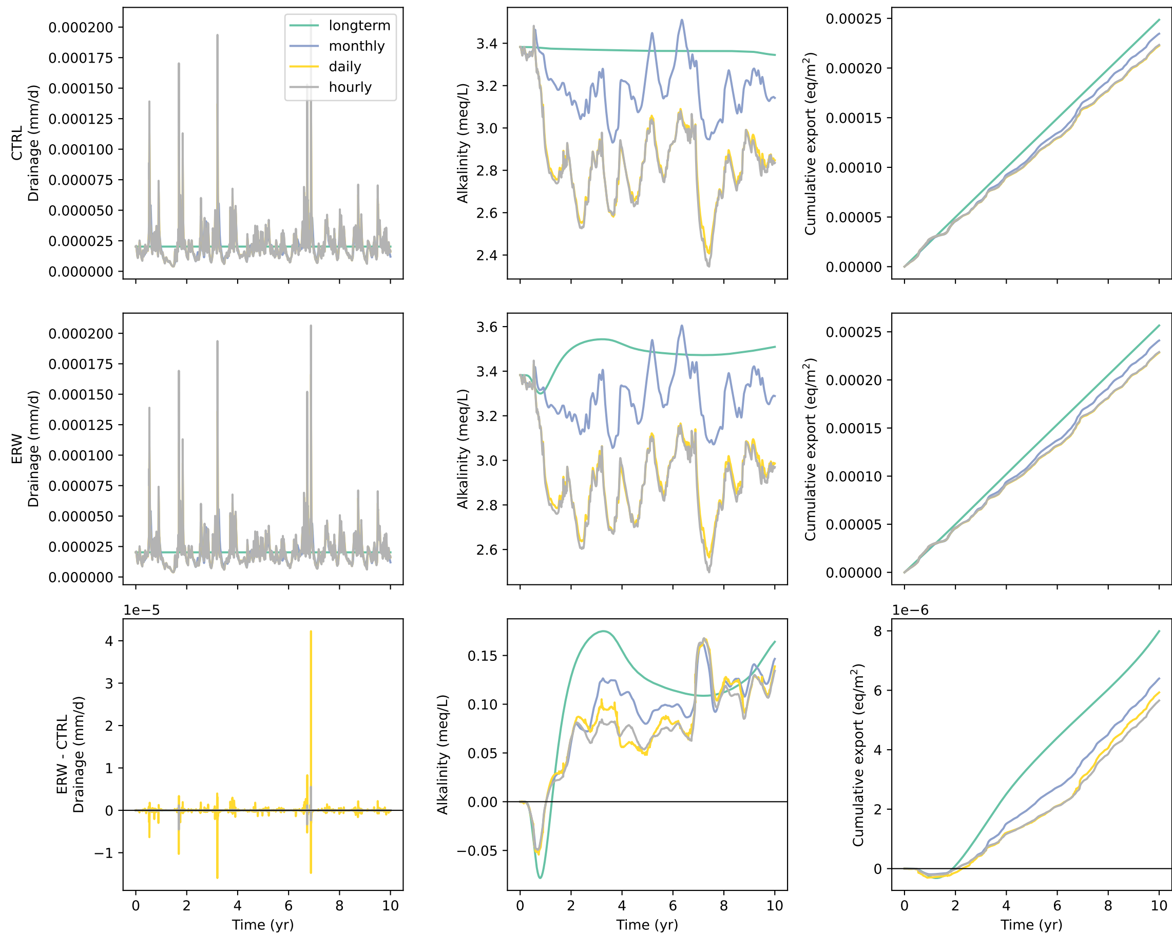
Flanagan: drainage and alkalinity export at 200 cm
