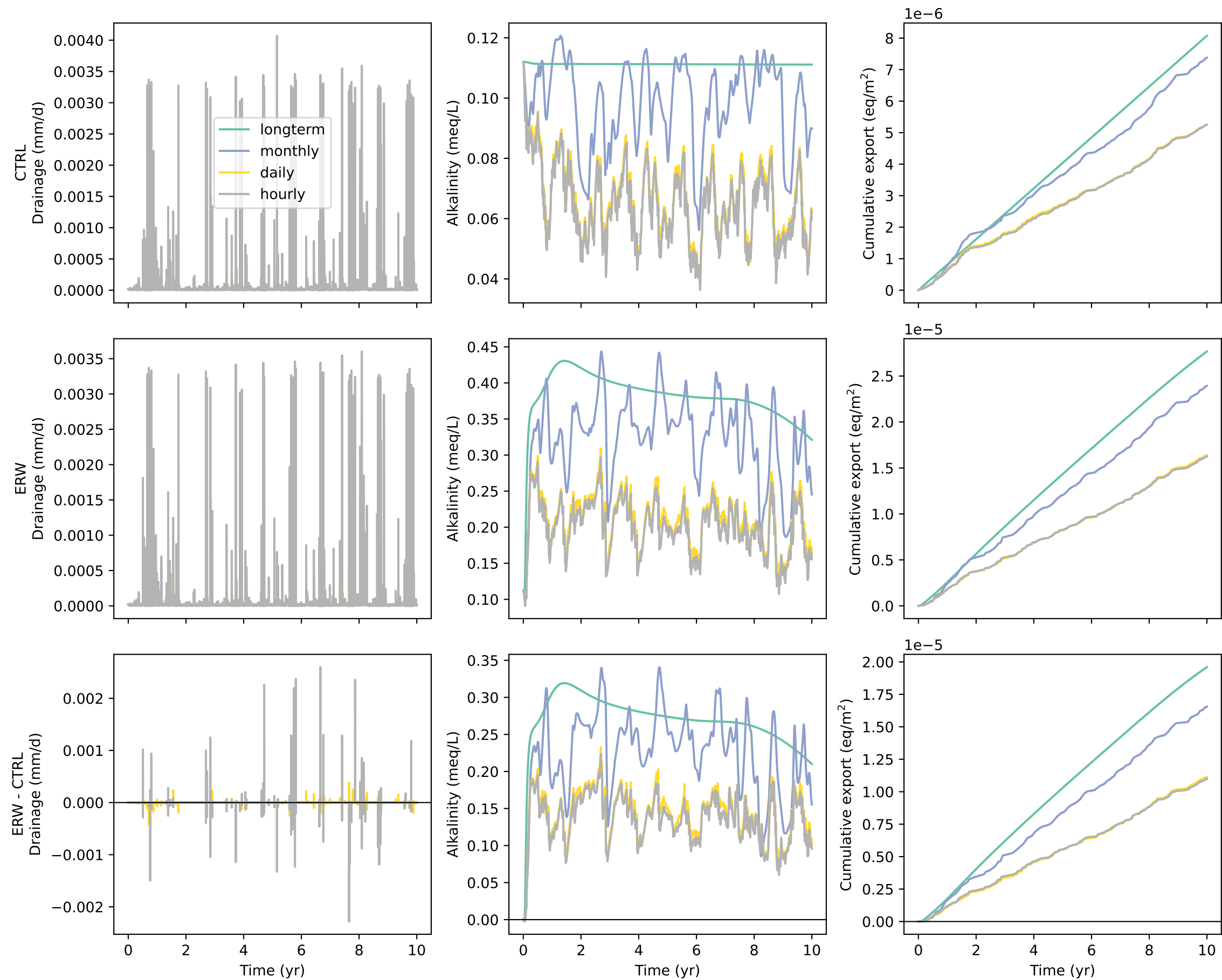
Cecil: drainage and alkalinity export at 50 cm
