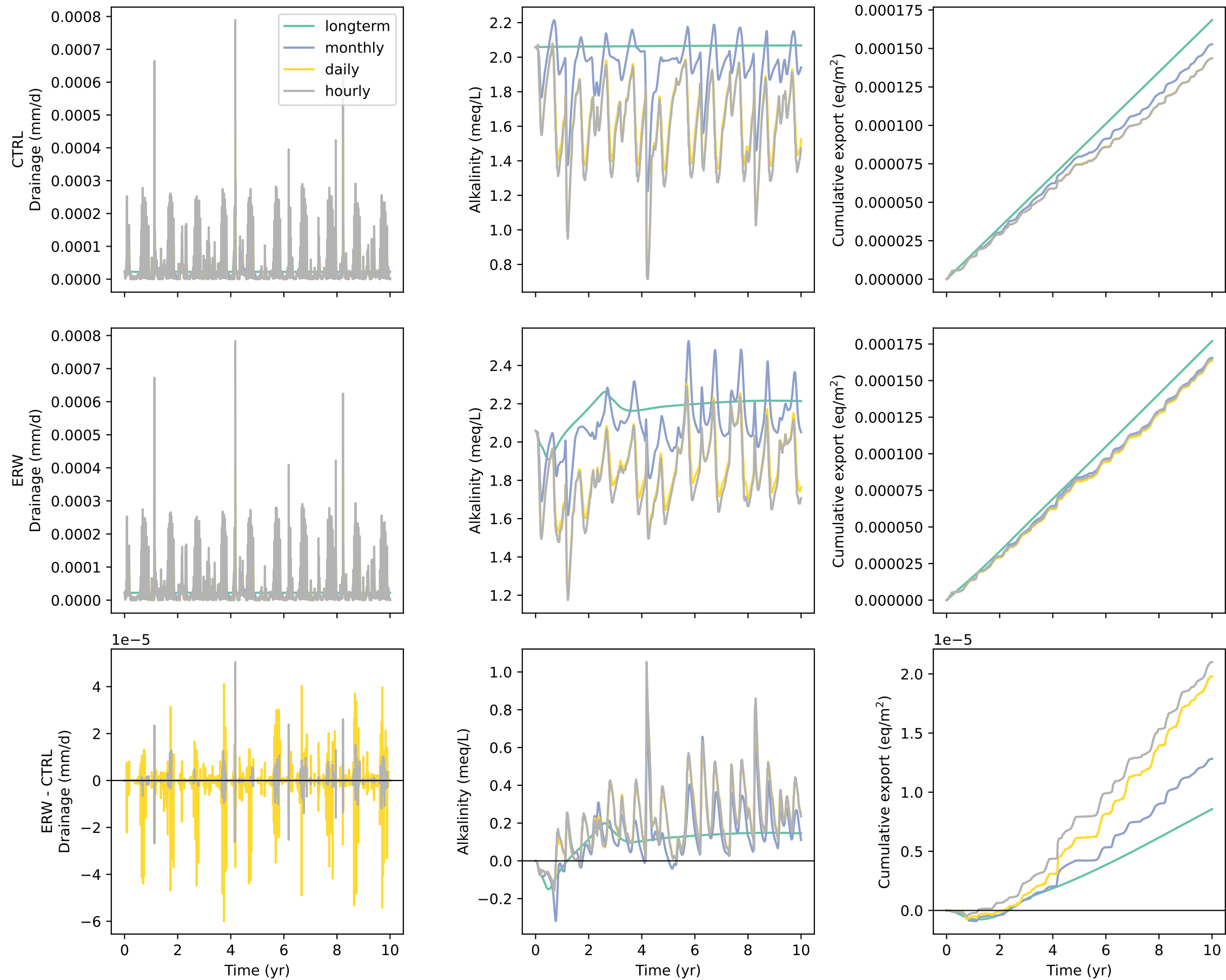
Yolo: drainage and alkalinity export at 100 cm
