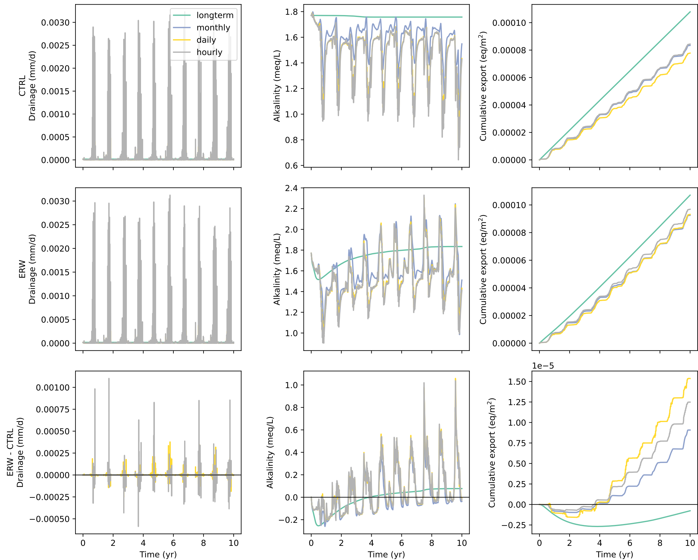
Kuma: drainage and alkalinity export at 50 cm
