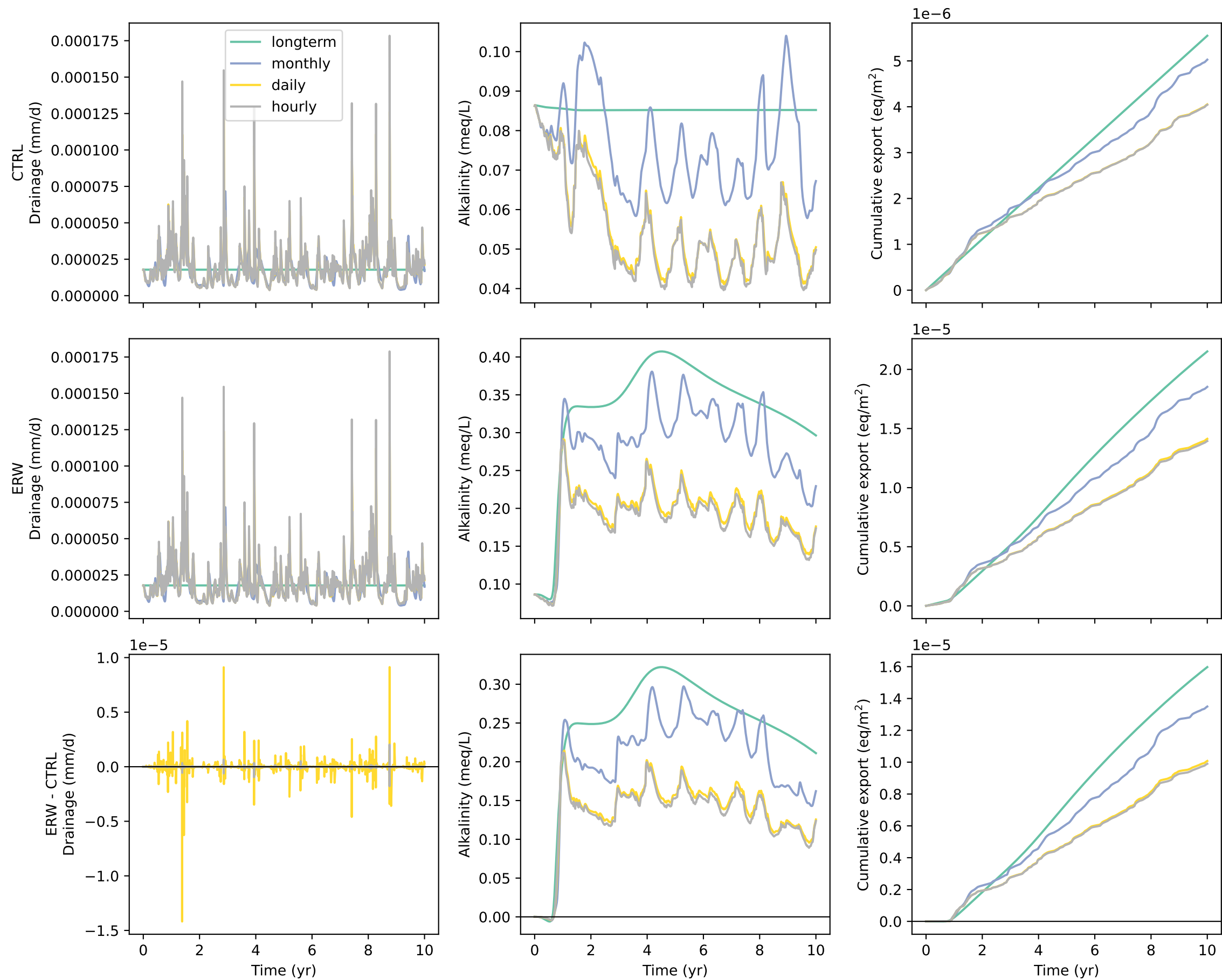
Cecil: drainage and alkalinity export at 200 cm
