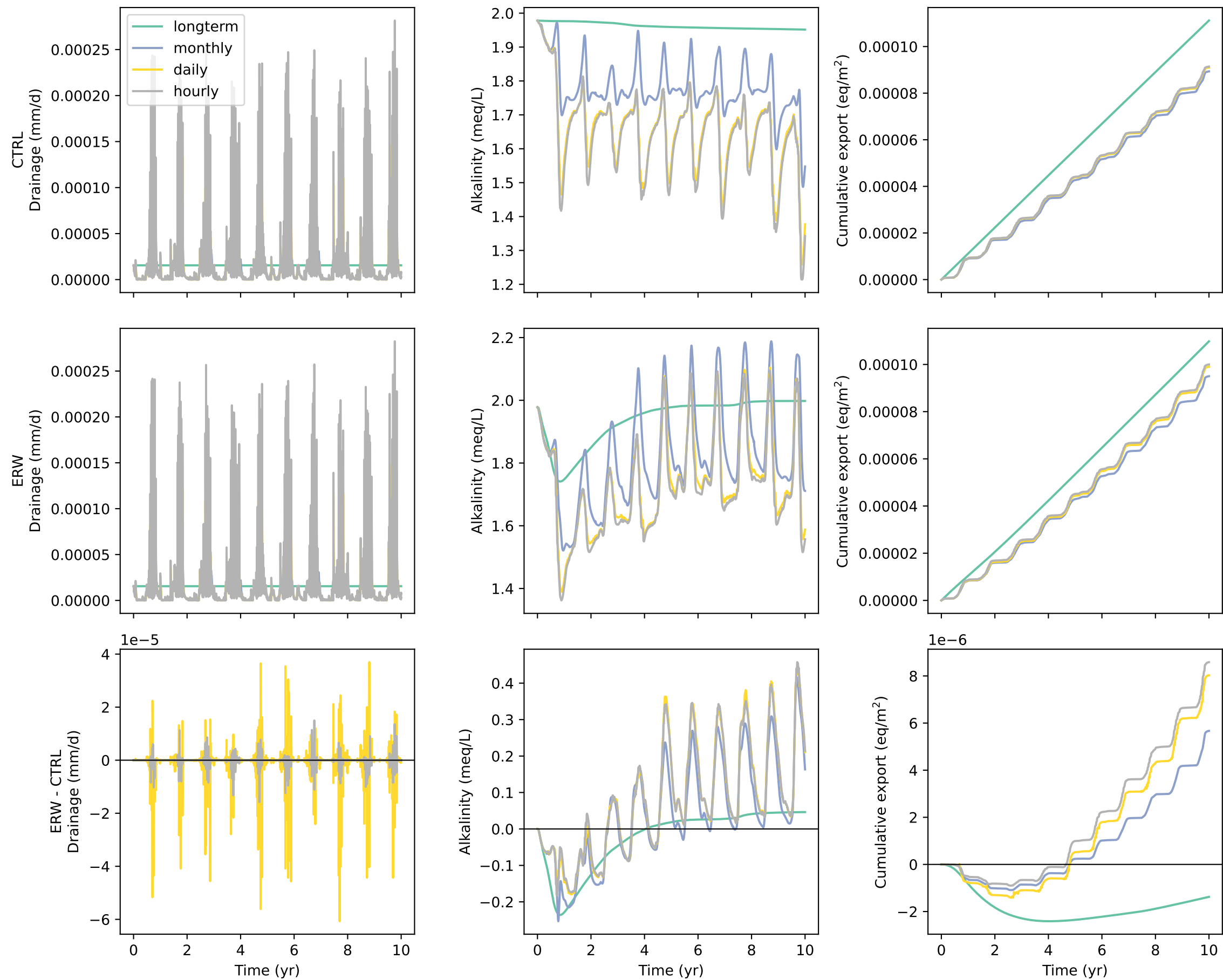
Kuma: drainage and alkalinity export at 100 cm
