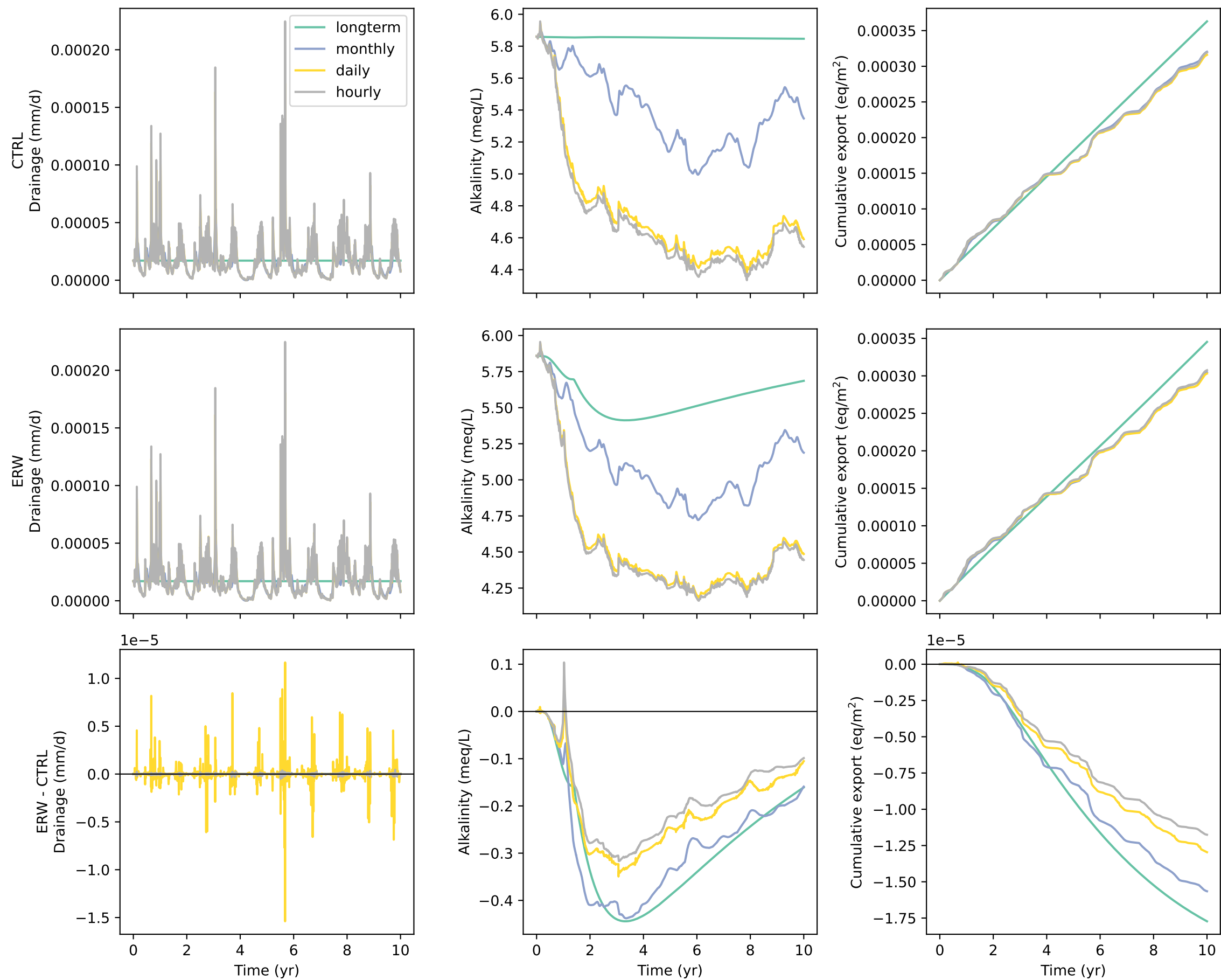
HoustonBlack: drainage and alkalinity export at 200 cm
