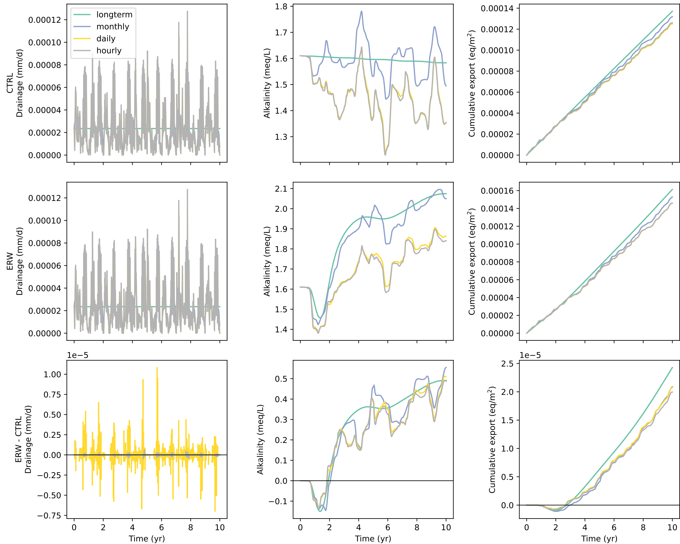
Palouse: drainage and alkalinity export at 300 cm
