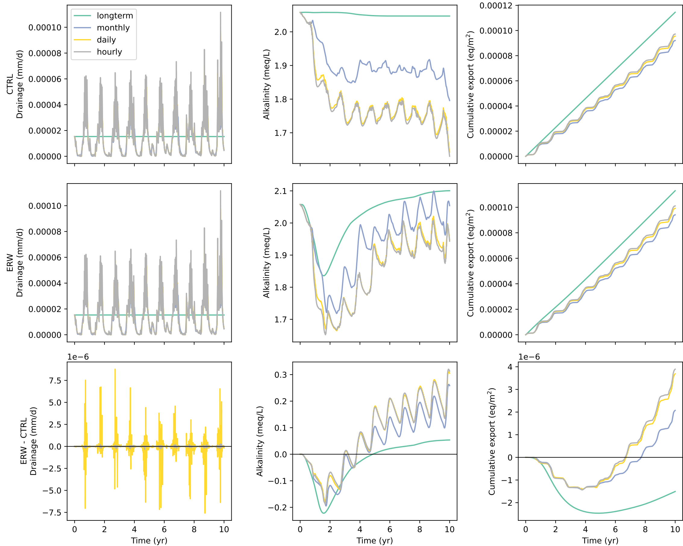
Kuma: drainage and alkalinity export at 200 cm
