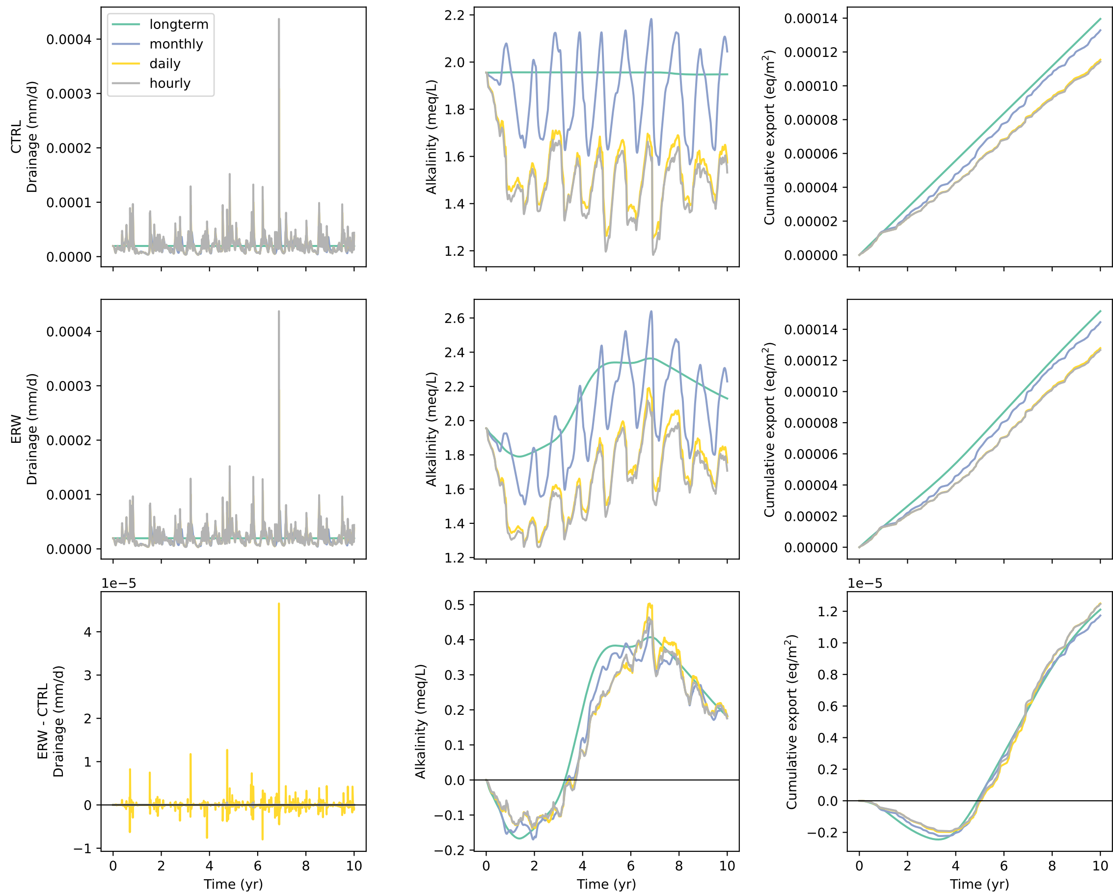
Kalamazoo: drainage and alkalinity export at 300 cm
