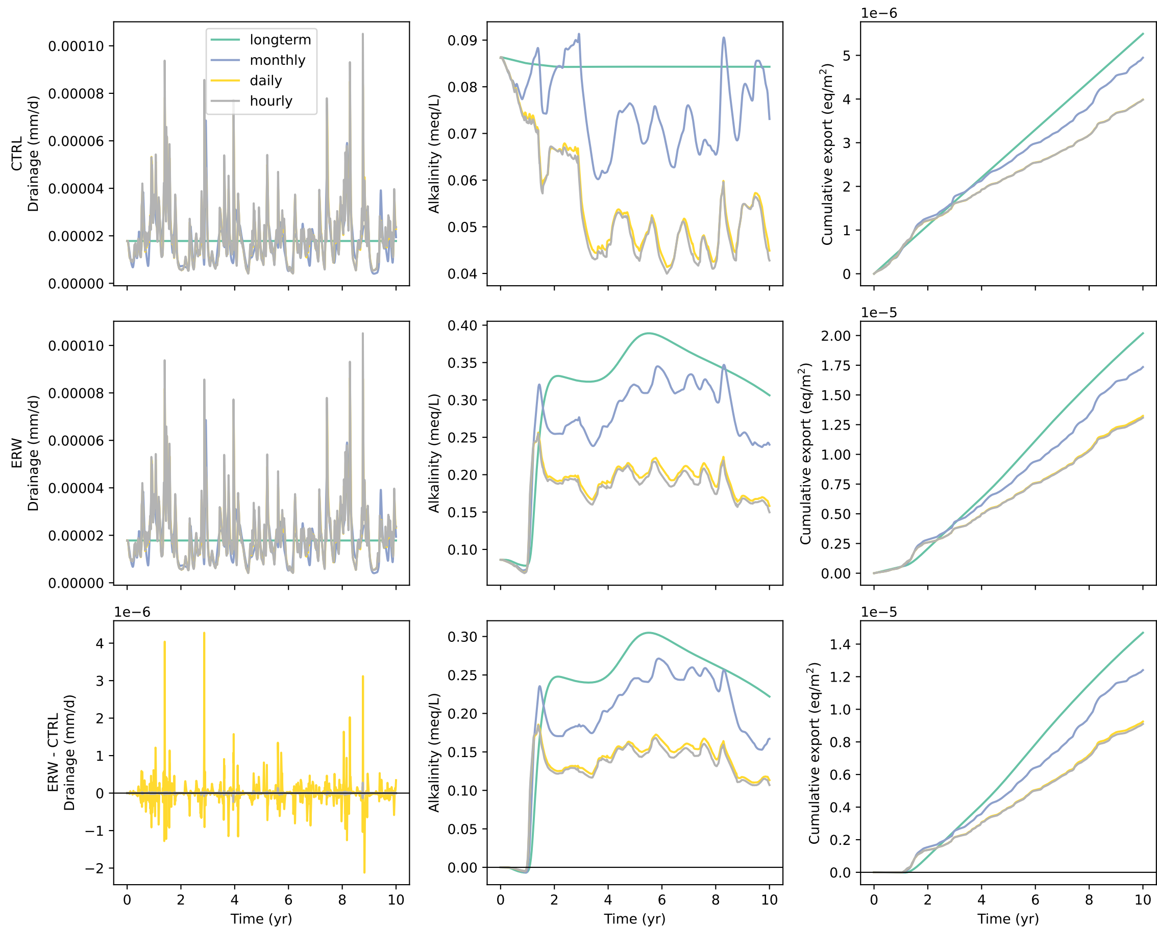
Cecil: drainage and alkalinity export at 300 cm
