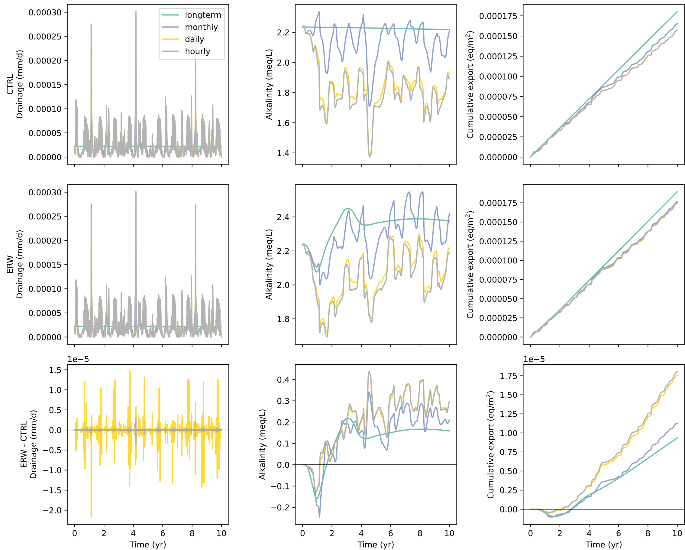
Yolo: drainage and alkalinity export at 200 cm
