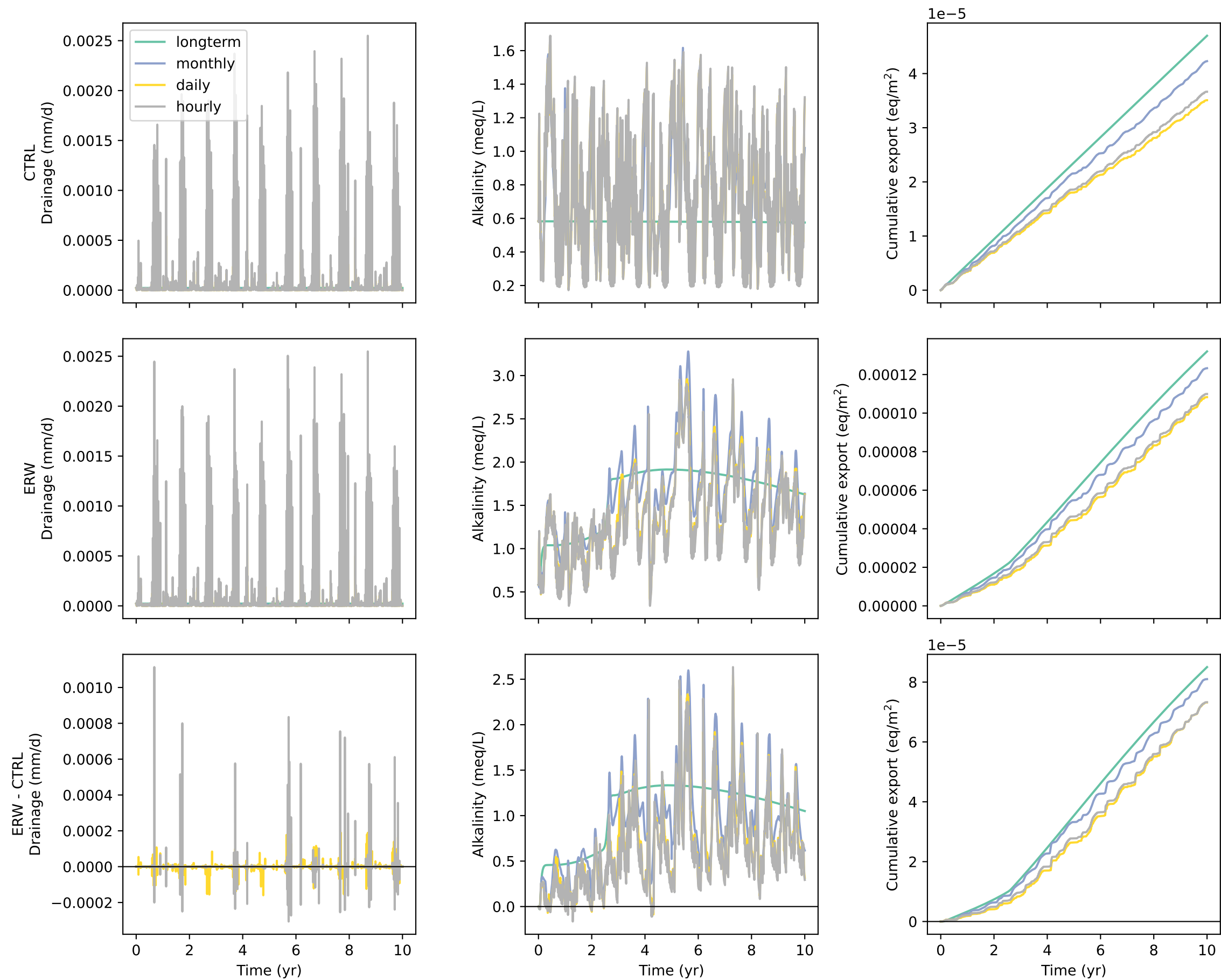
Yolo: drainage and alkalinity export at 50 cm
