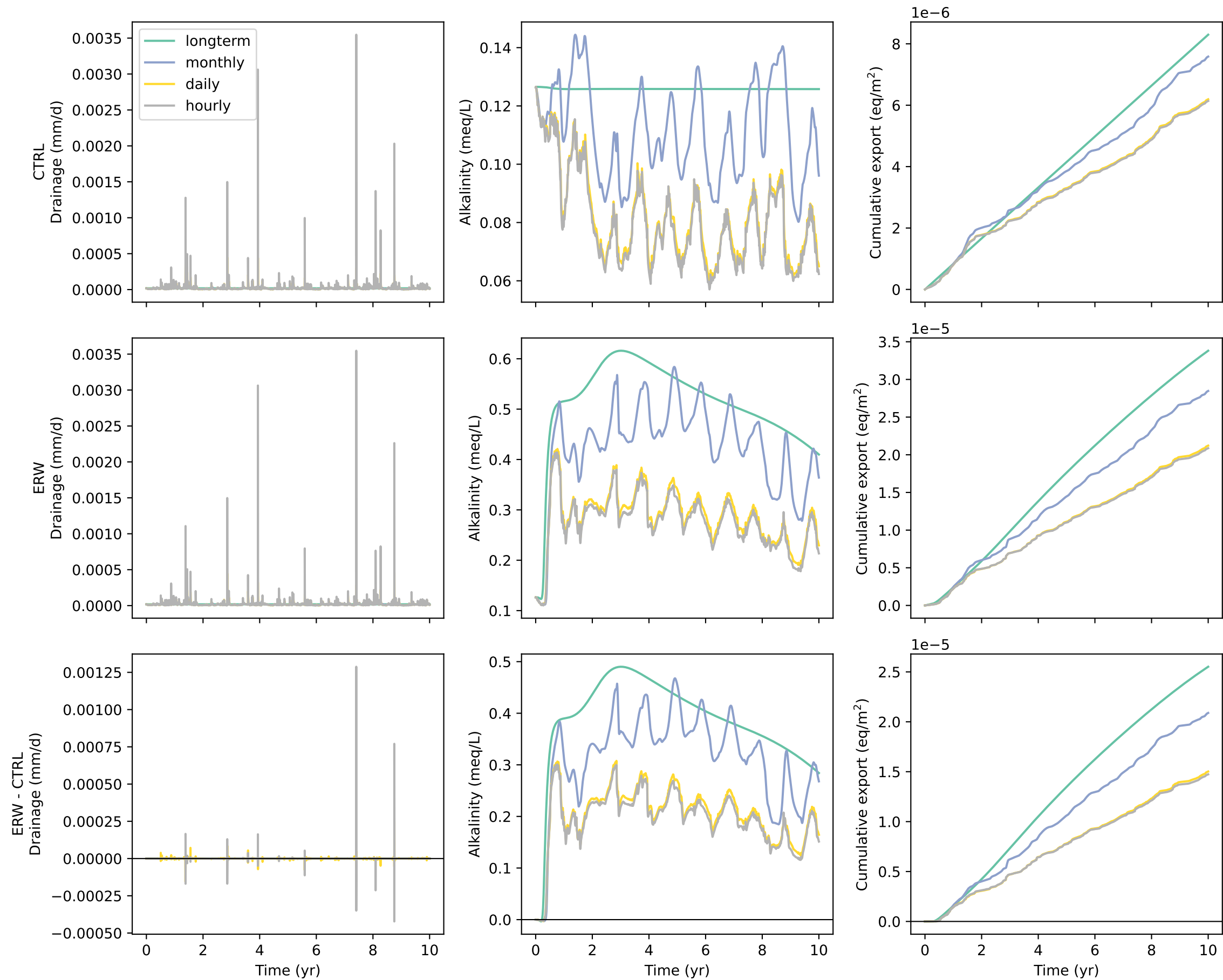
Cecil: drainage and alkalinity export at 100 cm
