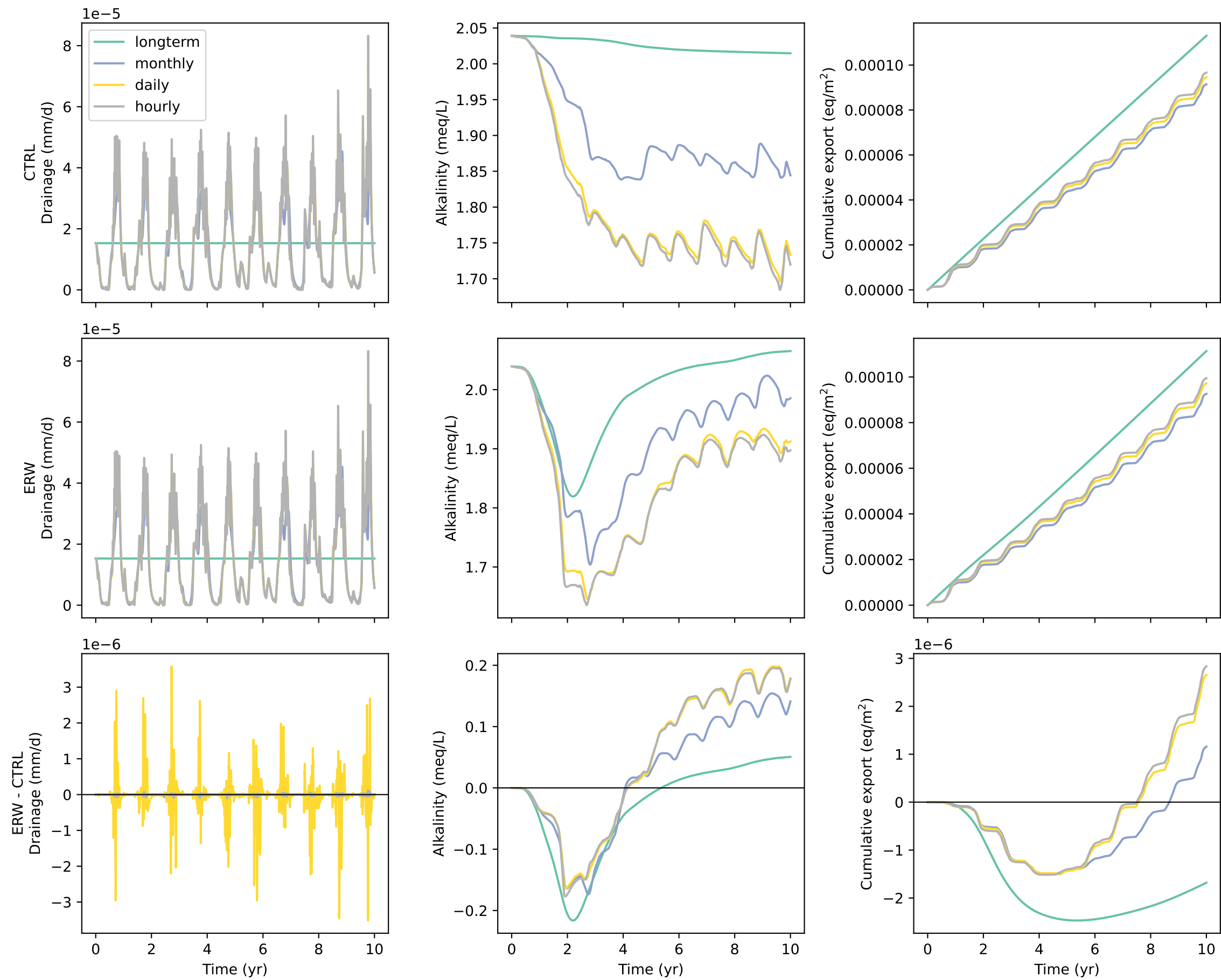
Kuma: drainage and alkalinity export at 300 cm
