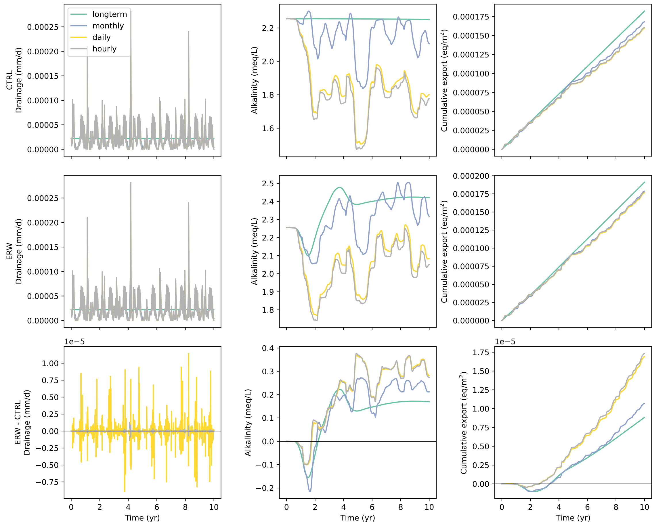
Yolo: drainage and alkalinity export at 300 cm
