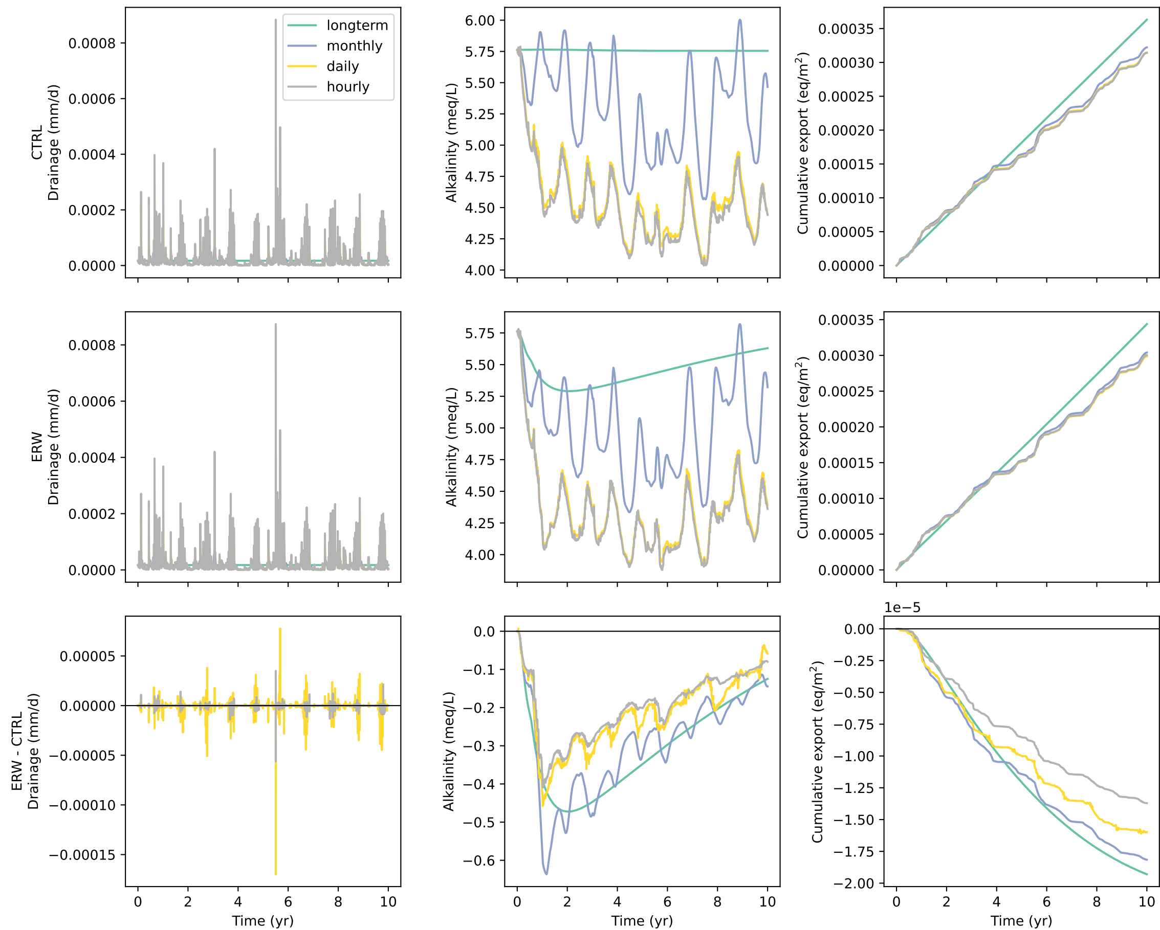
HoustonBlack: drainage and alkalinity export at 100 cm
