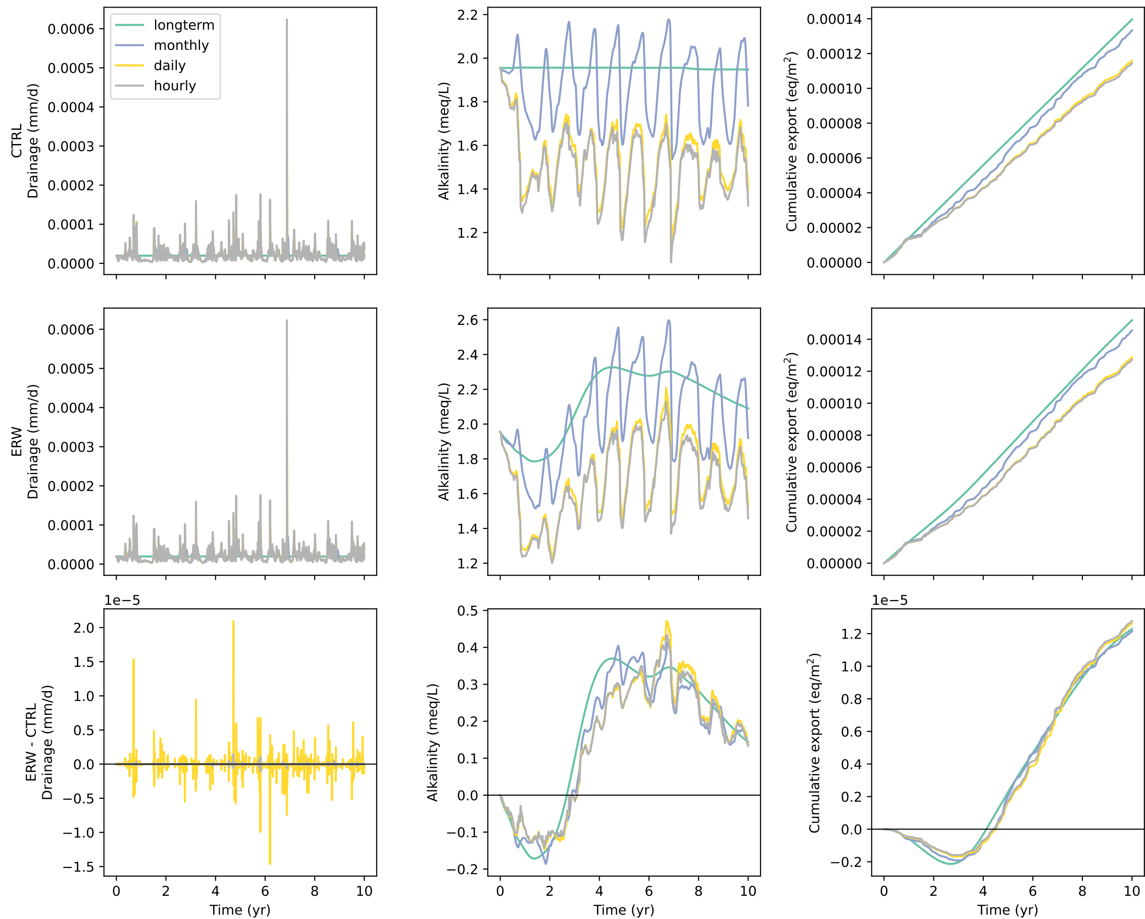
Kalamazoo: drainage and alkalinity export at 200 cm
