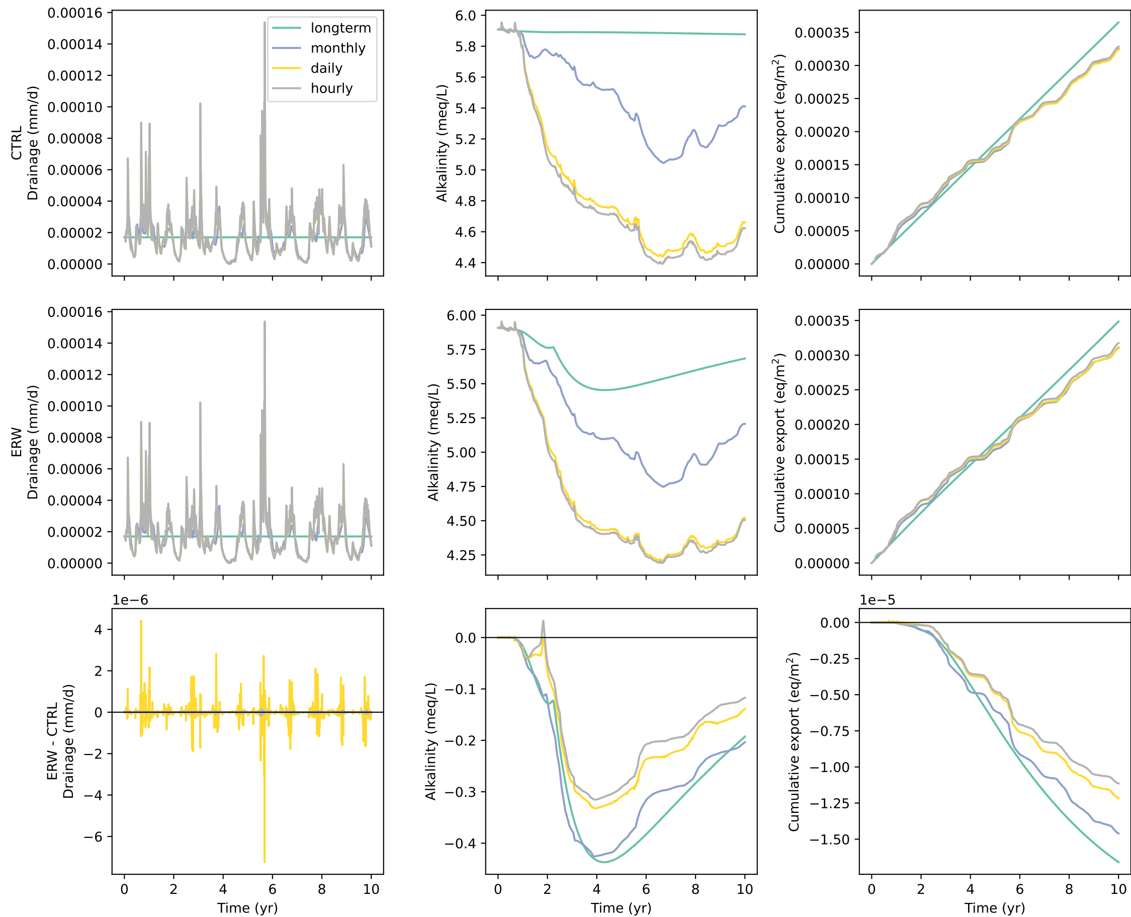
HoustonBlack: drainage and alkalinity export at 300 cm
