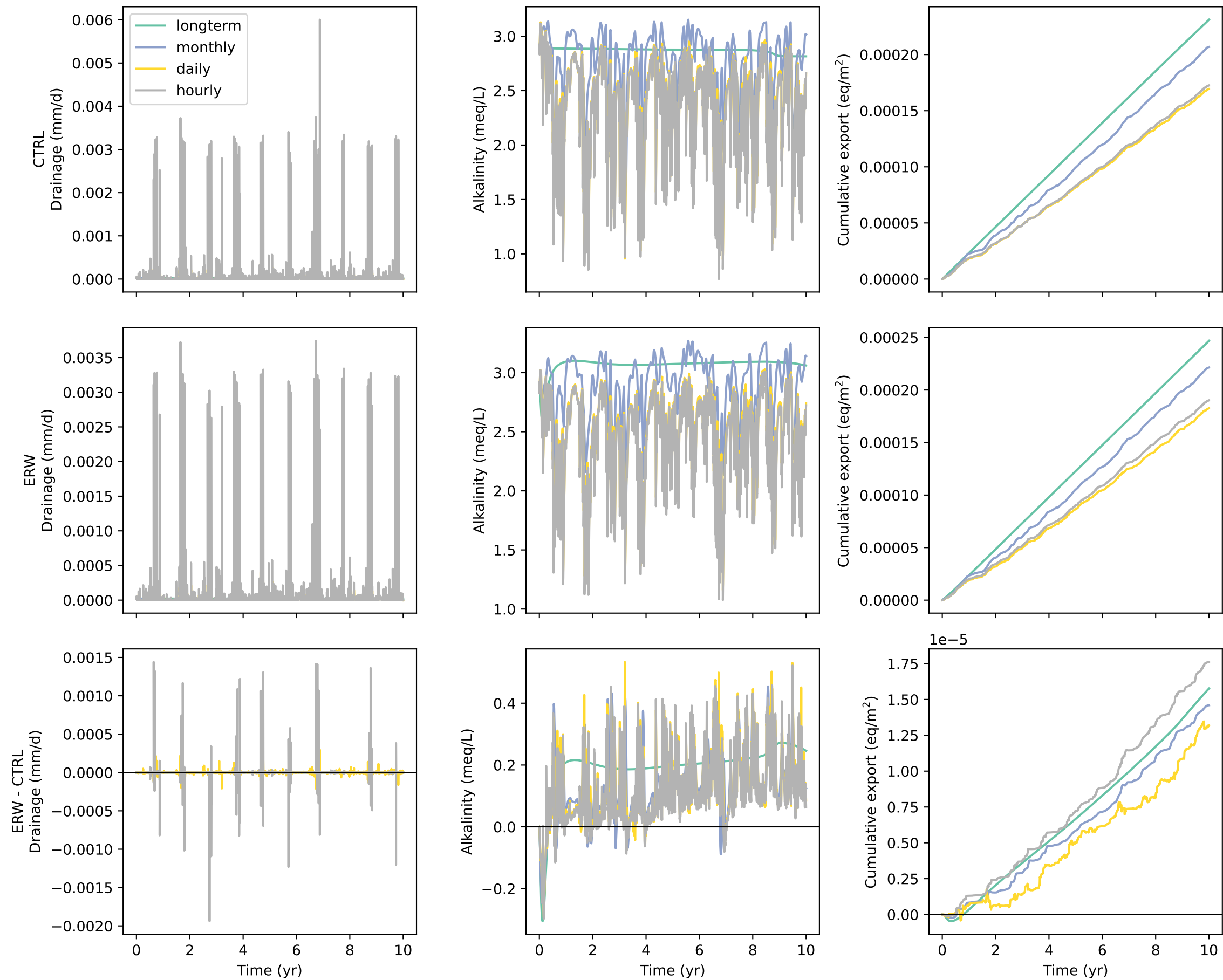
Flanagan: drainage and alkalinity export at 50 cm
