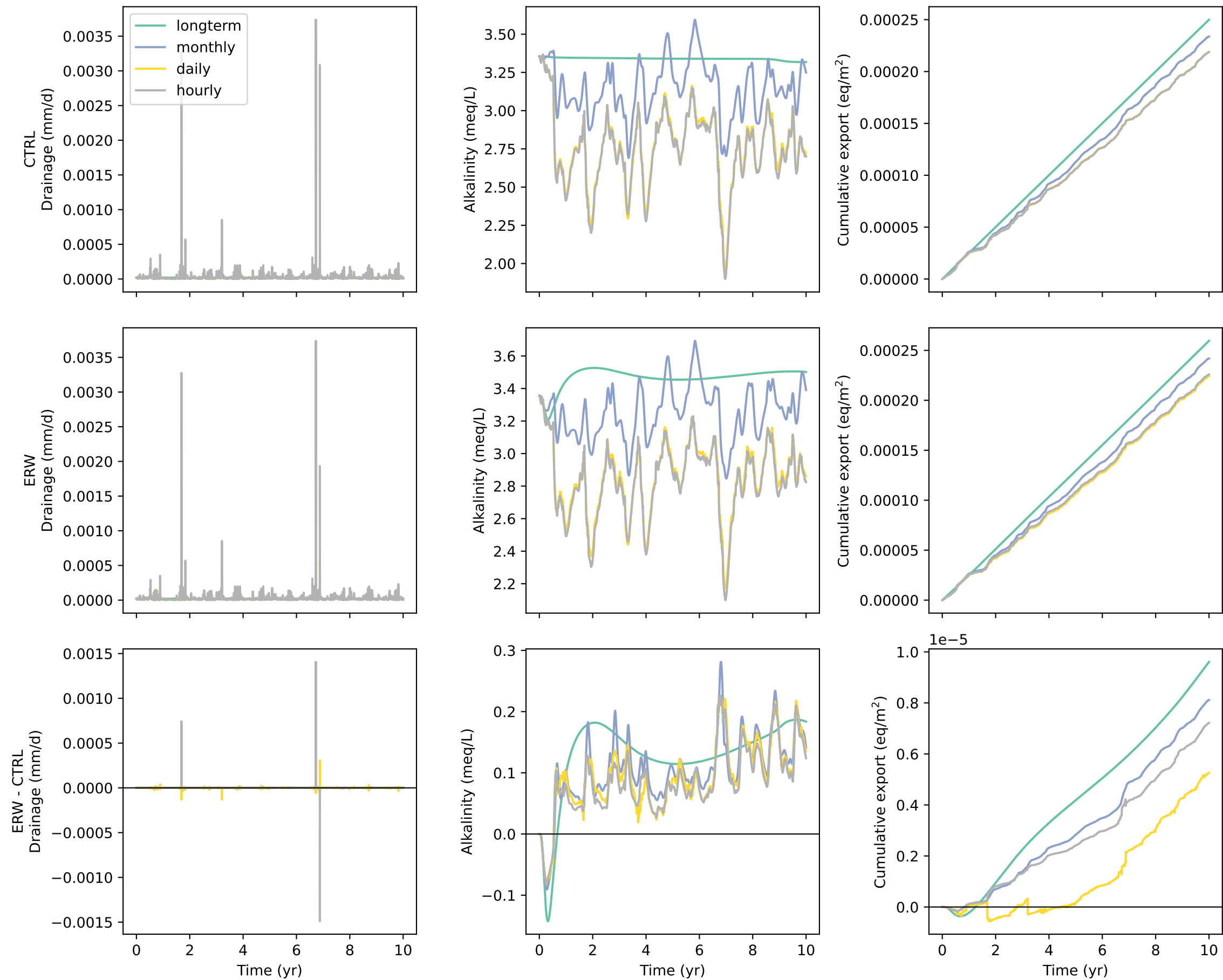
Flanagan: drainage and alkalinity export at 100 cm
