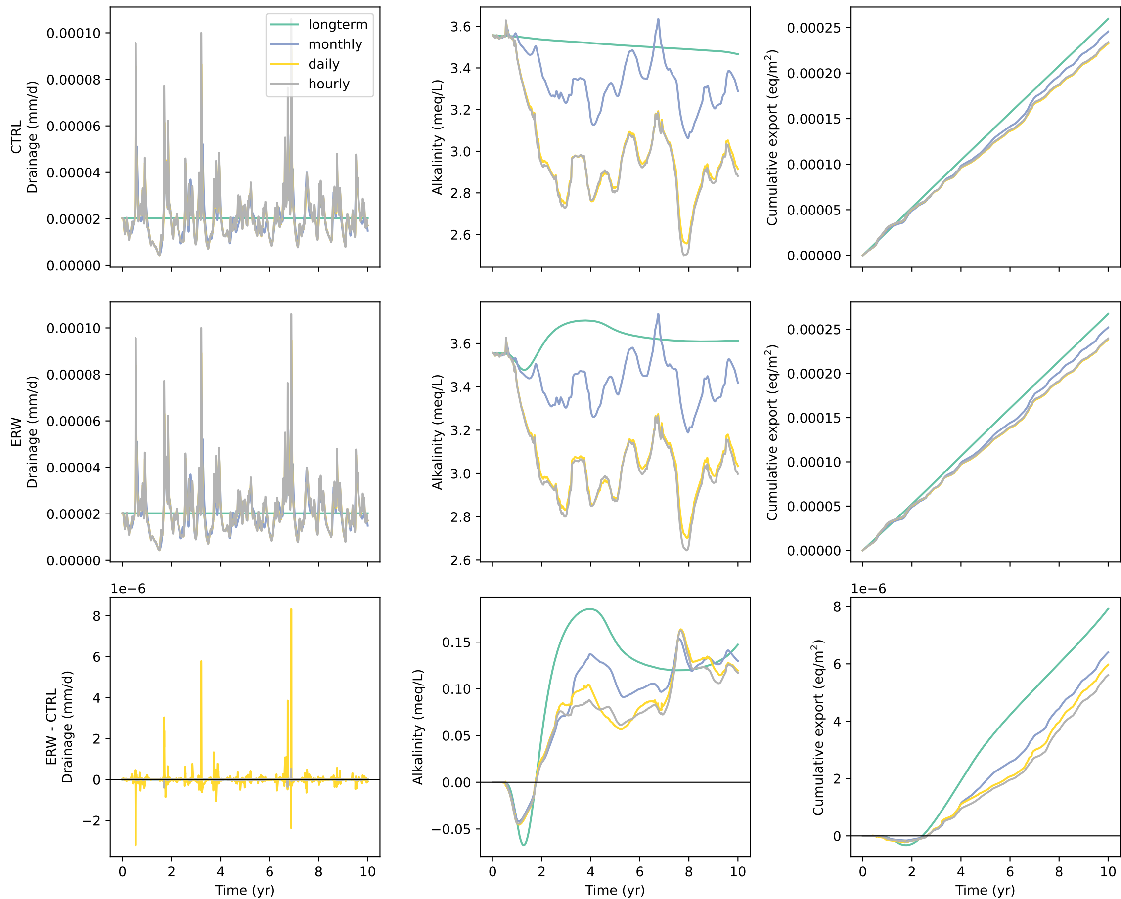
Flanagan: drainage and alkalinity export at 300 cm
