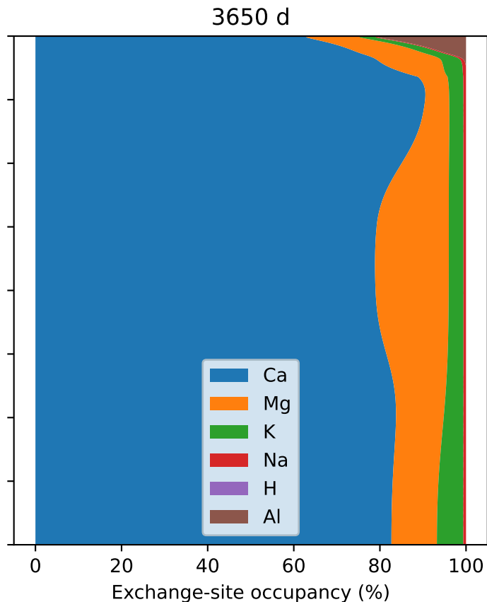
hourly (ctrl): Final exchanger composition
