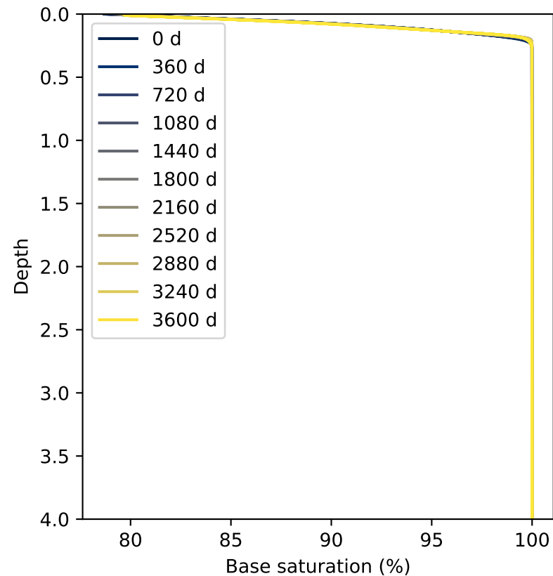
hourly (ctrl): Final exchanger composition
