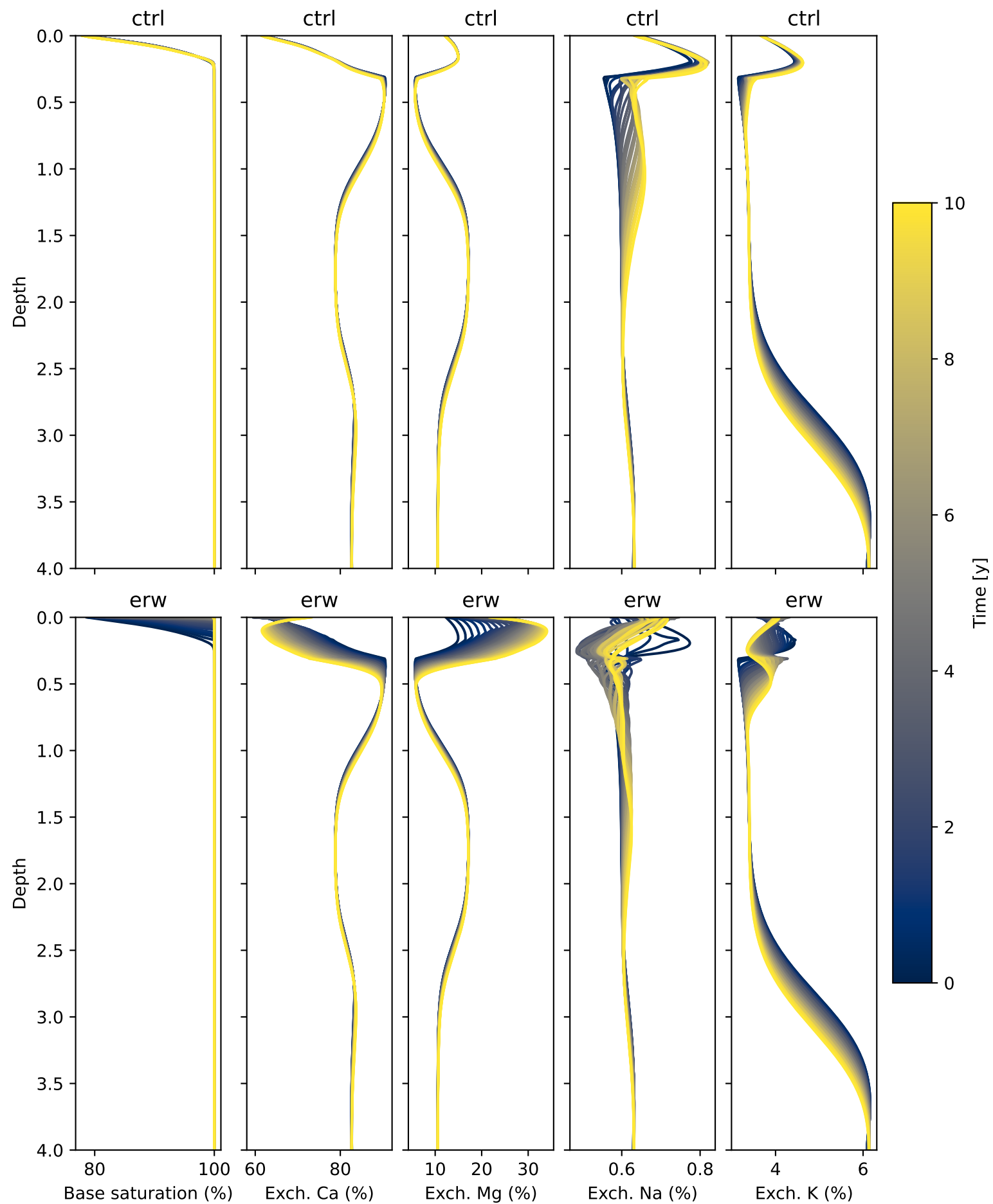
monthly: Base saturation and exchange composition
