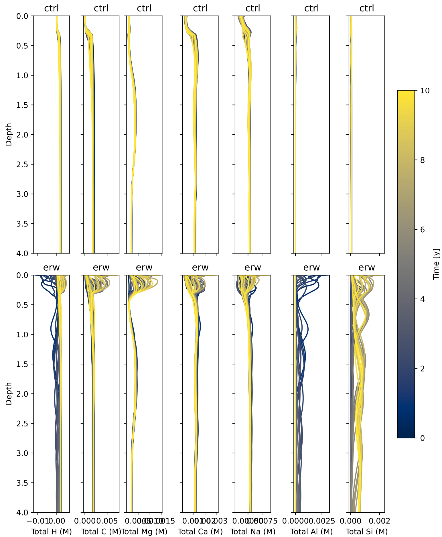
hourly: Total concentrations
