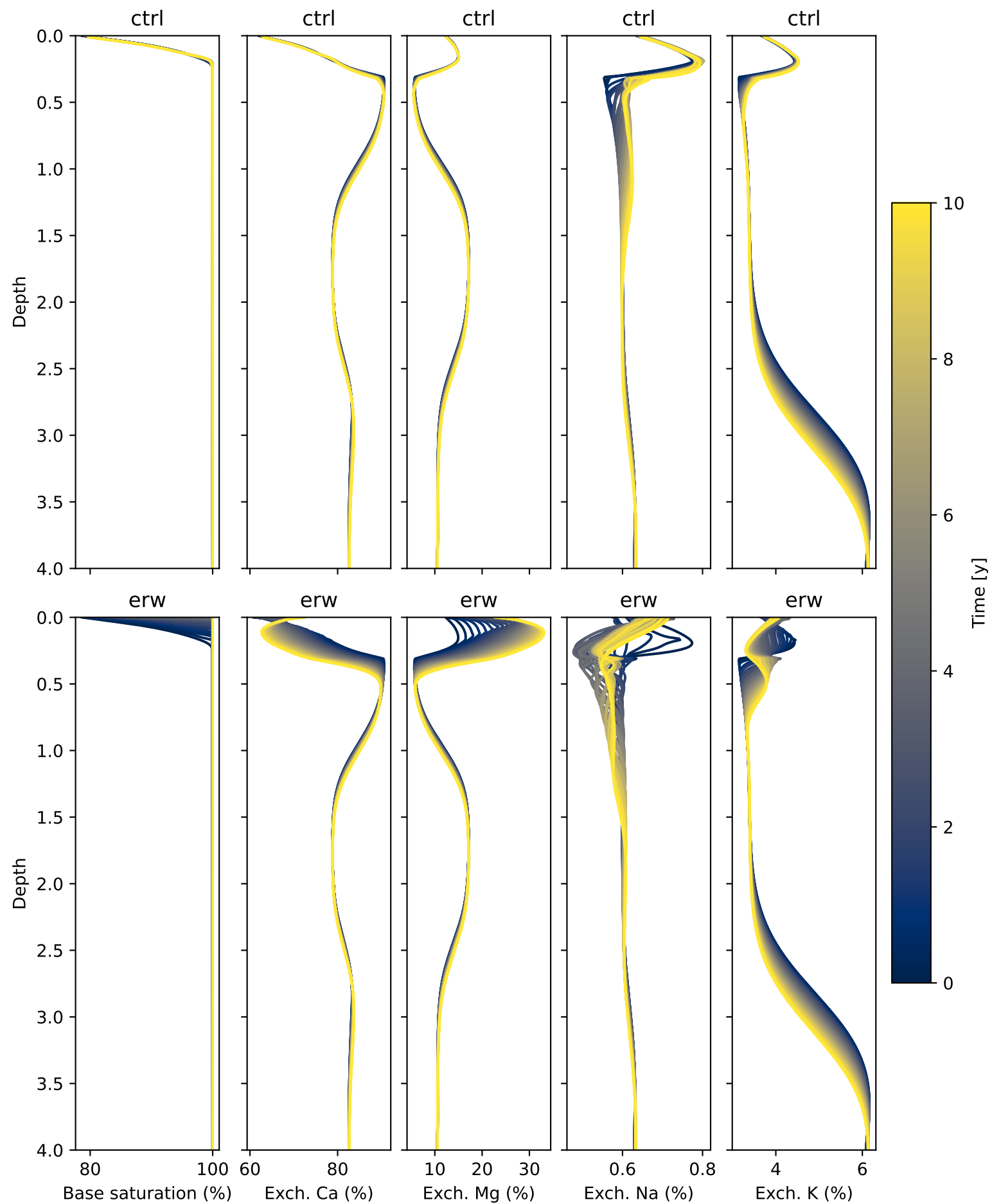
hourly: Base saturation and exchange composition
