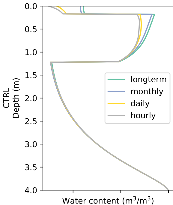
Cecil: mean water content and gas profiles
