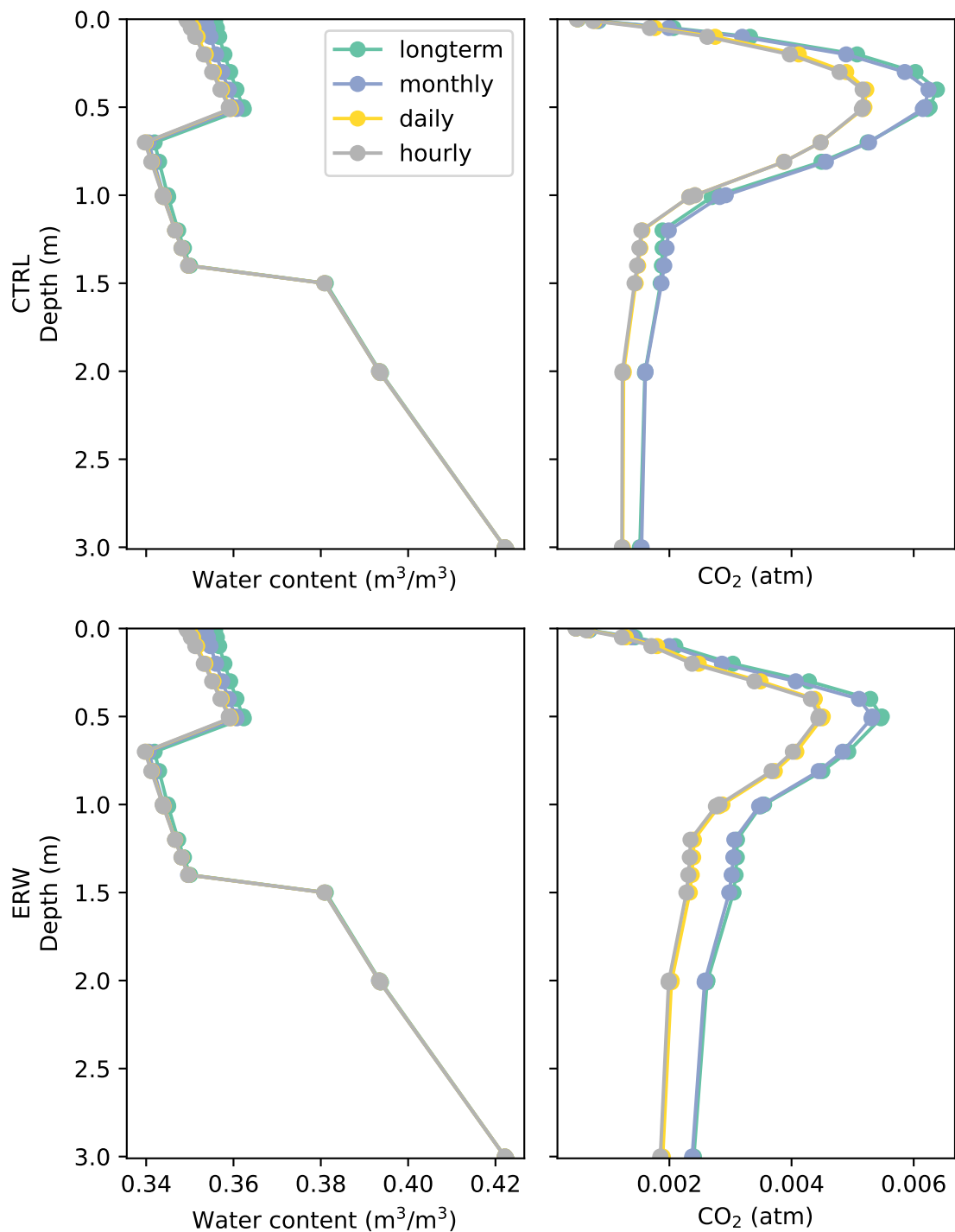
Palouse: mean water content and gas profiles, from transient output
