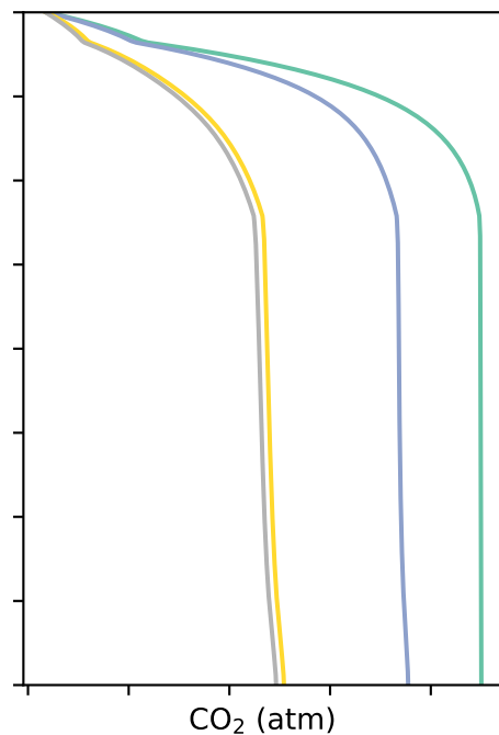
Cecil: mean water content and gas profiles
