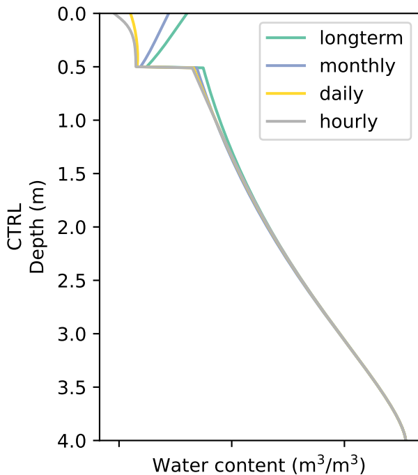
Yolo: mean water content and gas profiles
