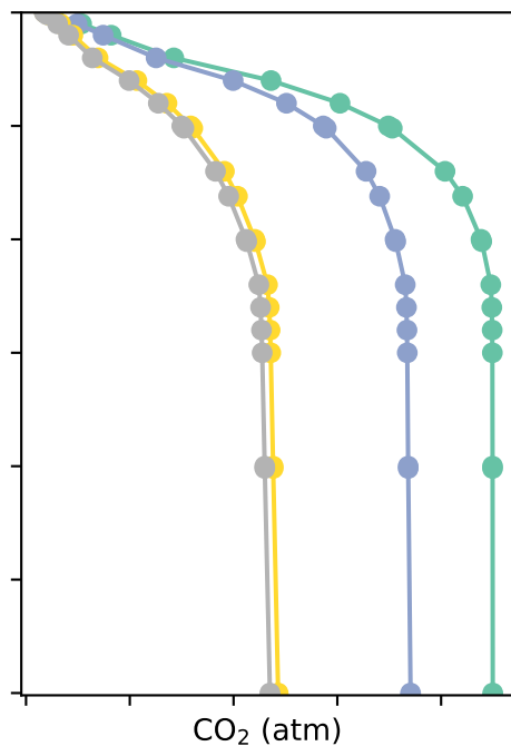
Cecil: mean water content and gas profiles, from transient output
