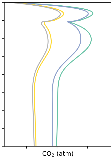
Yolo: mean water content and gas profiles
