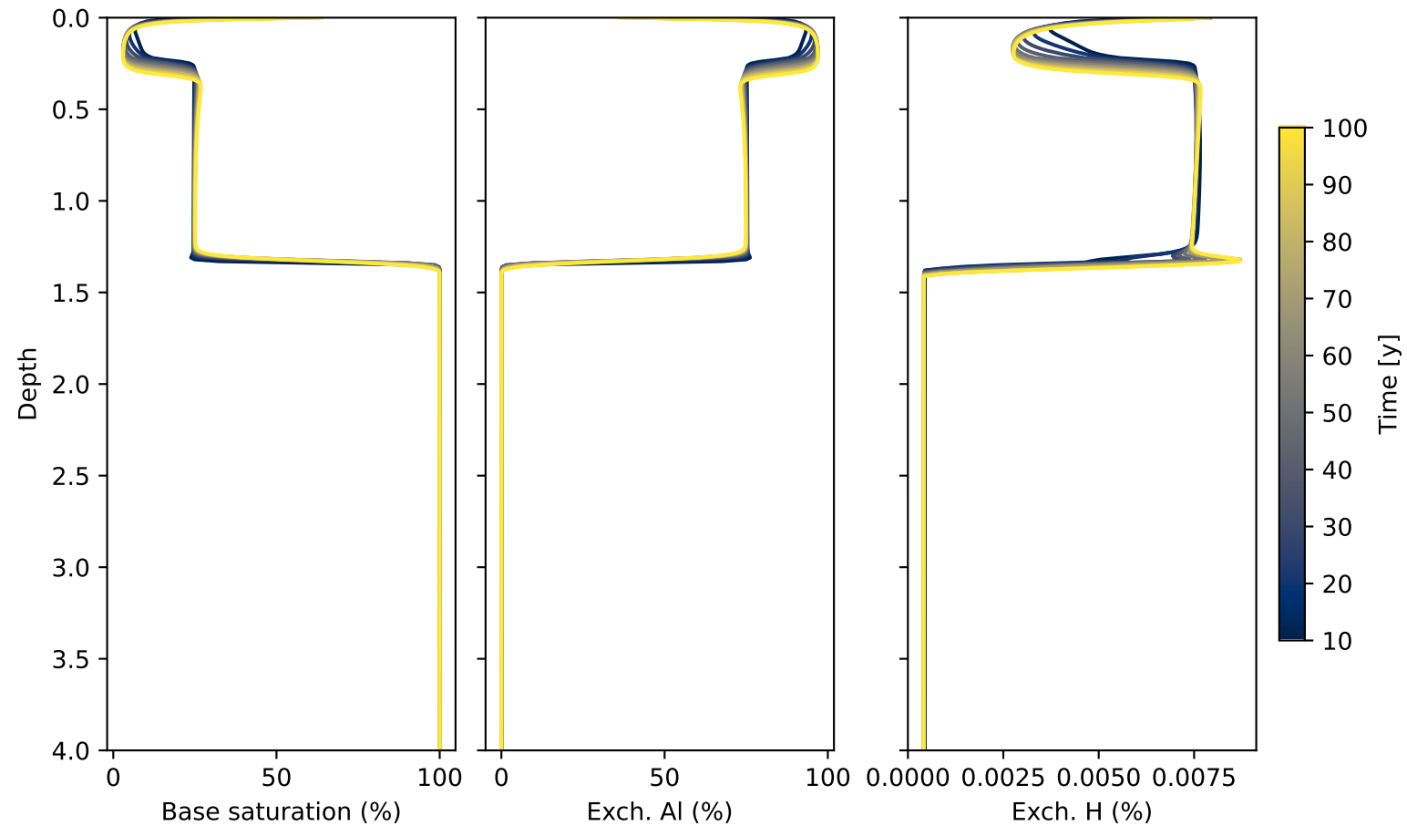
Kalamazoo: Base saturation and exchangeable acidity
