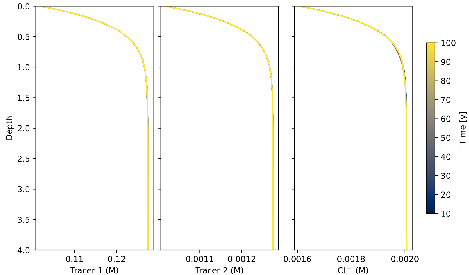
Palouse: Tracer profiles
