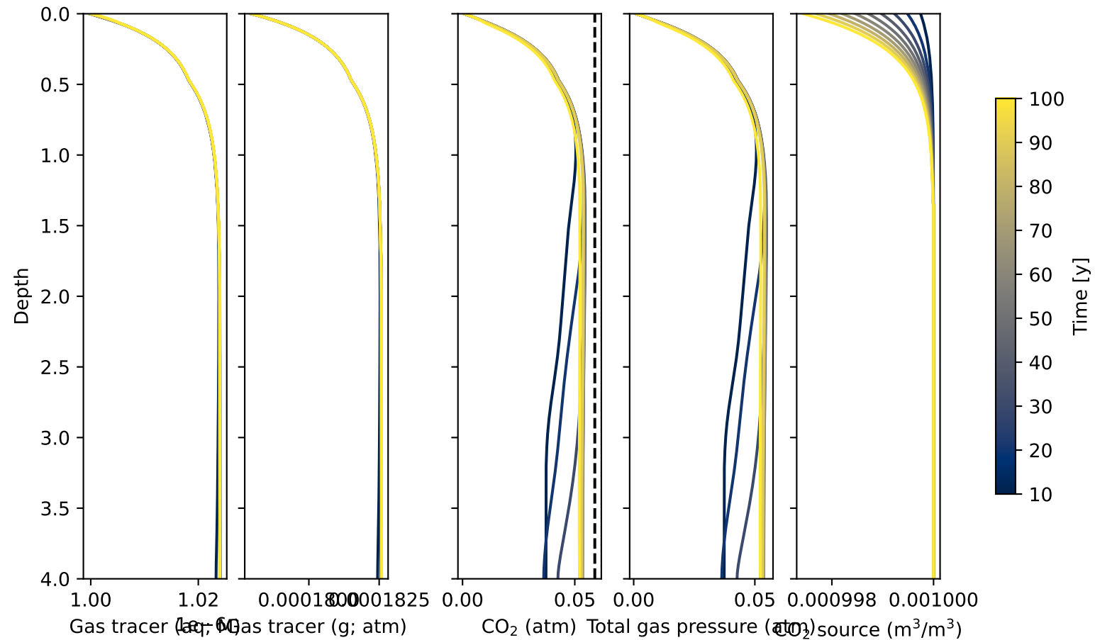
HoustonBlack: CO 2 and gas tracer
