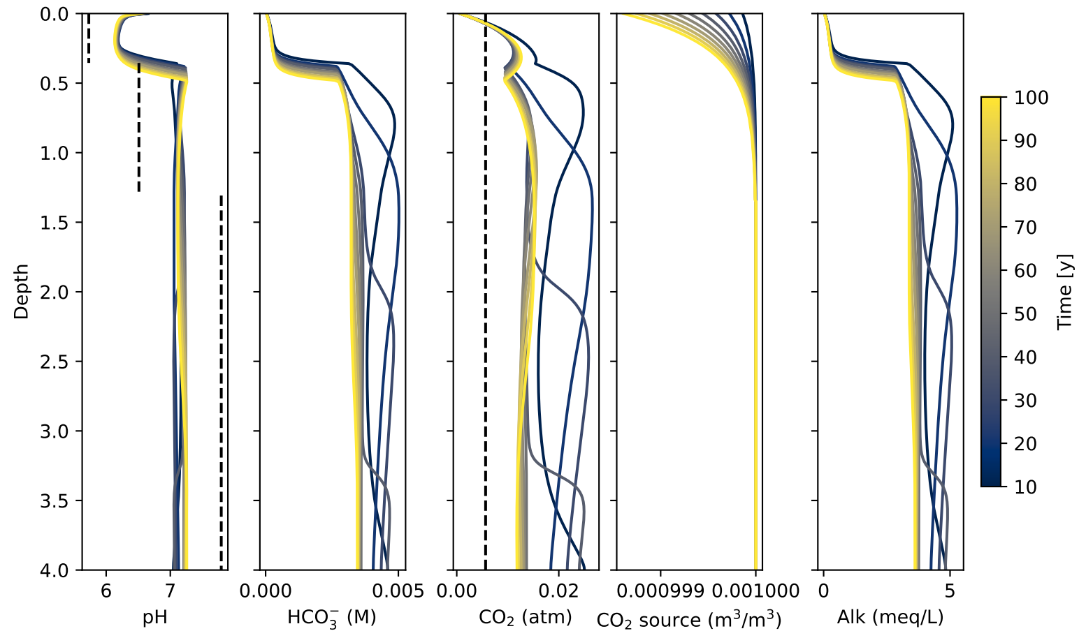
Flanagan: pH, alkalinity, and CO 2 respiration
