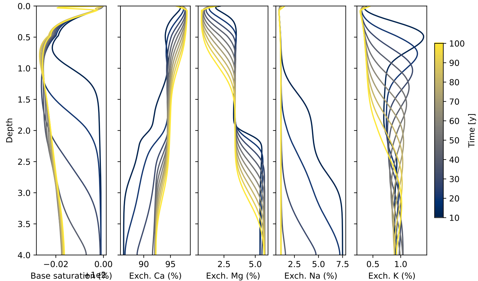
HoustonBlack: Base saturation and exchange composition
