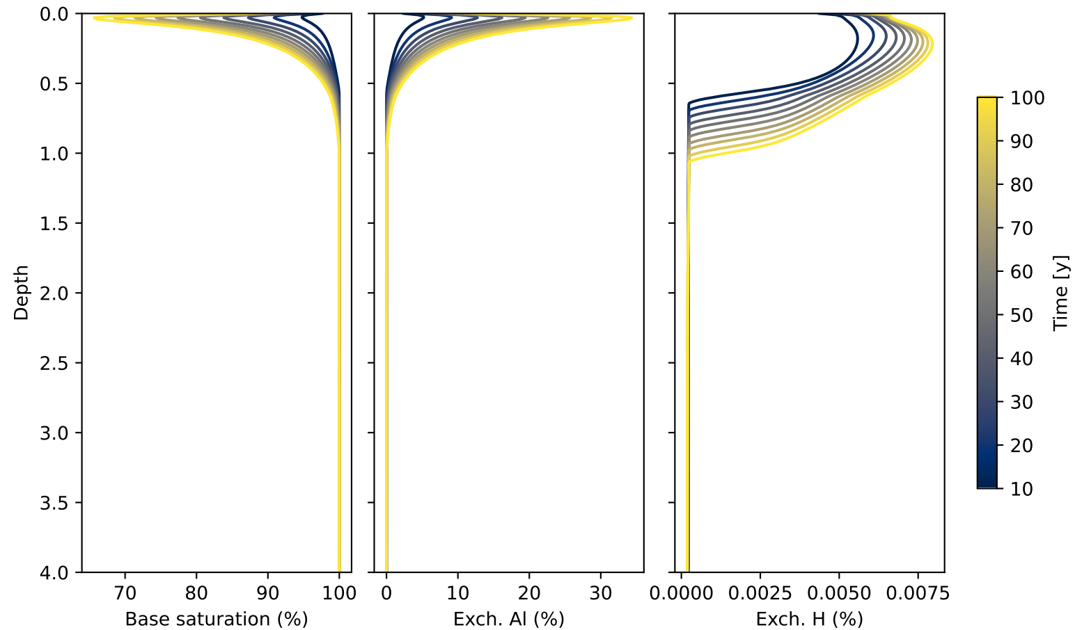
Palouse: Base saturation and exchangeable acidity
