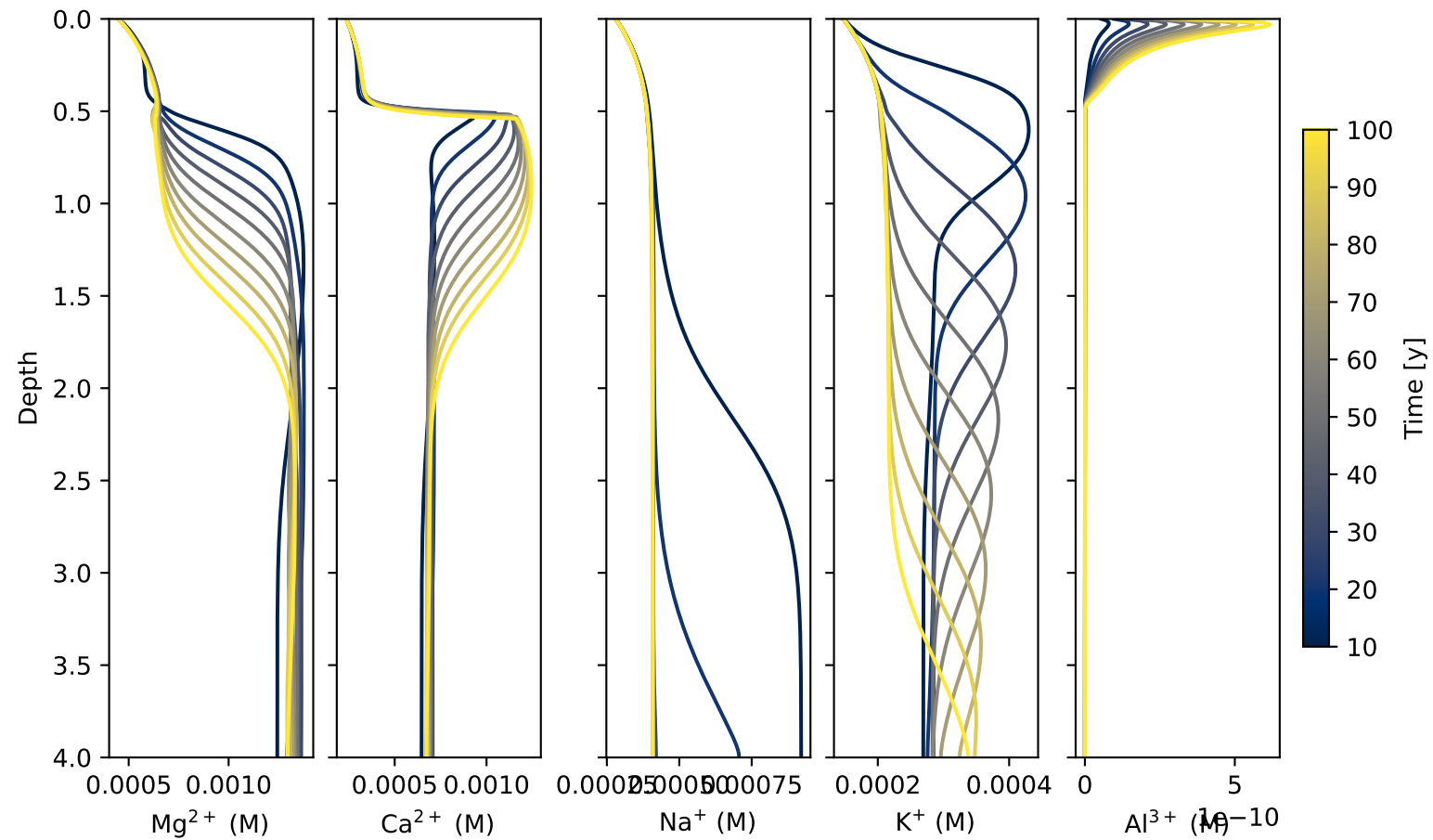
Yolo: Major cations
