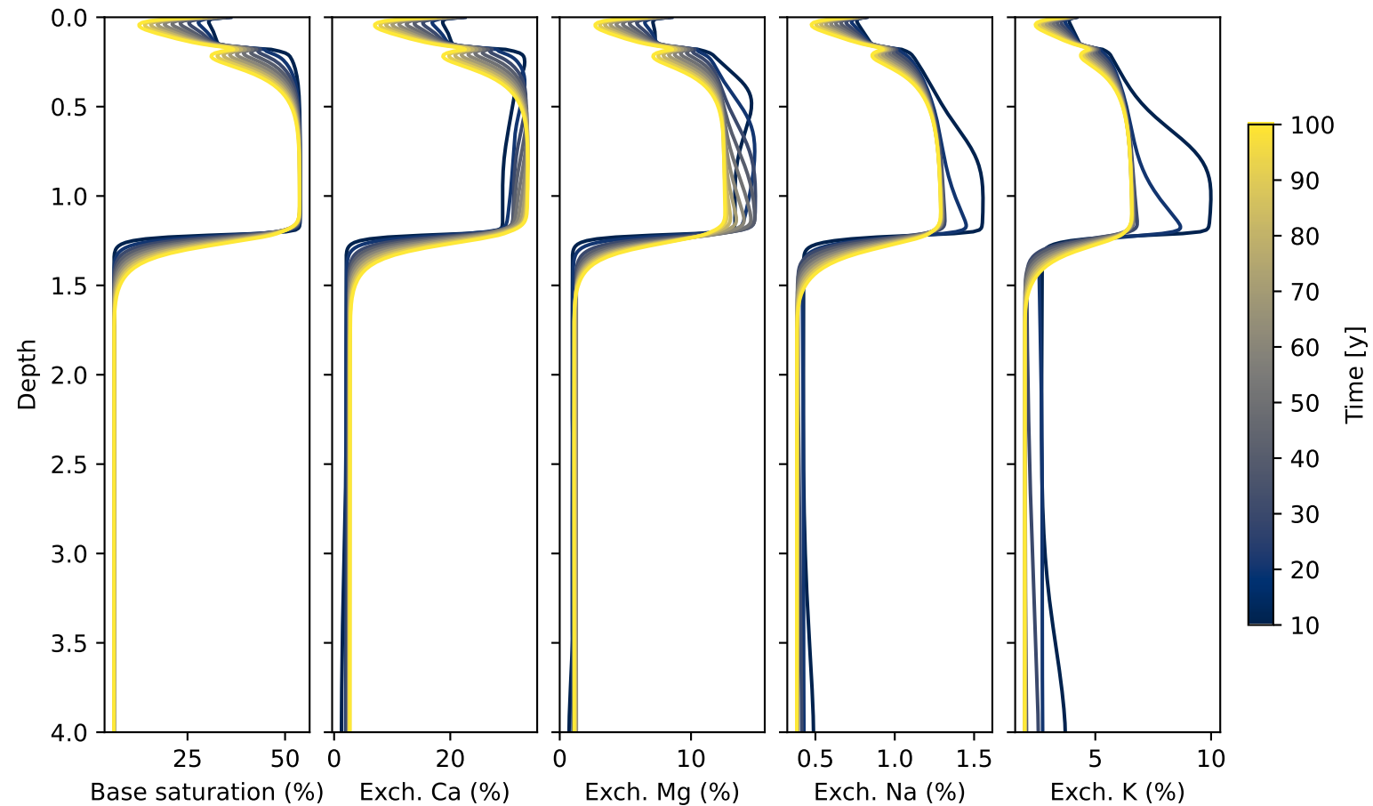
Cecil: Base saturation and exchange composition
