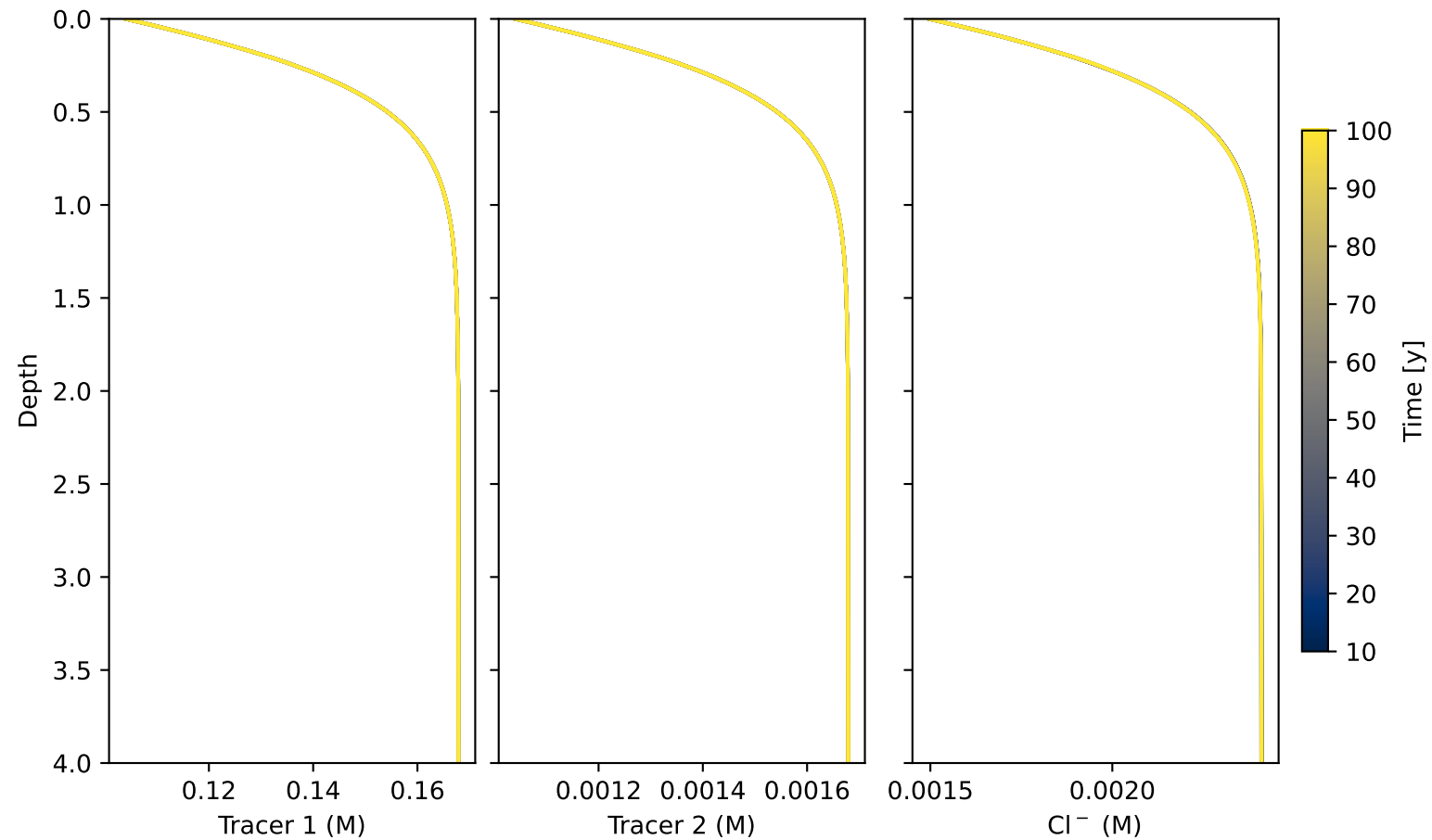
Kuma: Tracer profiles
