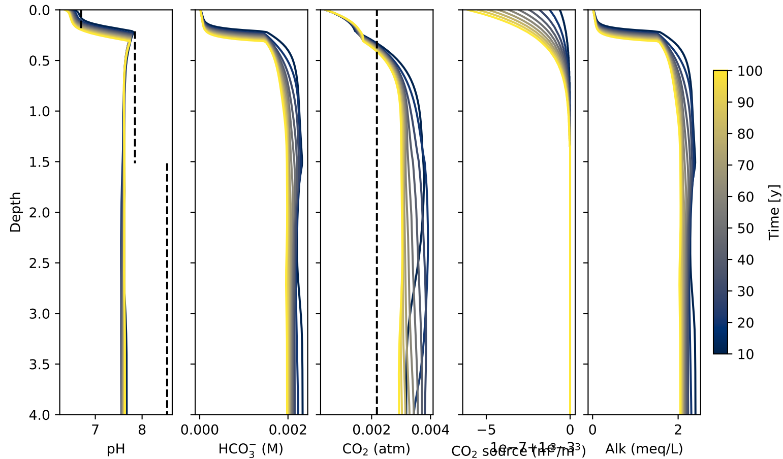
Kuma: pH, alkalinity, and CO 2 respiration
