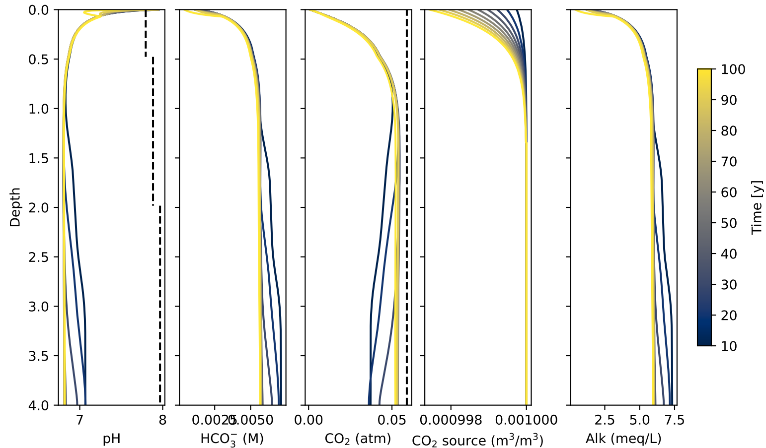
HoustonBlack: pH, alkalinity, and CO2 respiration
