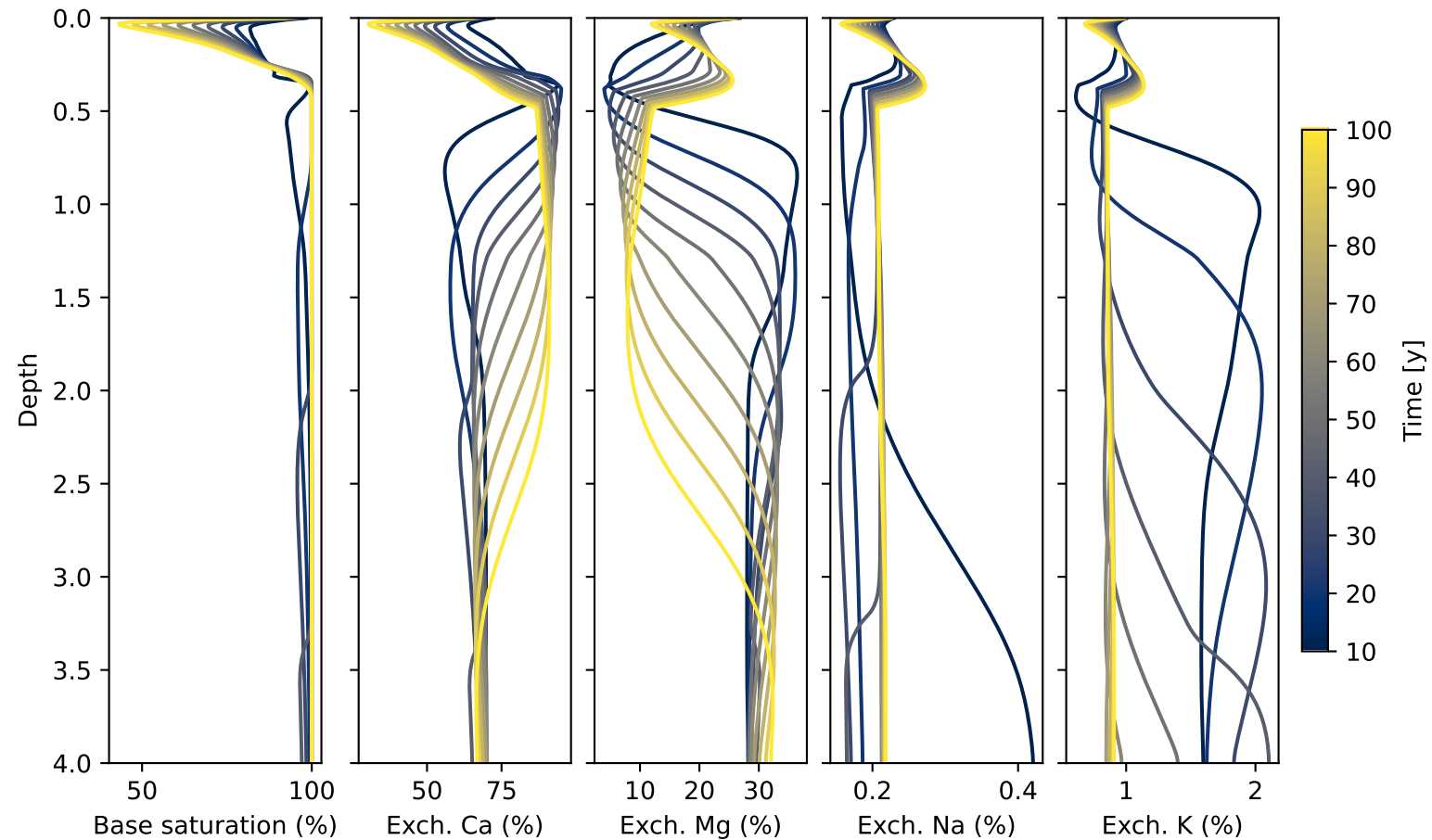
Flanagan: Base saturation and exchange composition
