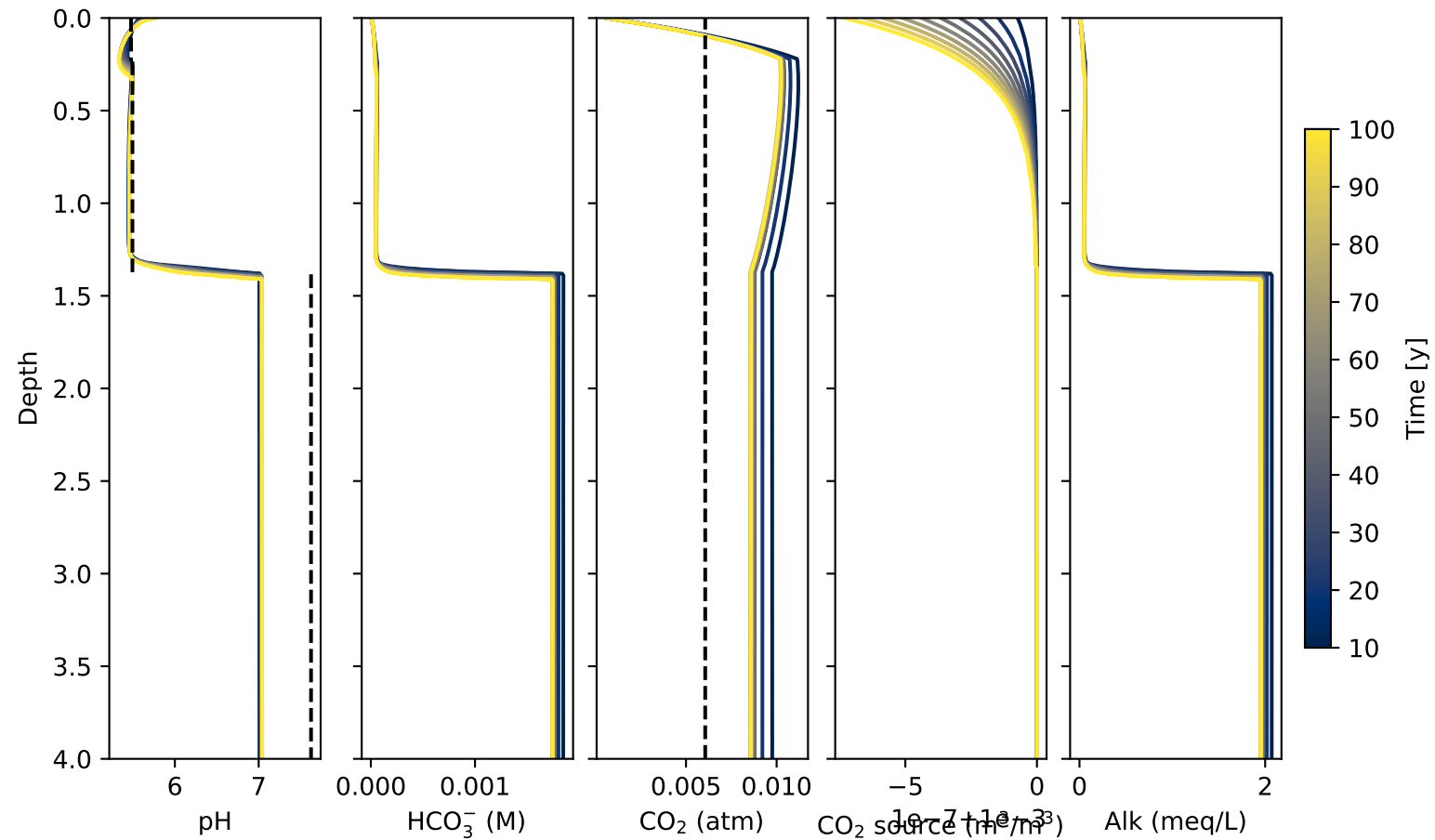
Kalamazoo: pH, alkalinity, and CO 2 respiration
