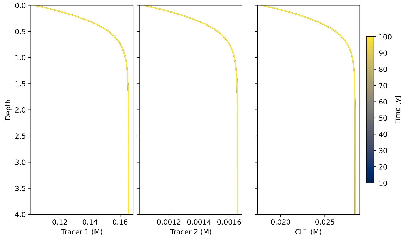
Kalamazoo: Tracer profiles
