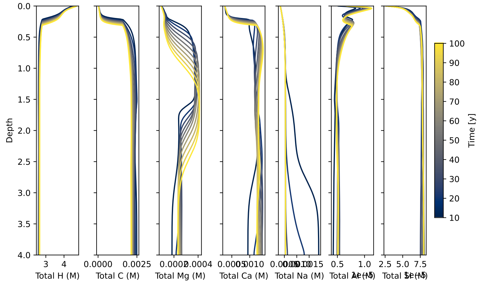
Kuma: Total concentrations
