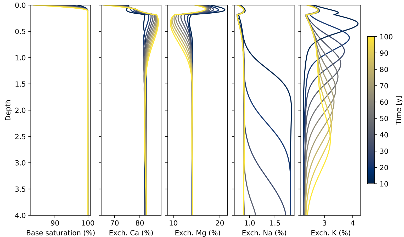
Pullman: Base saturation and exchange composition
