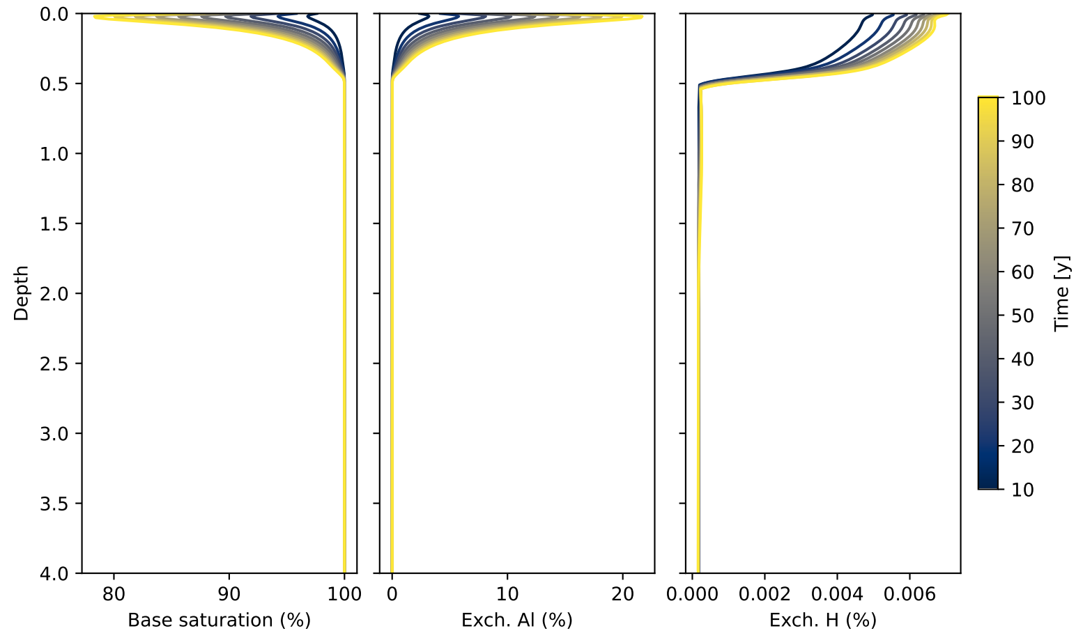
Yolo: Base saturation and exchangeable acidity
