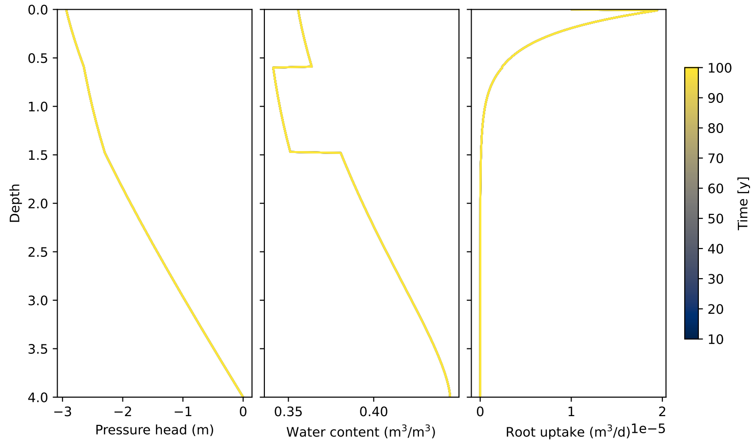
Palouse: Water content and root uptake
