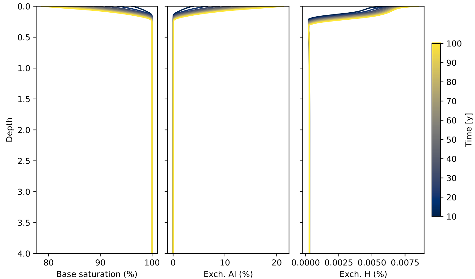
Kuma: Base saturation and exchangeable acidity
