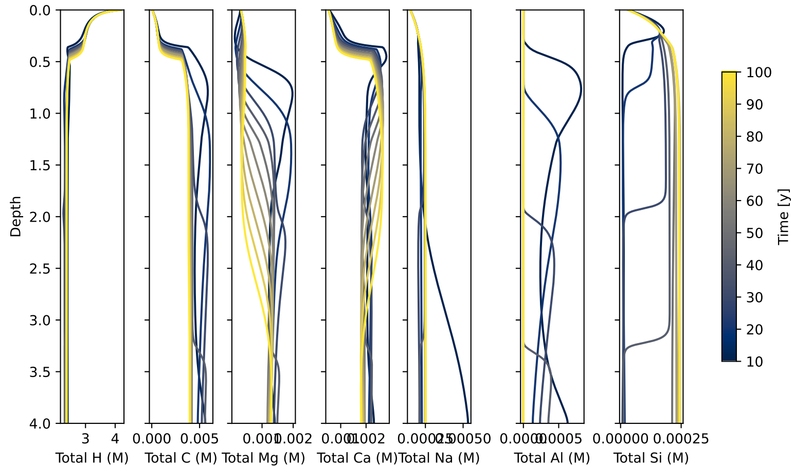
Flanagan: Total concentrations
