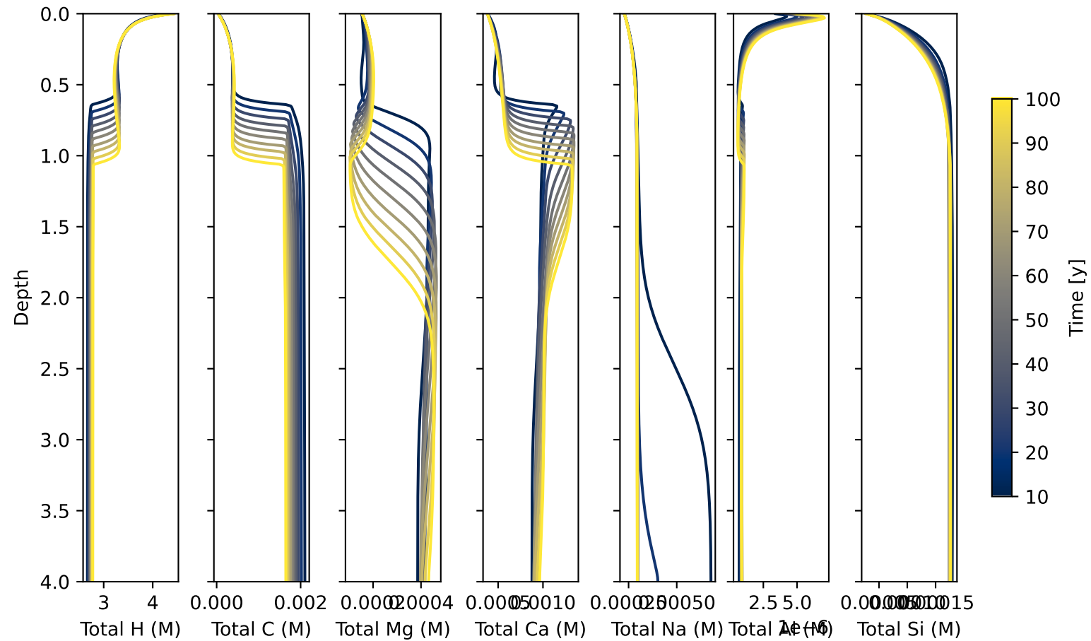
Palouse: Total concentrations
