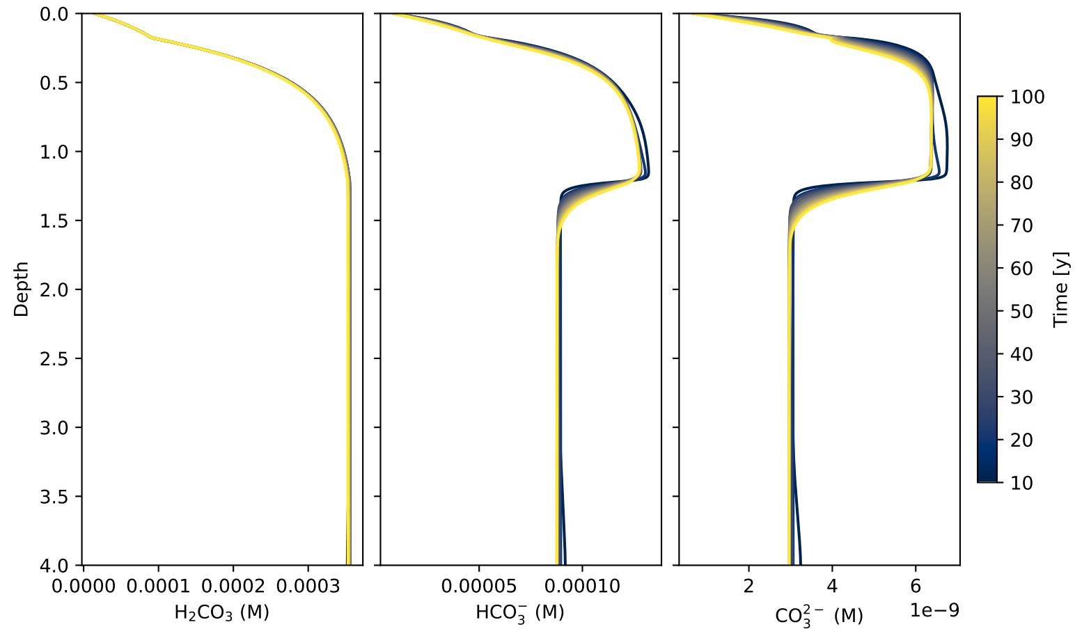
Cecil: Carbonate speciation
