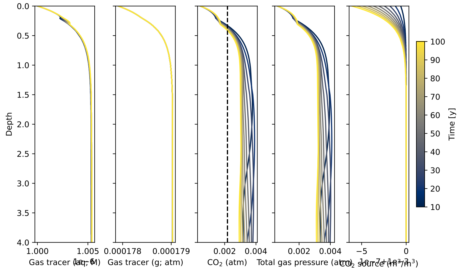
Kuma: CO 2 and gas tracer
