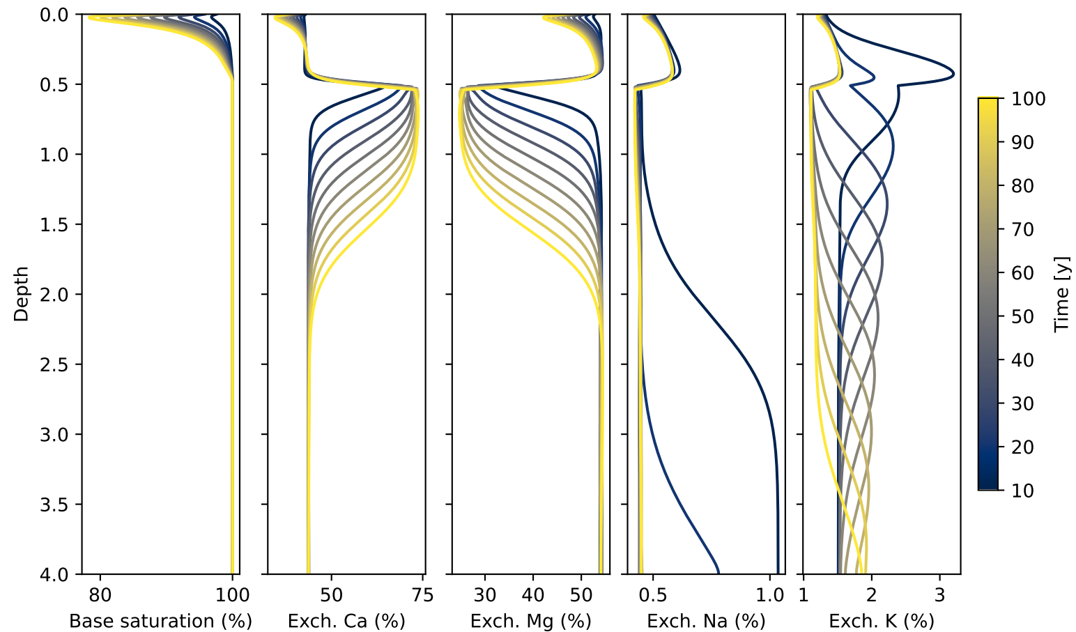
Yolo: Base saturation and exchange composition
