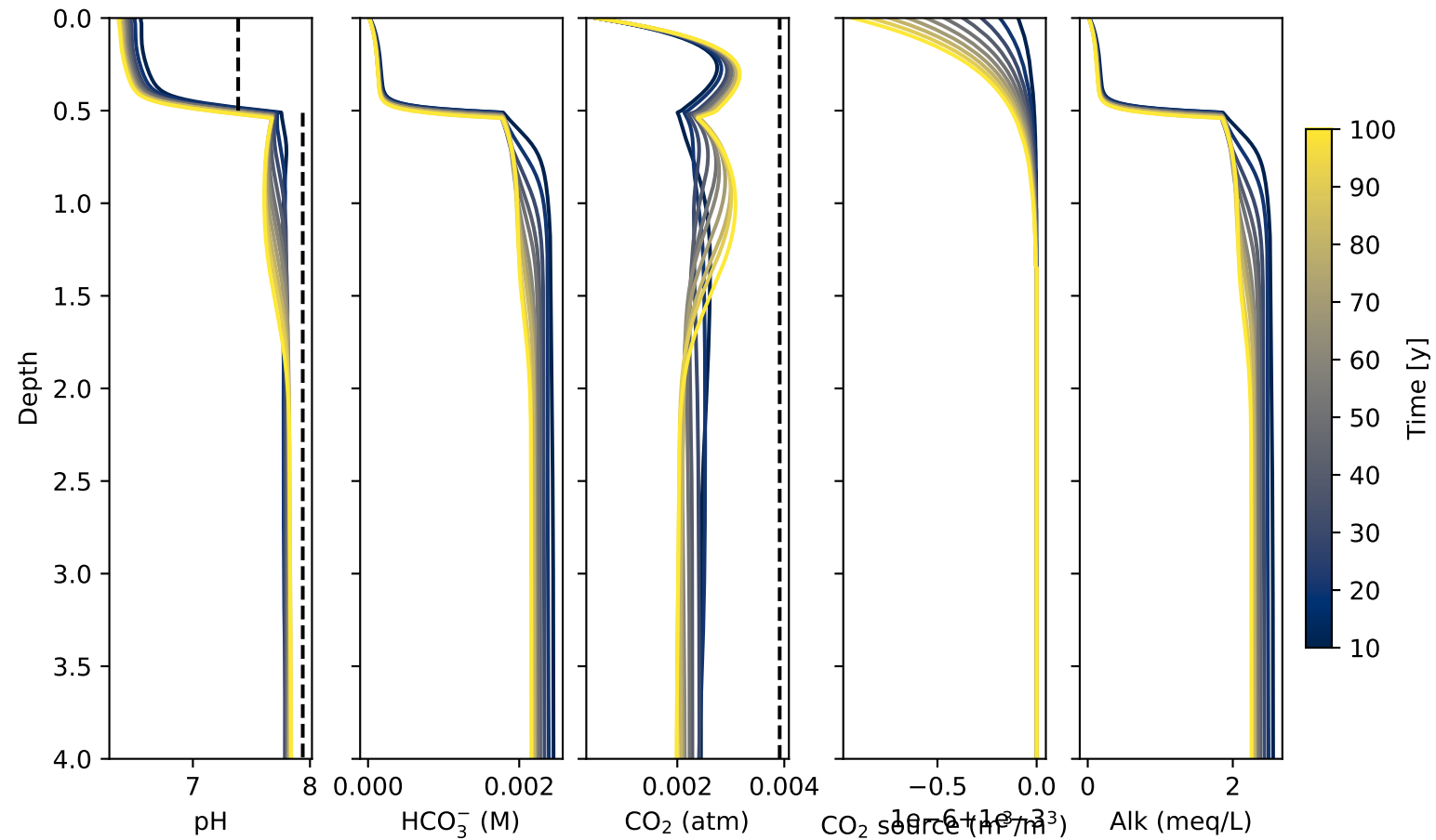
Yolo: pH, alkalinity, and CO 2 respiration
