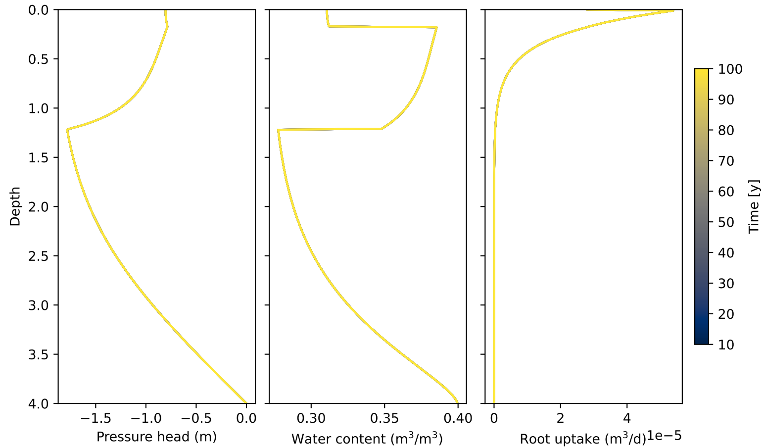
Cecil: Water content and root uptake
