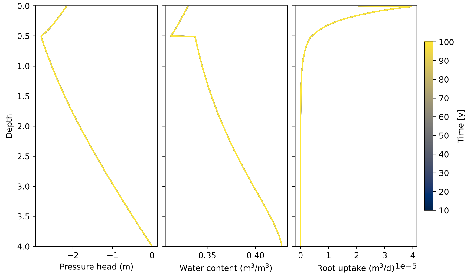
Yolo: Water content and root uptake
