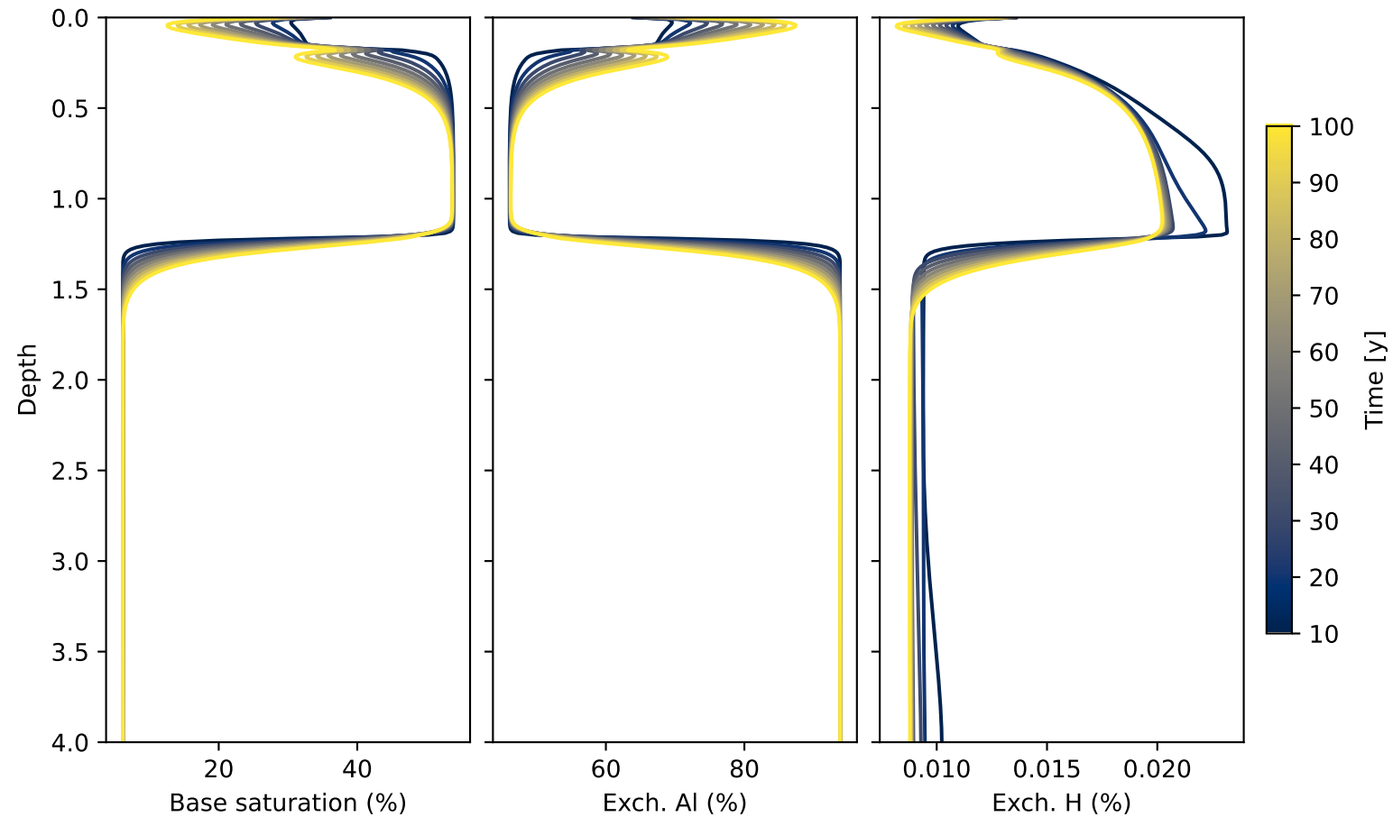
Cecil: Base saturation and exchangeable acidity
