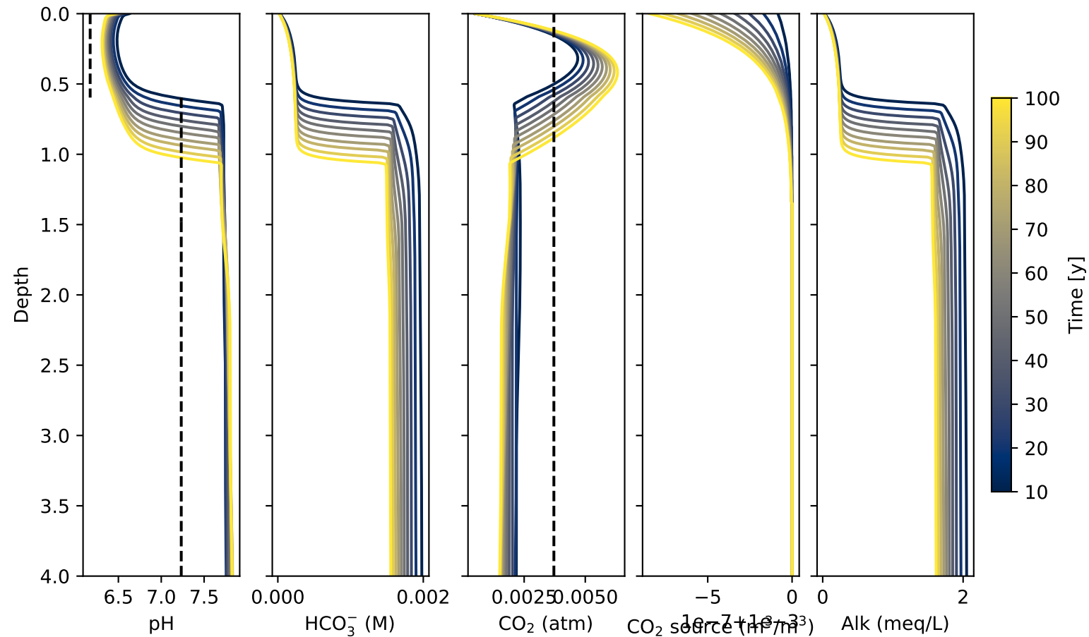
Palouse: pH, alkalinity, and CO2 respiration
