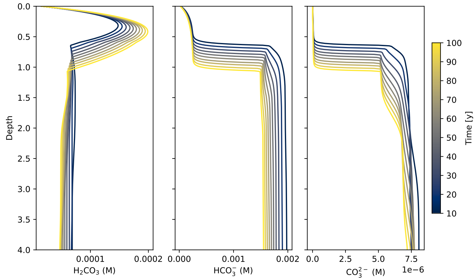
Palouse: Carbonate speciation
