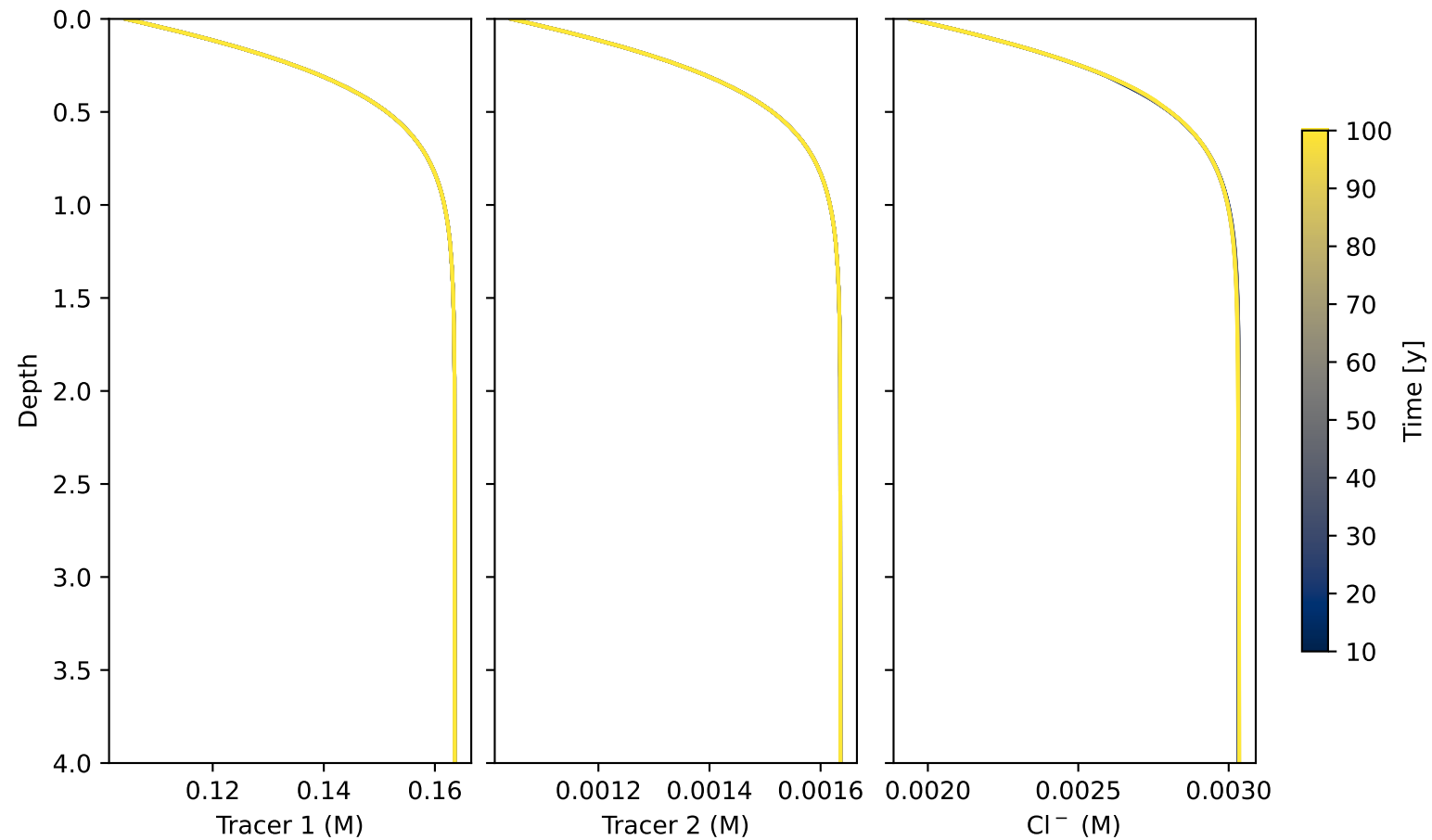
Flanagan: Tracer profiles
