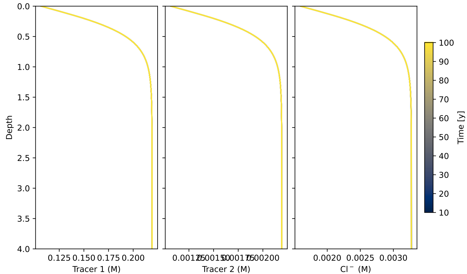
Pullman: Tracer profiles
