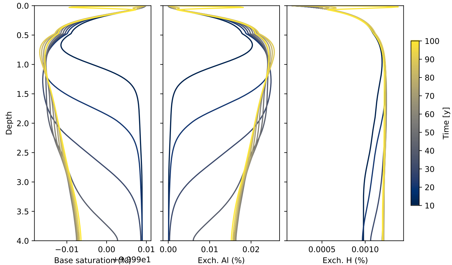
HoustonBlack: Base saturation and exchangeable acidity
