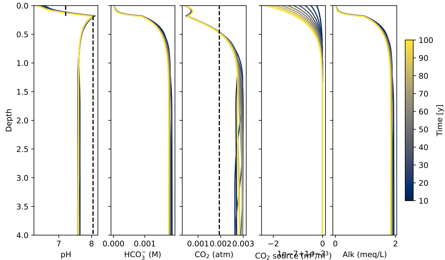
Pullman: pH, alkalinity, and CO2 respiration
