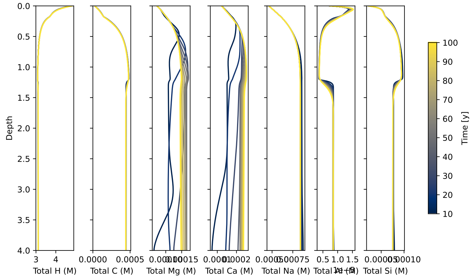
Cecil: Total concentrations
