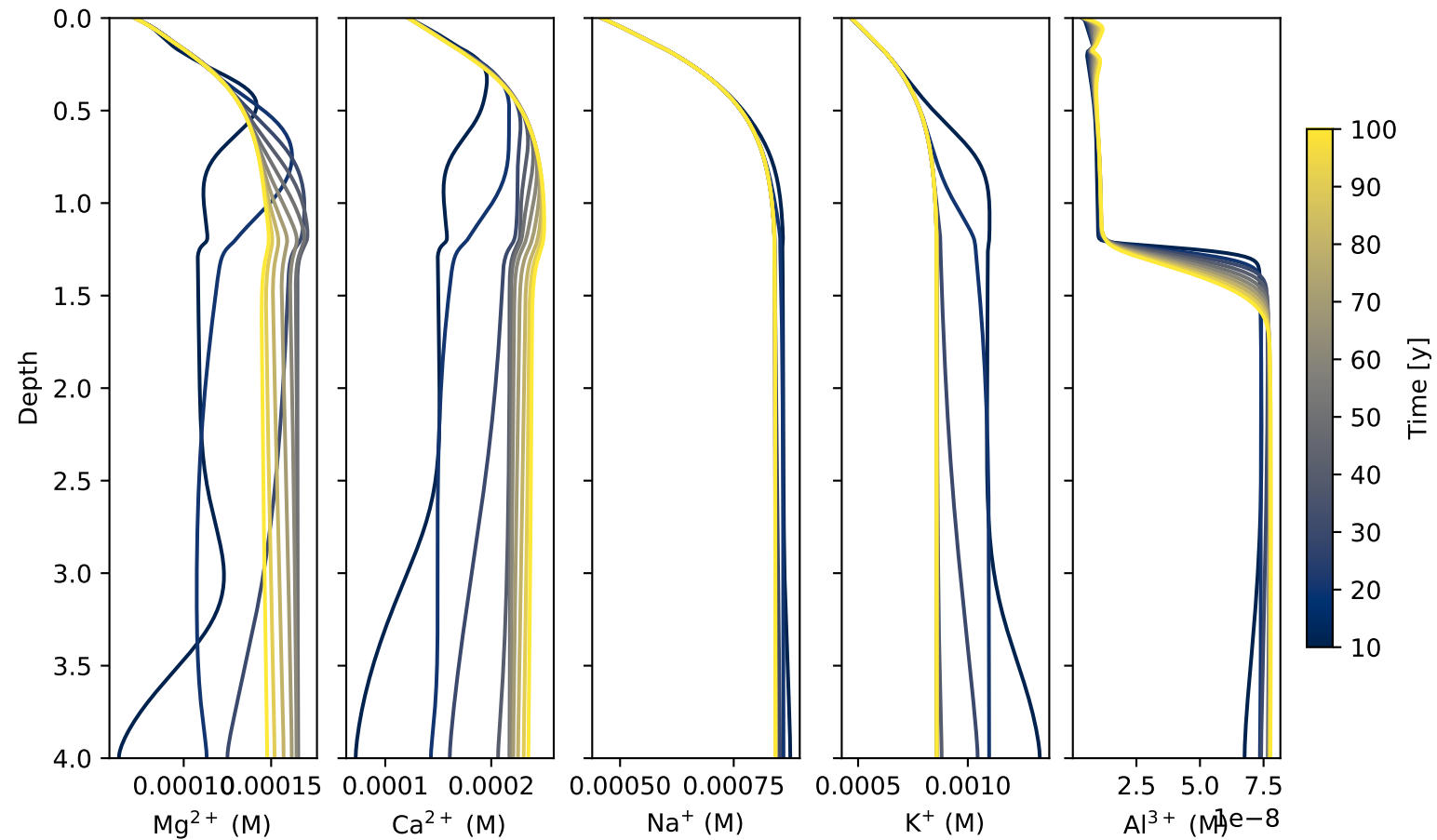
Cecil: Major cations
