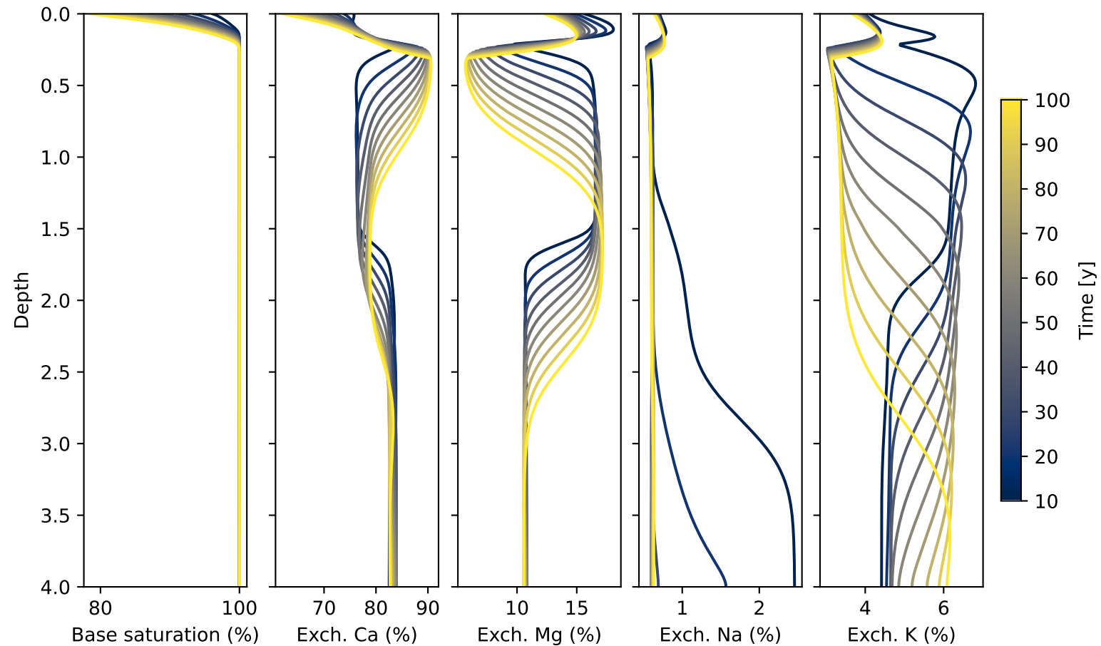
Kuma: Base saturation and exchange composition
