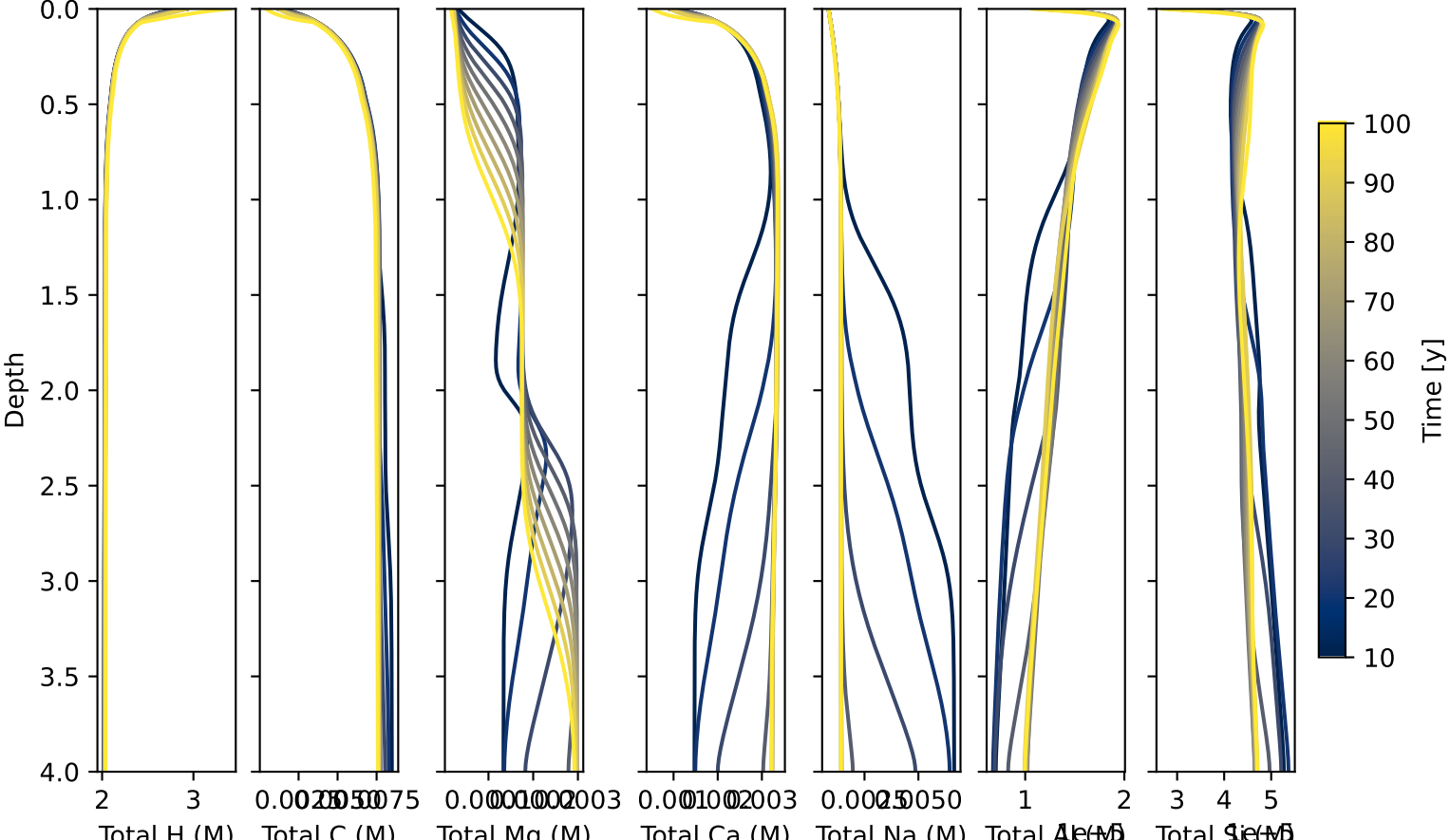
HoustonBlack: Total concentrations
