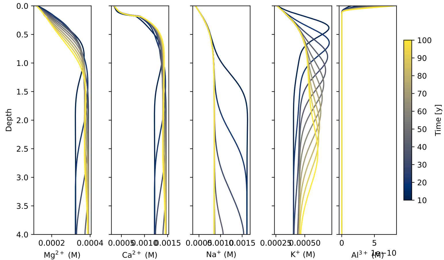
Pullman: Major cations
