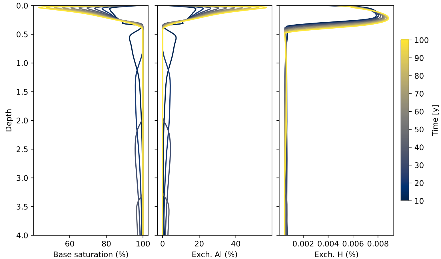
Flanagan: Base saturation and exchangeable acidity
