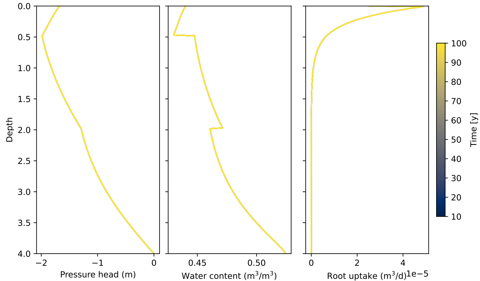
HoustonBlack: Water content and root uptake
