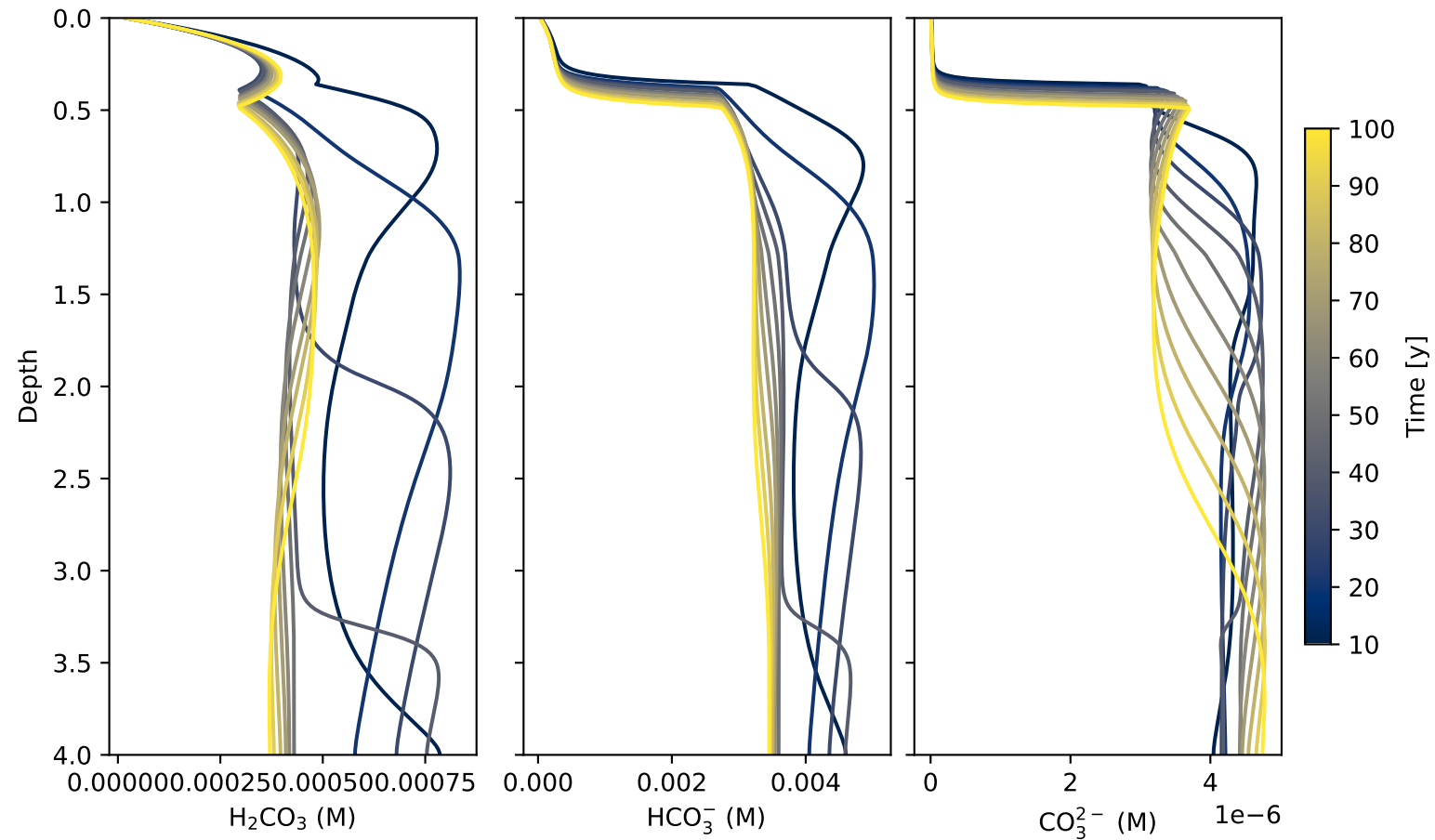
Flanagan: Carbonate speciation
