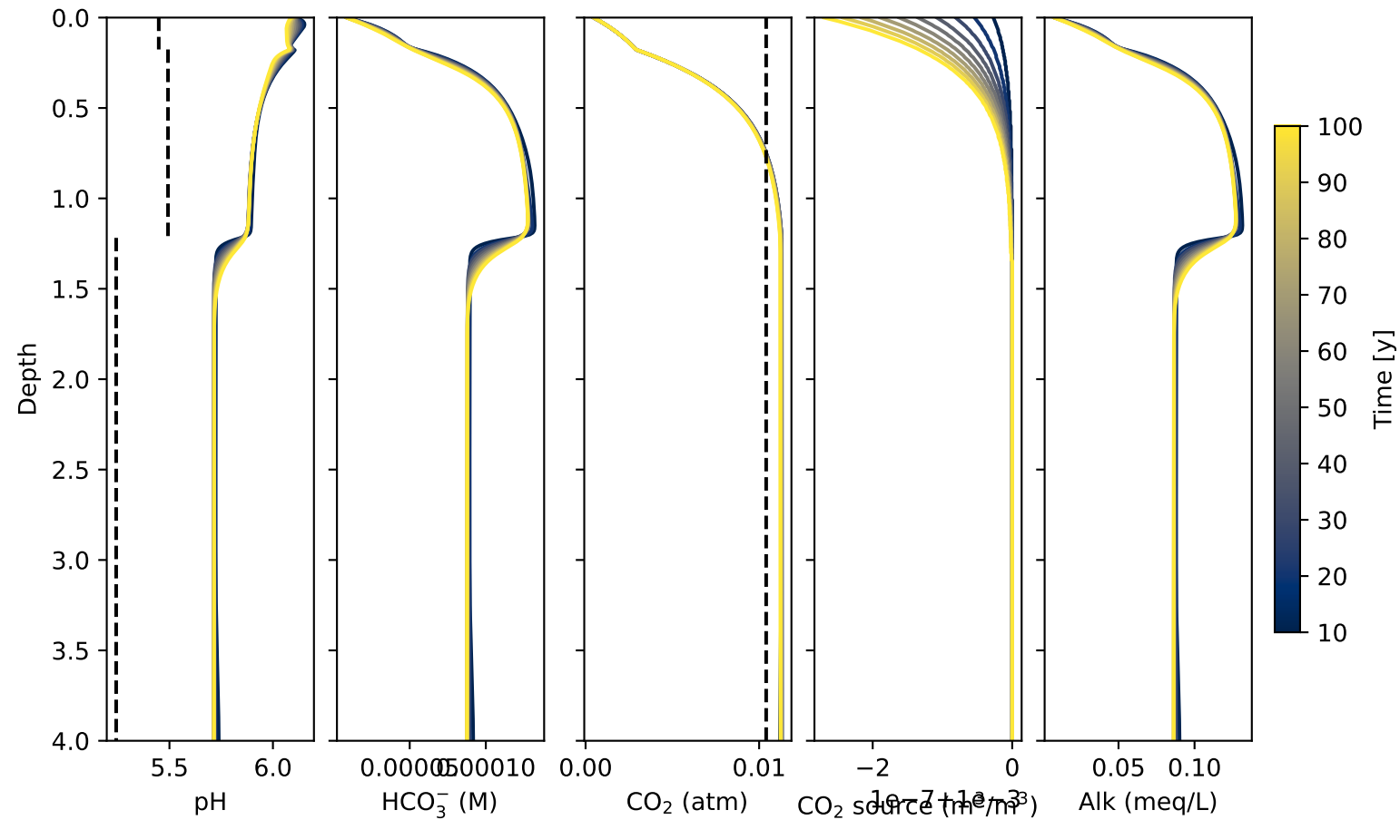
Cecil: pH, alkalinity, and CO 2 respiration
