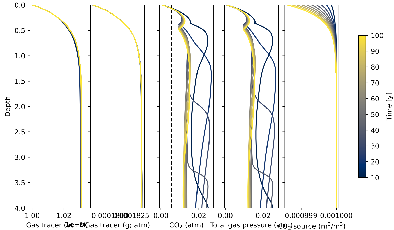
Flanagan: CO2 and gas tracer
