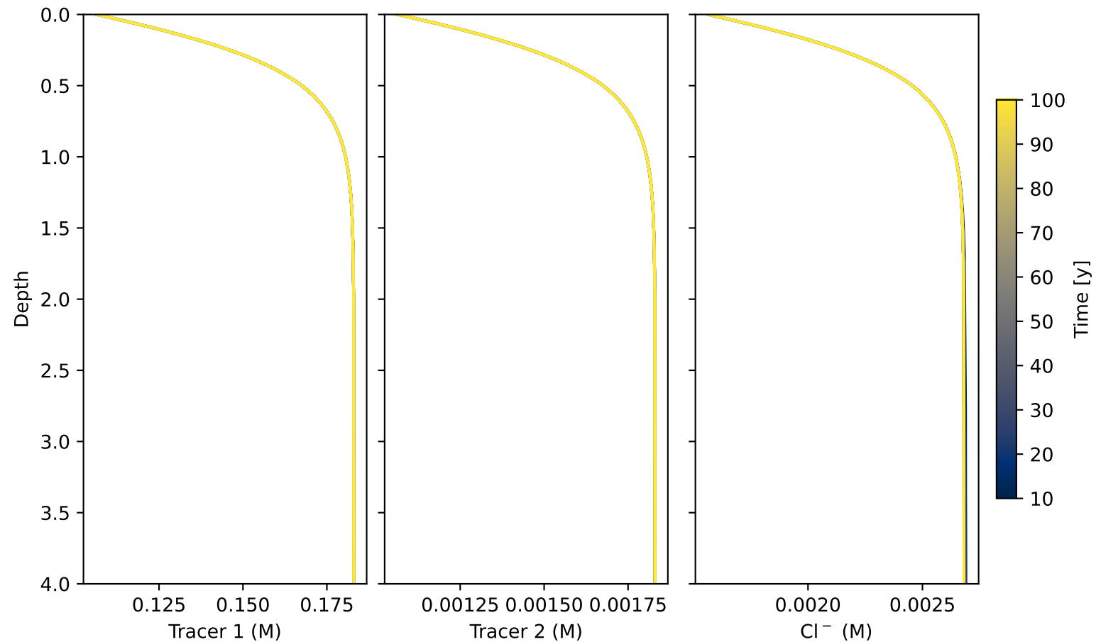
HoustonBlack: Tracer profiles
