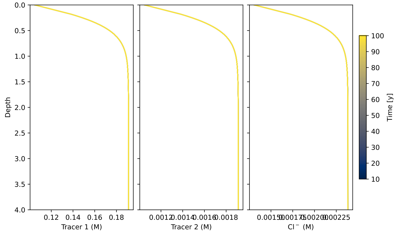
Cecil: Tracer profiles
