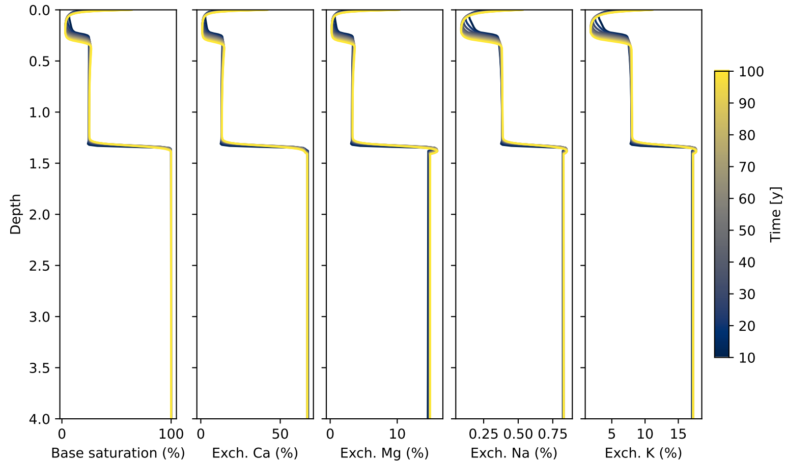
Kalamazoo: Base saturation and exchange composition
