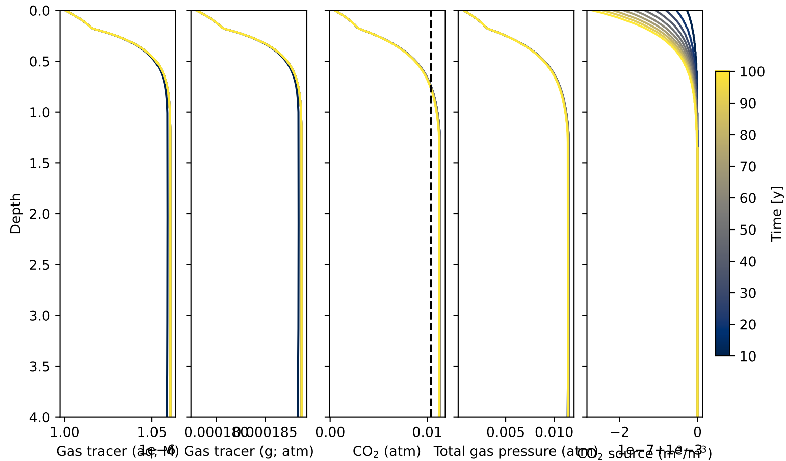
Cecil: CO 2 and gas tracer
