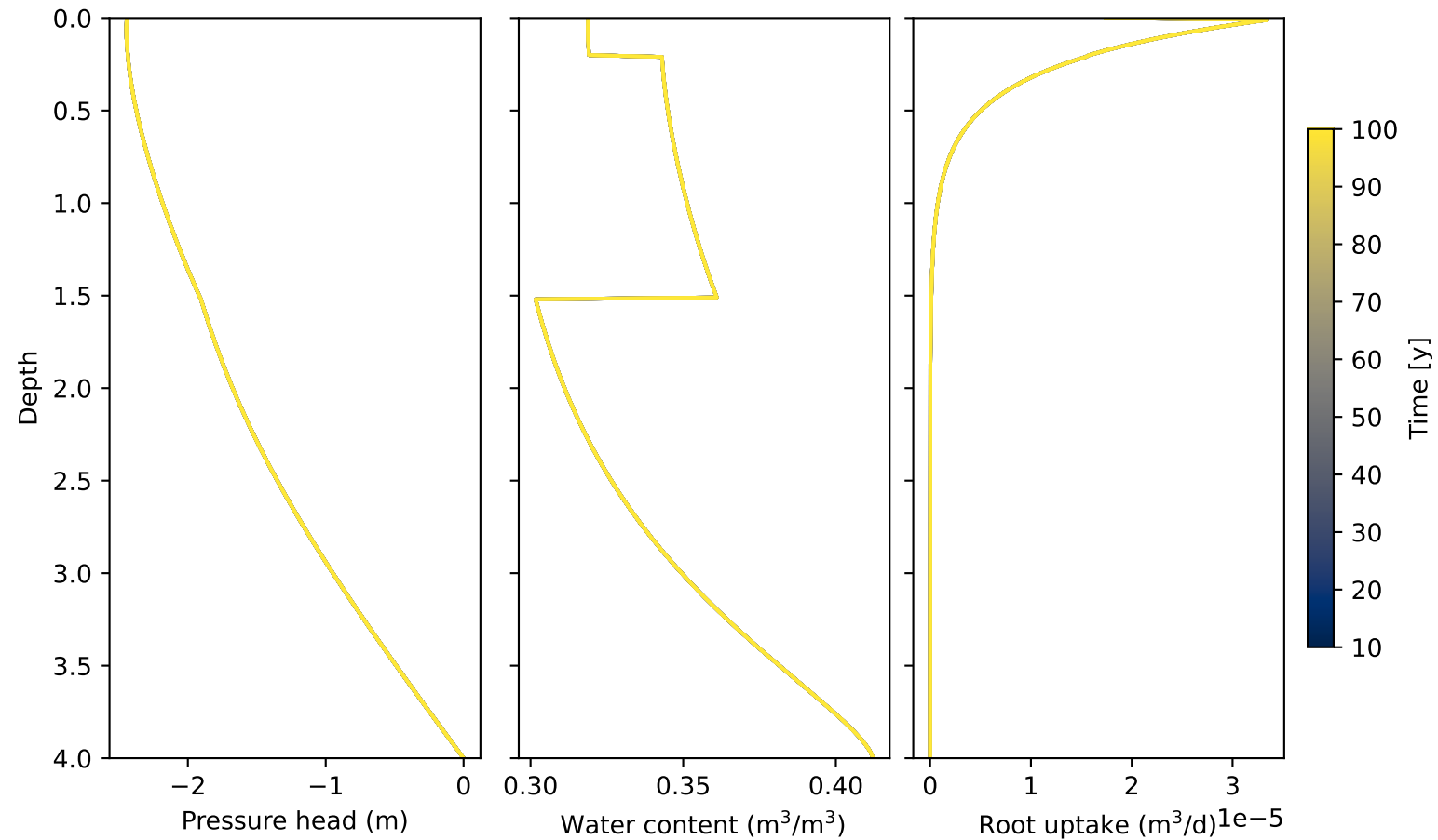
Kuma: Water content and root uptake
