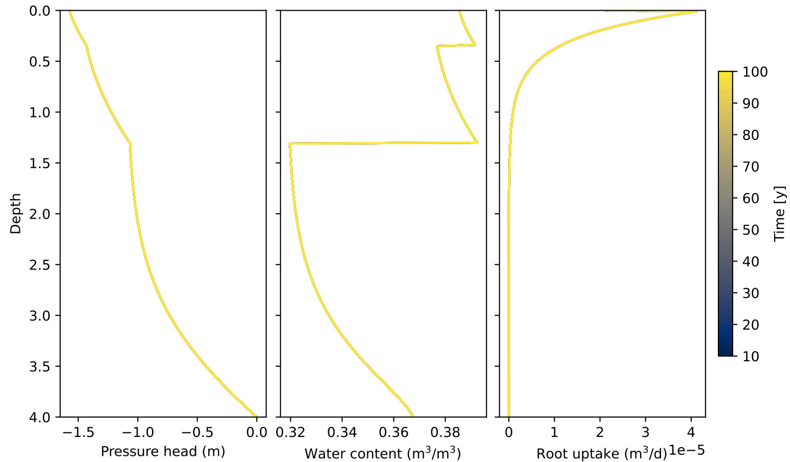
Flanagan: Water content and root uptake
