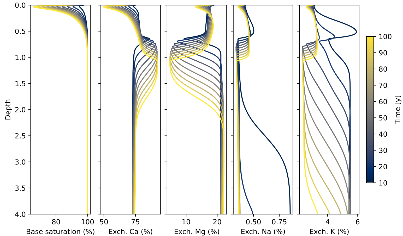
Palouse: Base saturation and exchange composition
