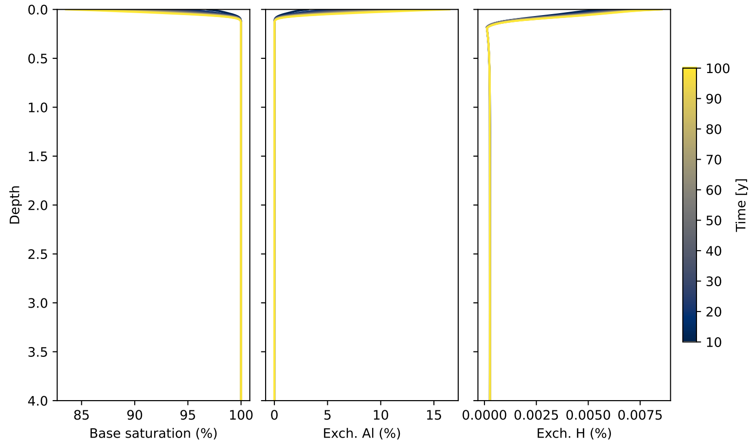
Pullman: Base saturation and exchangeable acidity
