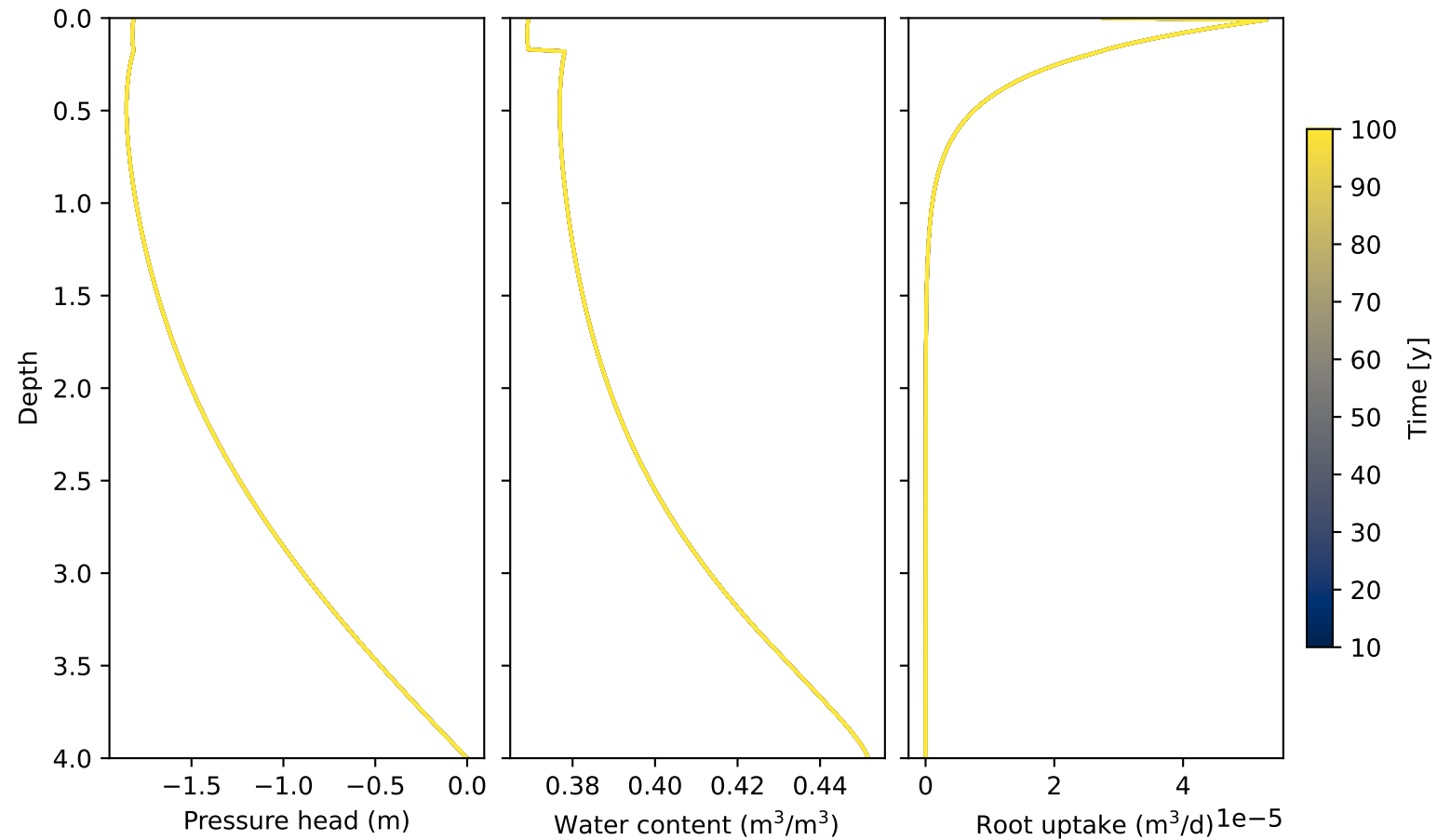
Pullman: Water content and root uptake
