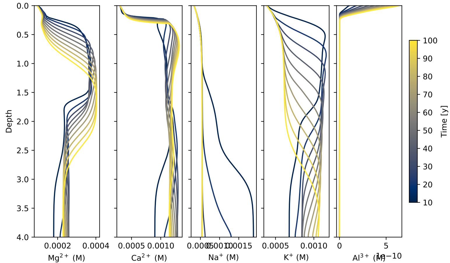
Kuma: Major cations
