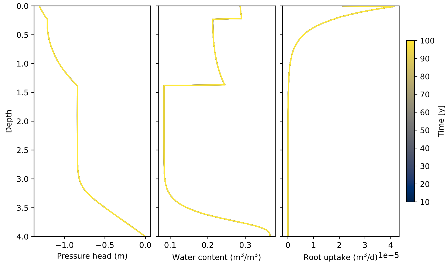
Kalamazoo: Water content and root uptake
