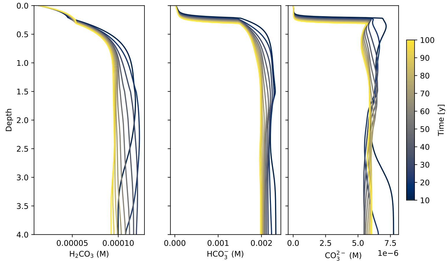
Kuma: Carbonate speciation
