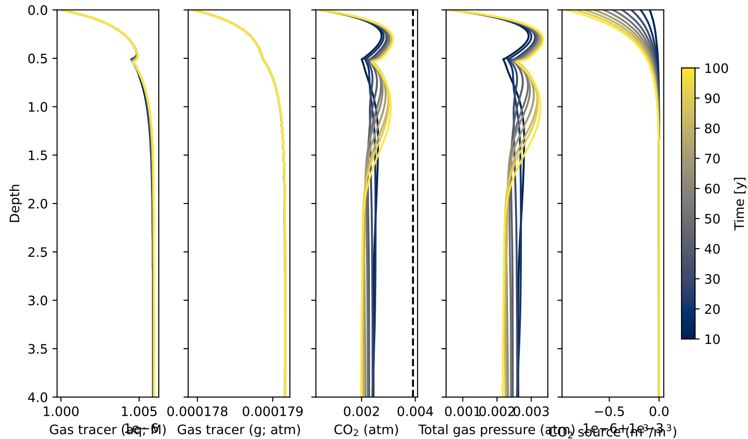
Yolo: CO 2 and gas tracer
