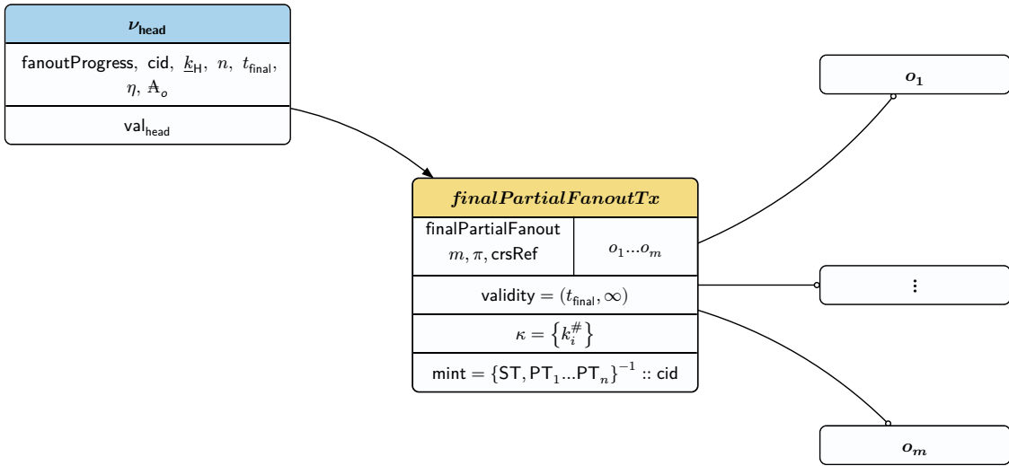
Figure 12: finalPartialFanout transaction spending the fanoutProgress head output, distributing the final batch of UTxOs o_1 \dots o_m , and burning all head tokens to reach final .
