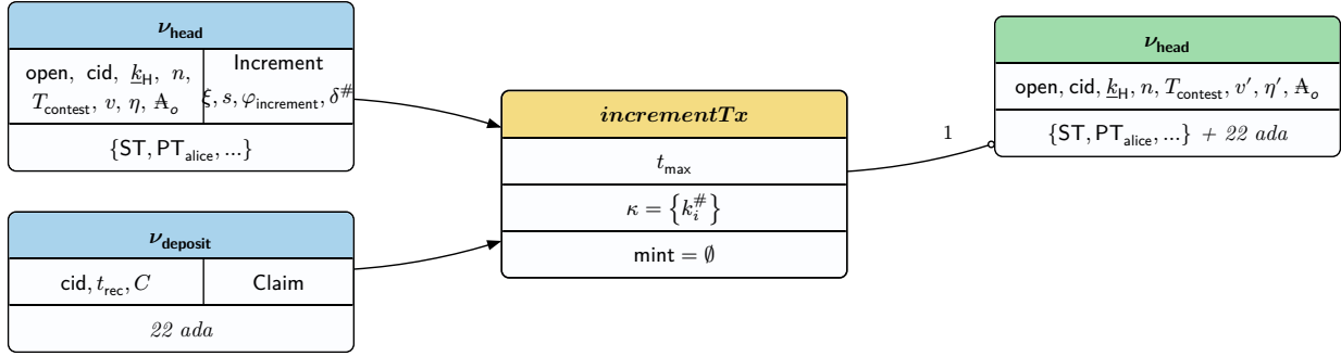
Figure 6: increment transaction spending an open head output, producing a new head output which includes the new UTxO.
