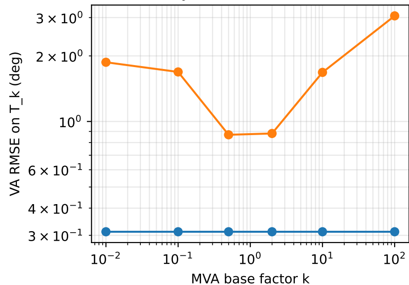
Accuracy on transformed test set
