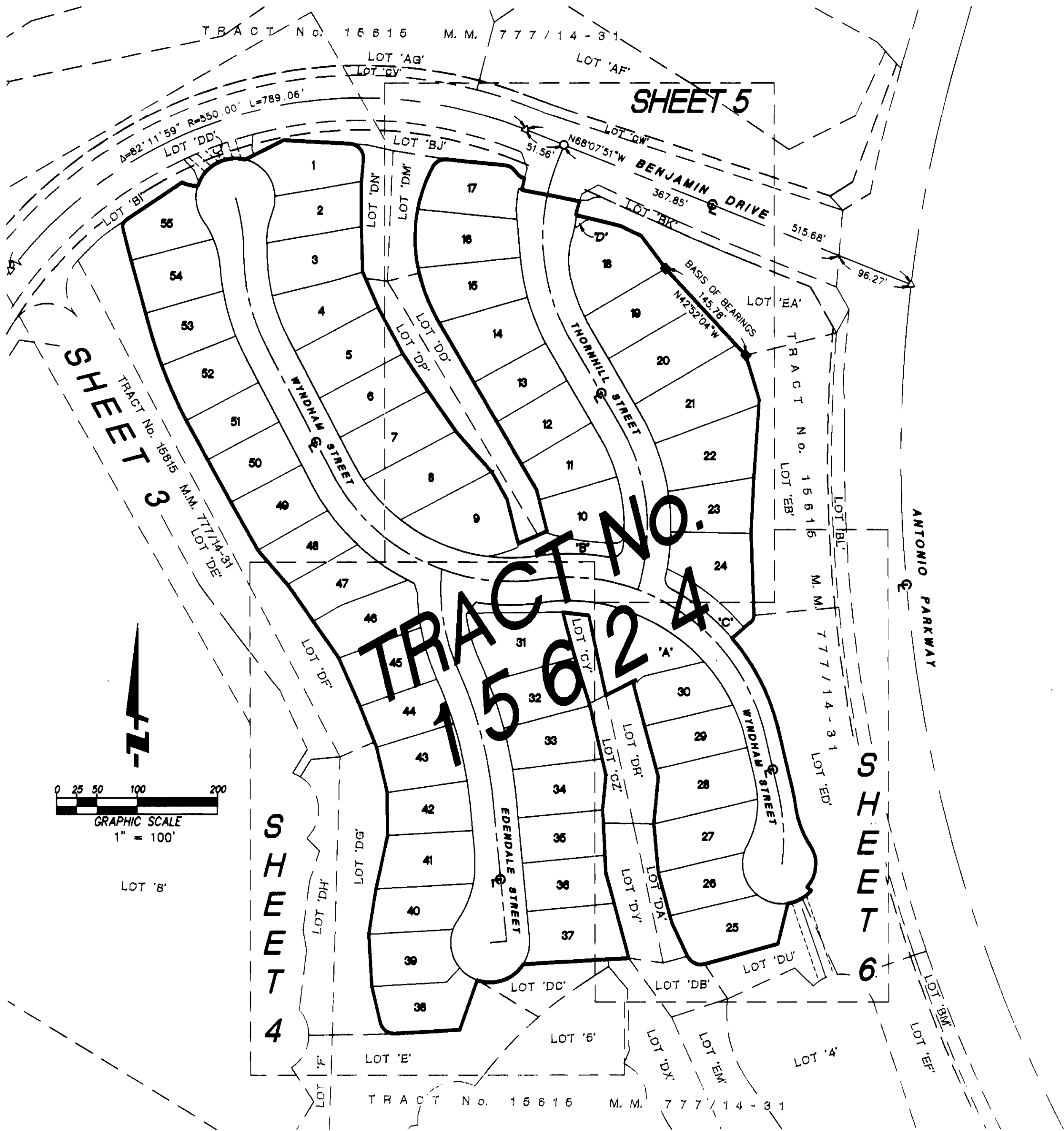
INDEX / VICINITY MAP
