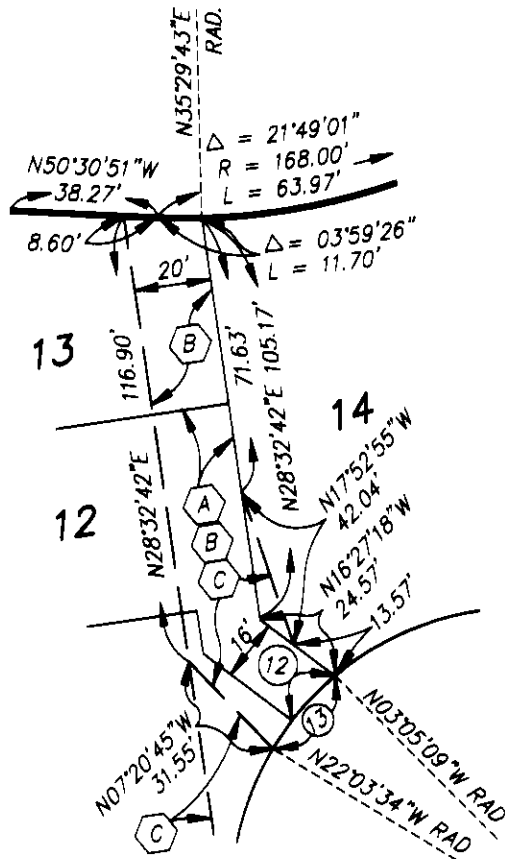
EASEMENT DETAIL
