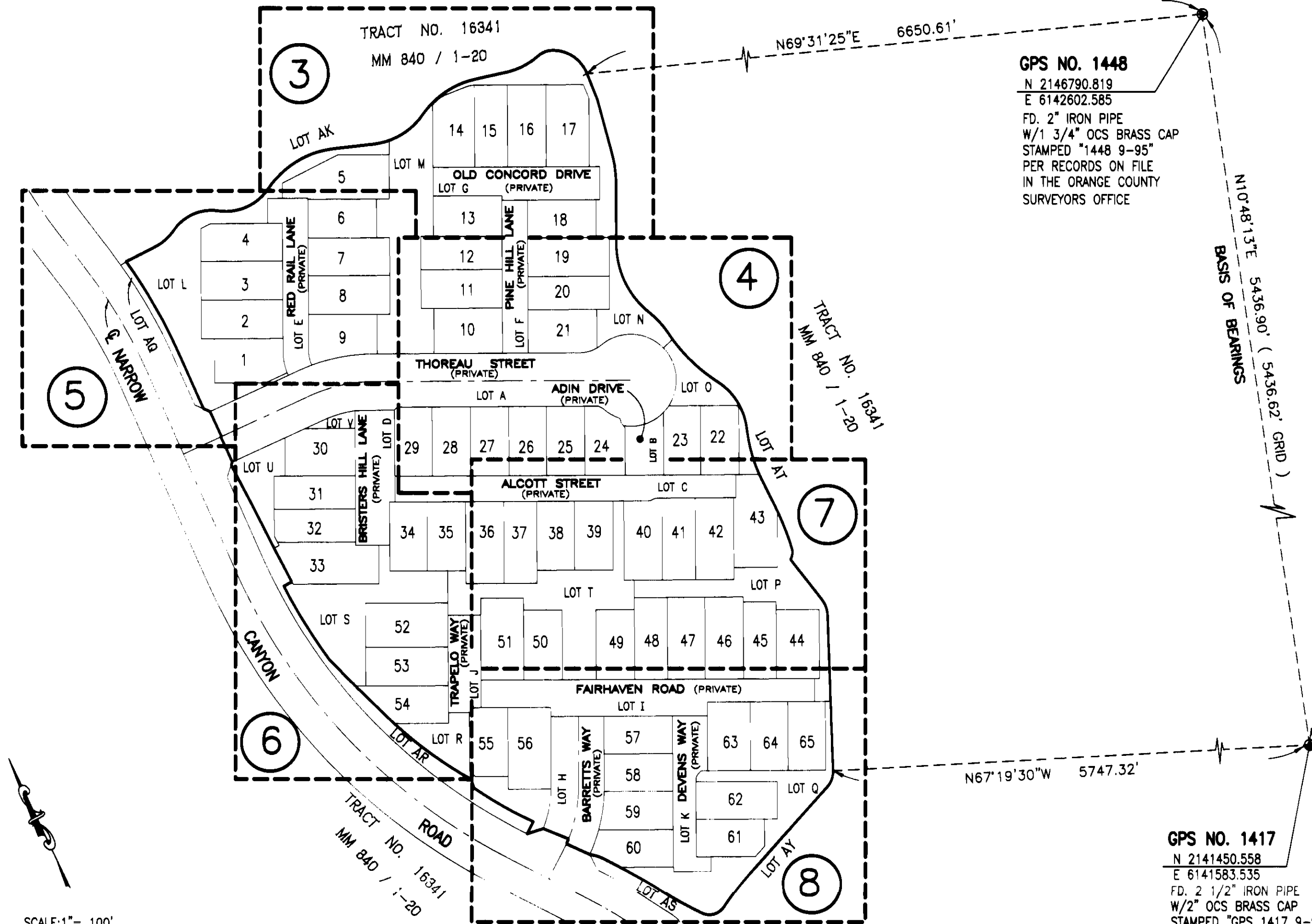
BOUNDARY CONTROL AND SHEET INDEX
