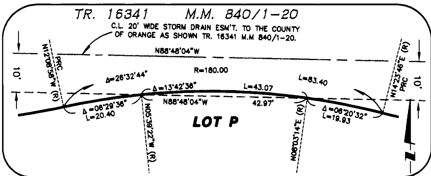
DETAIL 'F' NOT TO SCALE (SHEET 3)
