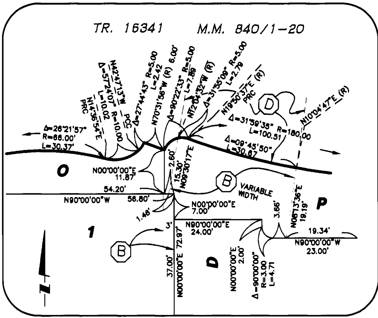
DETAIL 'A' NOT TO SCALE (SHEET 3)
