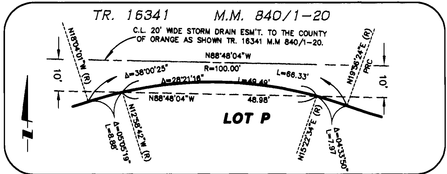
DETAIL 'G' NOT TO SCALE (SHEET 3)
