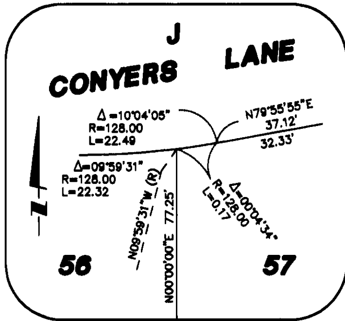
DETAIL 'B' NOT TO SCALE (SHEET 5)
