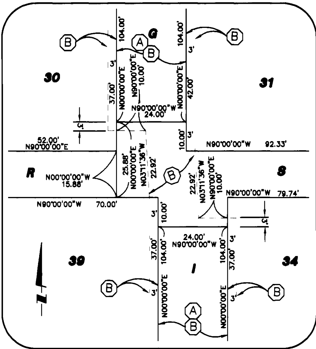
DETAIL 'D' NOT TO SCALE (SHEET 4)
