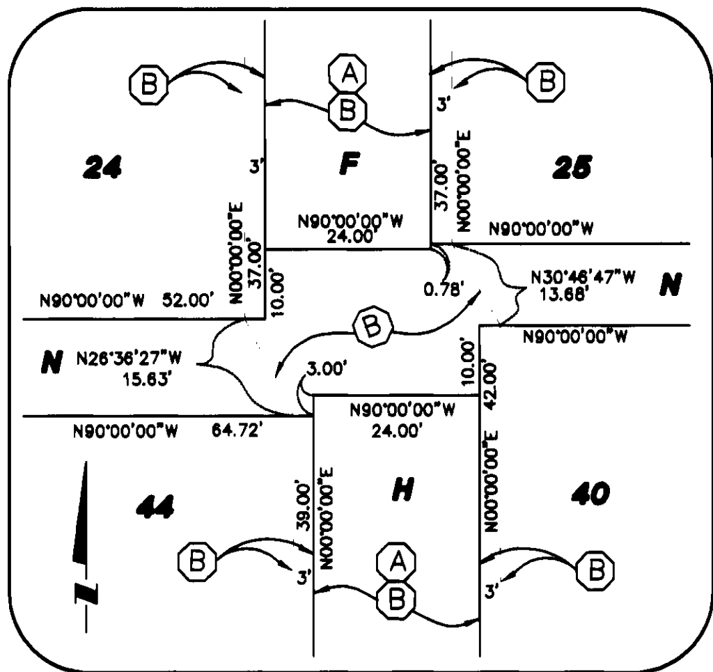
DETAIL 'E' NOT TO SCALE (SHEET 4)
