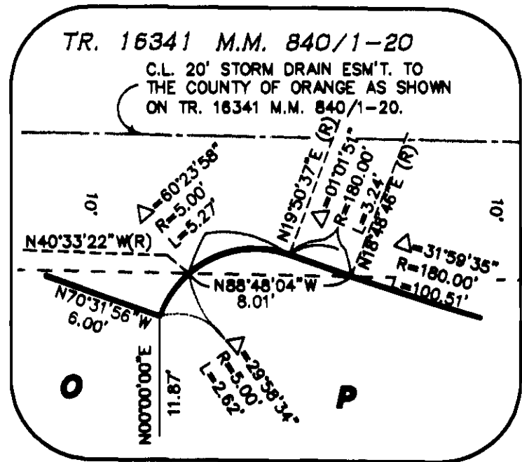
DETAIL 'C' NOT TO SCALE (SHEET 3)
