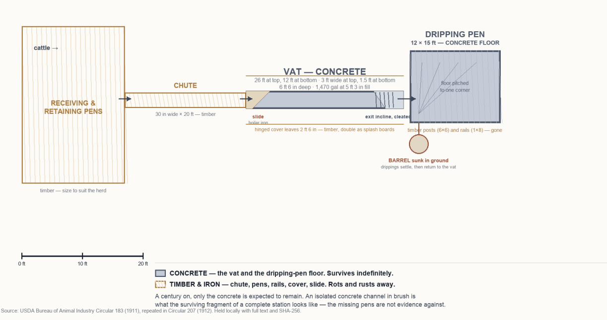
Scale plan of a complete 1911-specification station, drawn from the federal instructions. Every dimension is quoted from USDA Bureau of Animal Industry Circular 183 (1911), repeated in Circular 207 (1912). Solid = concrete; hatched = timber and iron.
