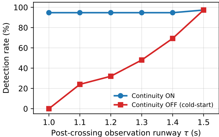
Detection rate vs. runway \tau
