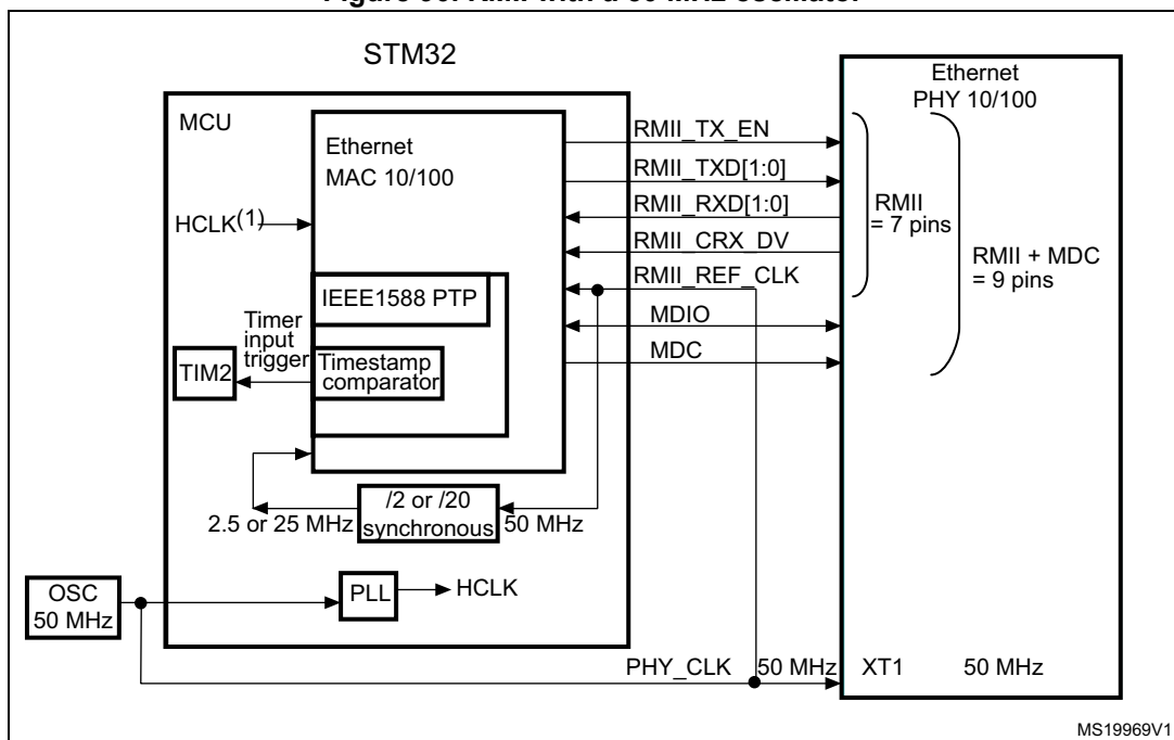
Figure 90. RMII with a 50 MHz oscillator
