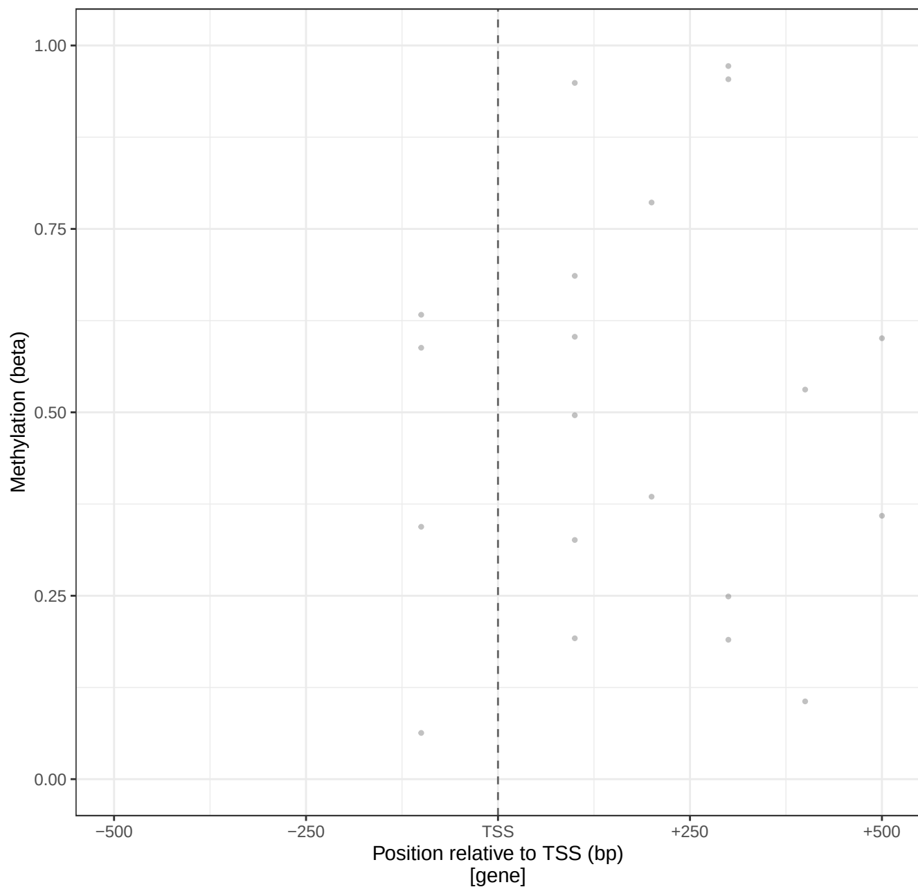
TSS methylation profile: gene ( \pm 500 bp)
