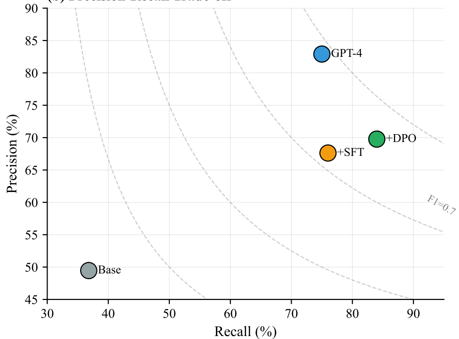
(b) Precision-Recall Trade-off
