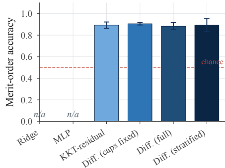
(c) Pairwise merit-order accuracy
