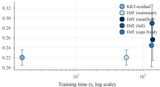
Accuracy-speed trade-off
