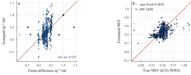
Fig. 7: Jacobian validation and downstream MEF accuracy on the 8-bus synthetic network. (a) Autograd vs. central finite-difference Jacobian entries on smooth rows (entries whose perturbation does not cross an active-set boundary). (b) Estimated vs. true MEFs; both the full (navy) and caps-fixed F&D (grey) estimators cluster around the y = x line with cosine 0.97. A small number of estimated MEFs are mildly negative: these are numerical artefacts from active-set transitions where the autograd Jacobian sign-flips across a kink in the merit-order map, not physical MEFs.
