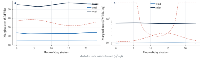
Fig. 6: Hour-resolved cost recovery on PJM-like data: dashed lines show true costs; solid lines show learned costs after the same affine calibration as Figure 5. The stratified estimator captures the wind/solar duck-curve shape and the gas peaking pattern.
