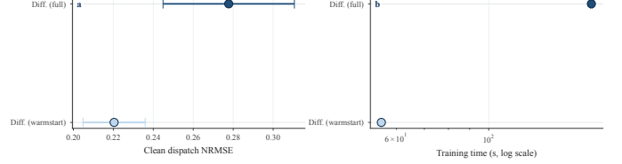
Fig. 10: KKT-warmstart vs. cold-start comparison (5 seeds, 95% CI), shown as horizontal dot plots so CI overlap is explicit. (a) Clean dispatch NRMSE; (b) wall-clock training time (log scale). Warmstart matches cold-start accuracy while reducing training time by 6\times .
