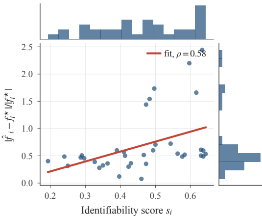
(a) Cost-vector identifiability
