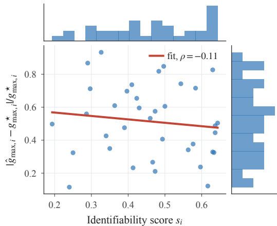
(b) Capacity identifiability
