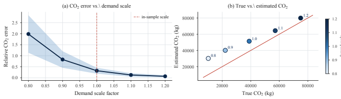
Fig. 13: Counterfactual CO 2 analysis across demand scale factors (5 seeds). (a) Relative CO 2 error vs. demand scale; error is lowest near the in-sample scale (dashed). (b) True vs. estimated CO 2 emissions; colour encodes demand scale.
