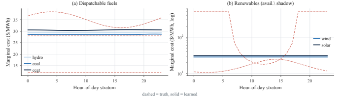
Fig. 6: Hour-resolved cost recovery on PJM-like data: dashed lines show true costs; solid lines show learned costs. The stratified estimator captures the wind/solar duck-curve shape and the gas peaking pattern.
