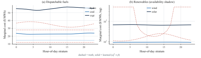
Fig. 6: Hour-resolved cost recovery on PJM-like data: dashed lines show true costs; solid lines show learned costs after the same affine calibration as Fig. 5. The stratified estimator captures the wind/solar duck-curve shape and the gas peaking pattern.
