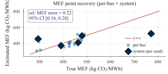
Fig. 14: MEF recovery across 5 seeds. Small navy points are per-bus MEFs ( 40 = 8 \text{ buses} \times 5 \text{ seeds} ), large diamond markers are system-wide MEFs per seed; rust line is y = x .
