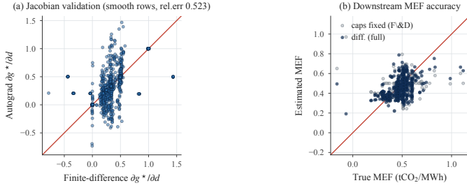
Fig. 7: Jacobian validation and downstream MEF accuracy on the 8-bus synthetic network. (a) Autograd vs. central finite-difference Jacobian entries on smooth rows (entries whose perturbation does not cross an active-set boundary). (b) Estimated vs. true MEFs; both the full (navy) and caps-fixed F&D (grey) estimators cluster around the y = x line with cosine 0.97.
