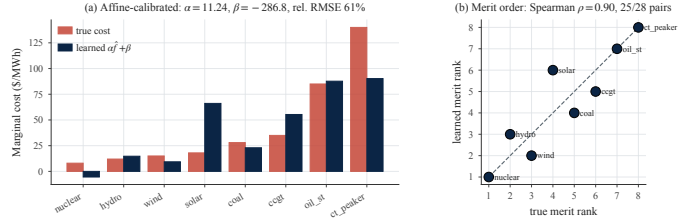
Fig. 5: PJM-like merit-order recovery. (a) True base costs (rust) vs. affinely calibrated learned costs \alpha \hat{f} + \beta (navy), sorted by truth. (b) Rank–rank plot of true vs. learned merit order. Costs are identifiable from dispatch only up to an affine transform on the demand-balanced subspace, so we calibrate once per run by OLS; the calibration does not change ordering metrics.
