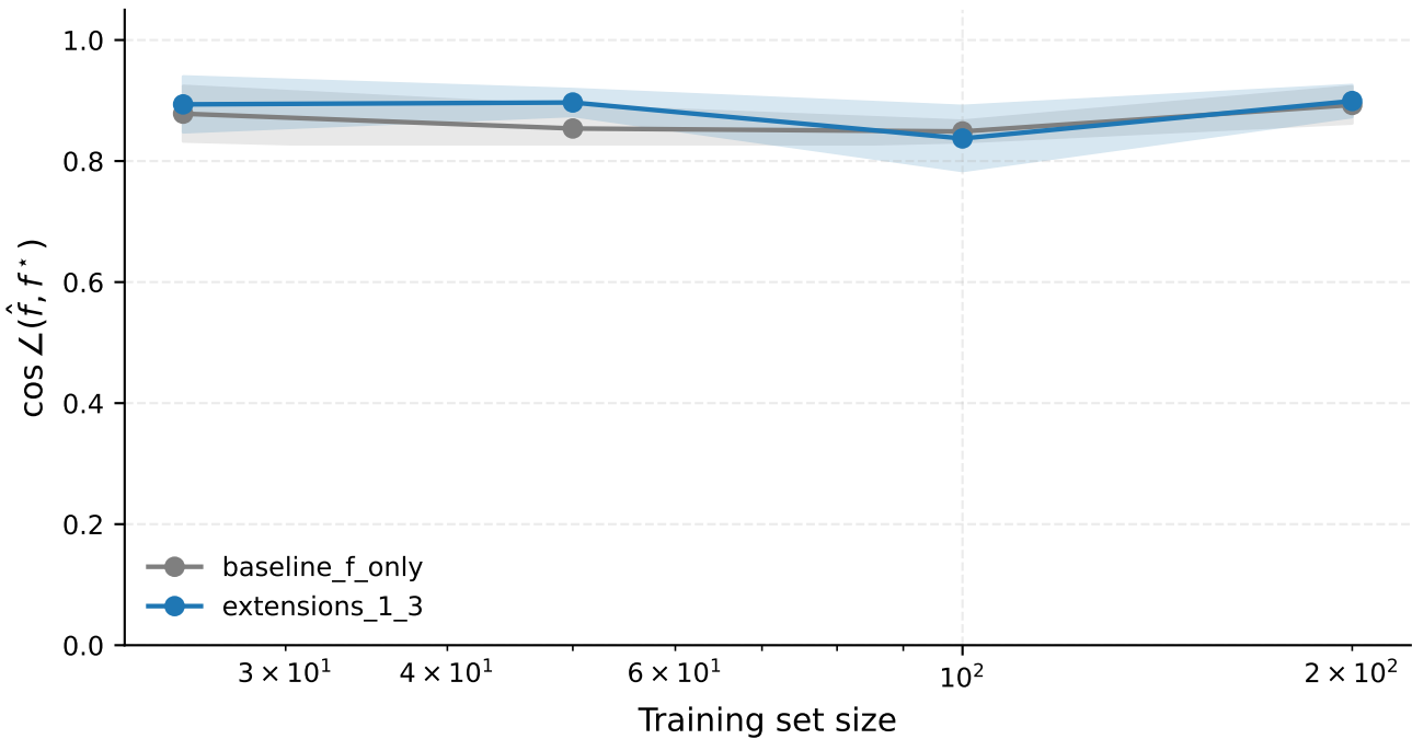
Cost recovery vs. dataset size (mean \pm 1 std, n=3 seeds)
