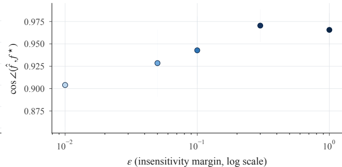
(b) Cost cosine vs. \epsilon
