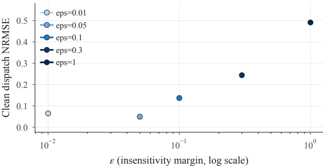
(a) NRMSE vs. \epsilon
