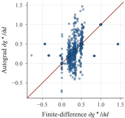
(a) Jacobian validation (smooth rows, rel.err 0.523)
