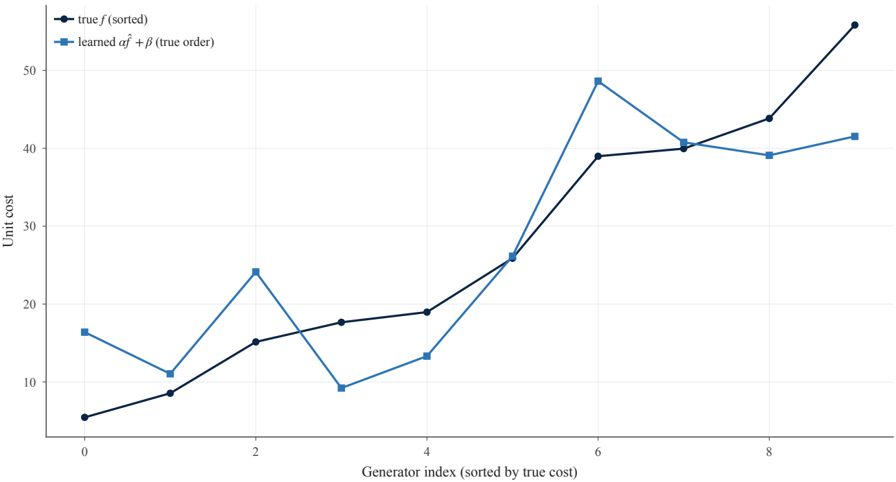
Merit-order recovery ( \alpha=5.95 , \beta=-88.21 )
