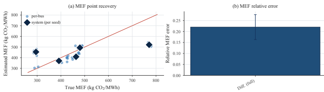
Fig. 14: MEF recovery across 5 seeds. (a) True vs. estimated MEFs: small navy points are per-bus MEFs (40 = 8 buses \times 5 seeds), large diamond markers are system-wide MEFs per seed. (b) Relative MEF error per method (95% CI).
