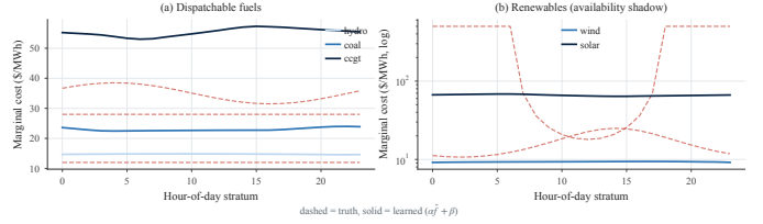
Fig. 6: Hour-resolved cost recovery on PJM-like data: dashed lines show true costs; solid lines show learned costs after the same affine calibration as Fig. 5. The stratified estimator captures the wind/solar duck-curve shape and the gas peaking pattern.
