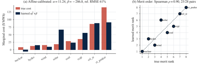
Fig. 5: PJM-like merit-order recovery. (a) True base costs (rust) vs. affinely calibrated learned costs \alpha\hat{f} + \beta (navy), sorted by truth. (b) Rank-rank plot of true vs. learned merit order. Costs are identifiable from dispatch only up to an affine transform on the demand-balanced subspace, so we calibrate once per run by OLS; the calibration does not change ordering metrics.
