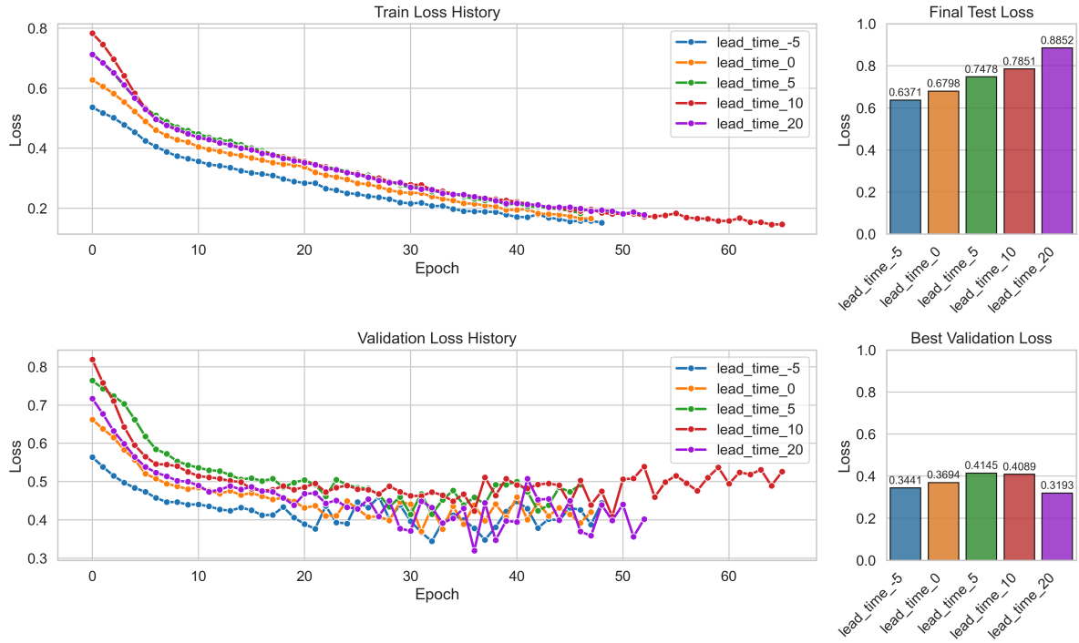
Figure 5.5: Training performance of models with varying lead time
