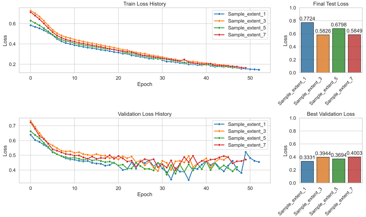
Figure 5.3: Training performance of models with varying sample length
