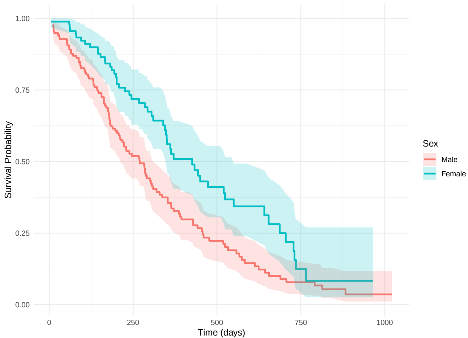
Kaplan–Meier Survival Curves by Sex
