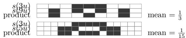
FIGURE 1. Two parity waves and their product; a cell is dark where the wave is -1 . The product's mean is exactly \text{gcd}(m, n)^2 / (mn) : one third for (3, 9) , one fifteenth for the coprime (3, 5) .
