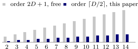
FIGURE 1. How much memory the slice census needs, by dimension D .
