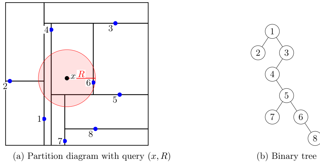
Figure 1: A two-dimensional k-d tree constructed by adding 8 random points from the unit cube [-1, 1]^2 .
