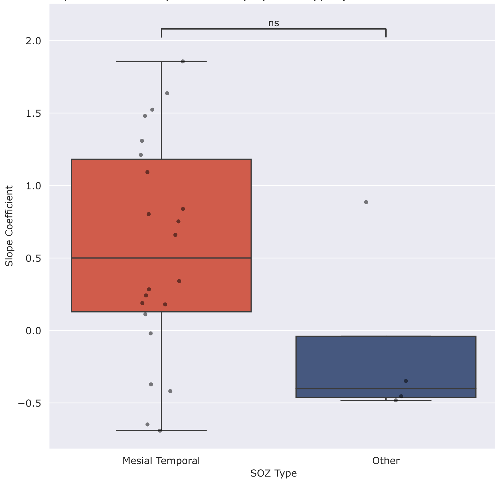
Distribution of Slope Coefficients (all contacts) by SOZ Type (Feature = recruitment_latency_t
