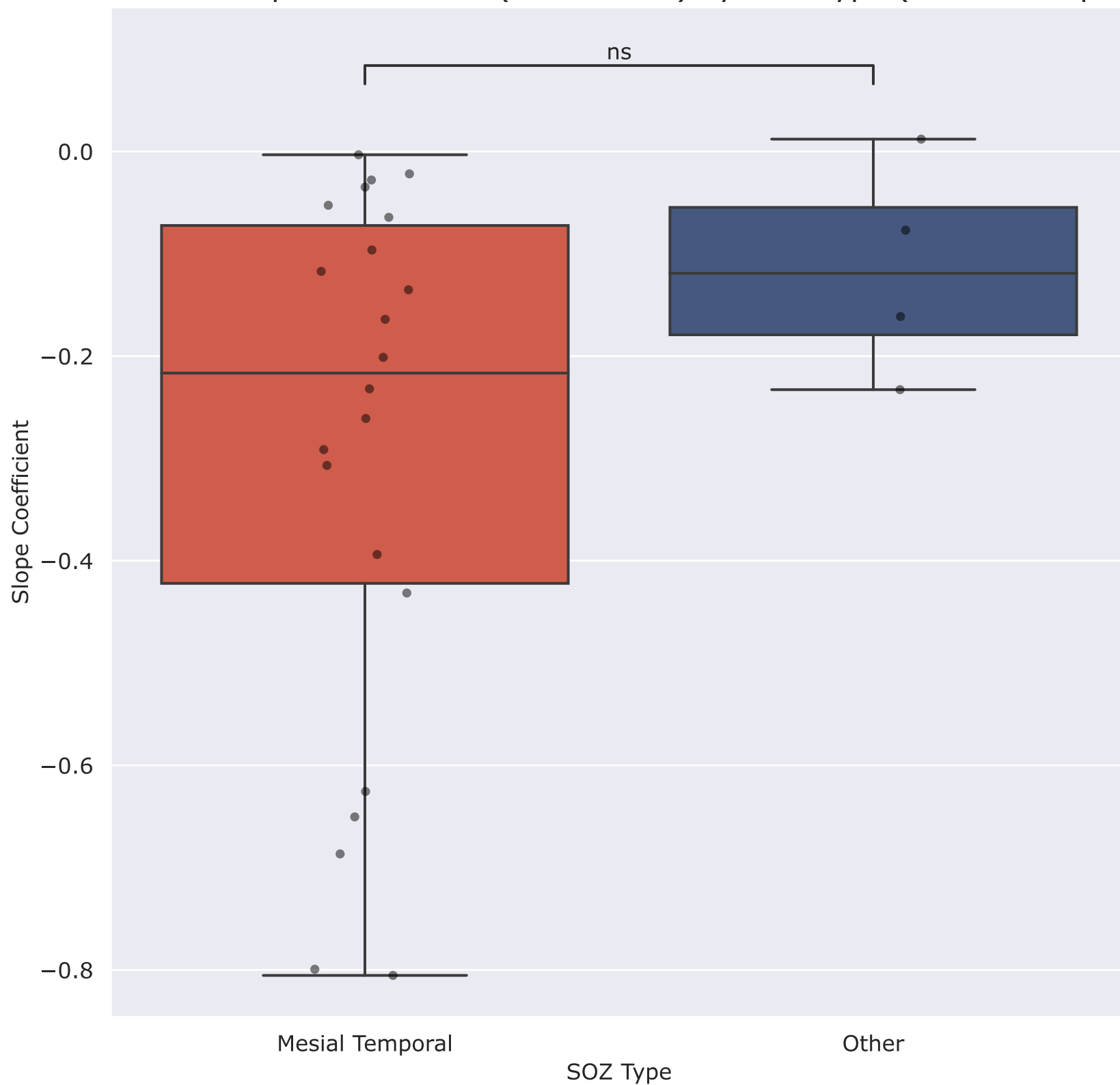
Distribution of Slope Coefficients (all contacts) by SOZ Type (Feature = spike_rate)
