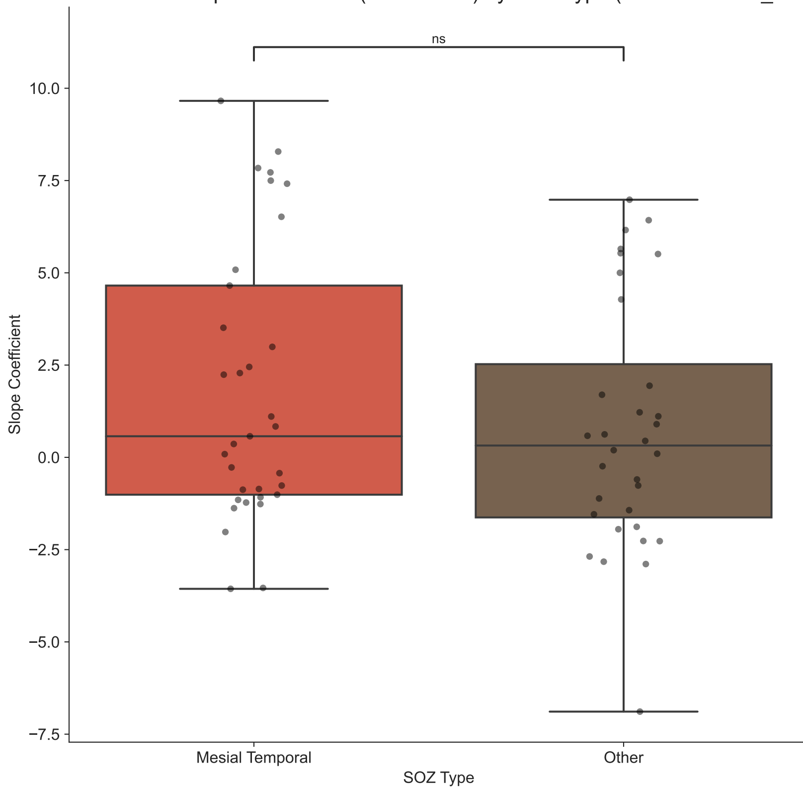
Distribution of Slope Coefficients (all contacts) by SOZ Type (Feature = slow_width)
