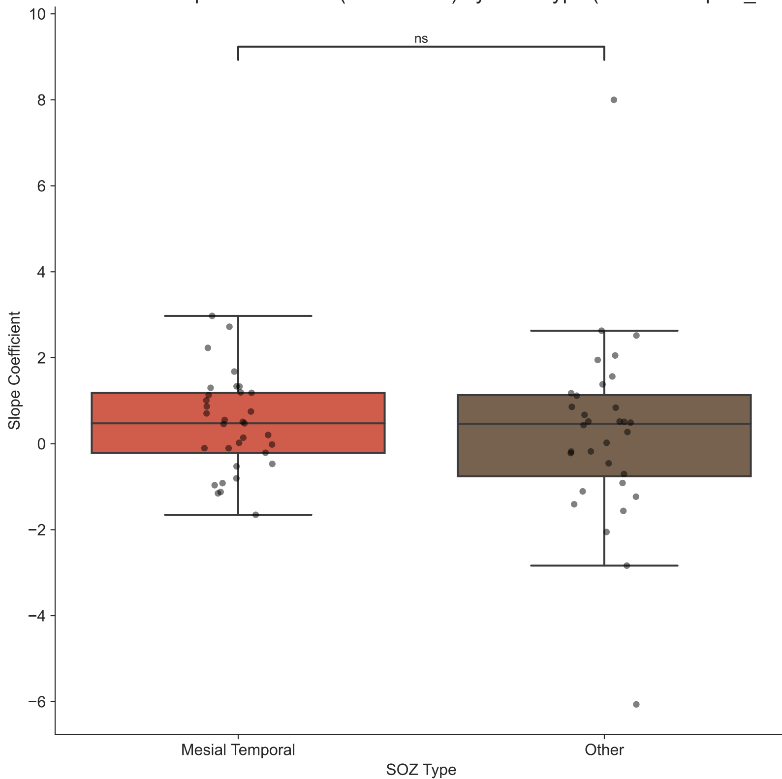
Distribution of Slope Coefficients (all contacts) by SOZ Type (Feature = spike_width)
