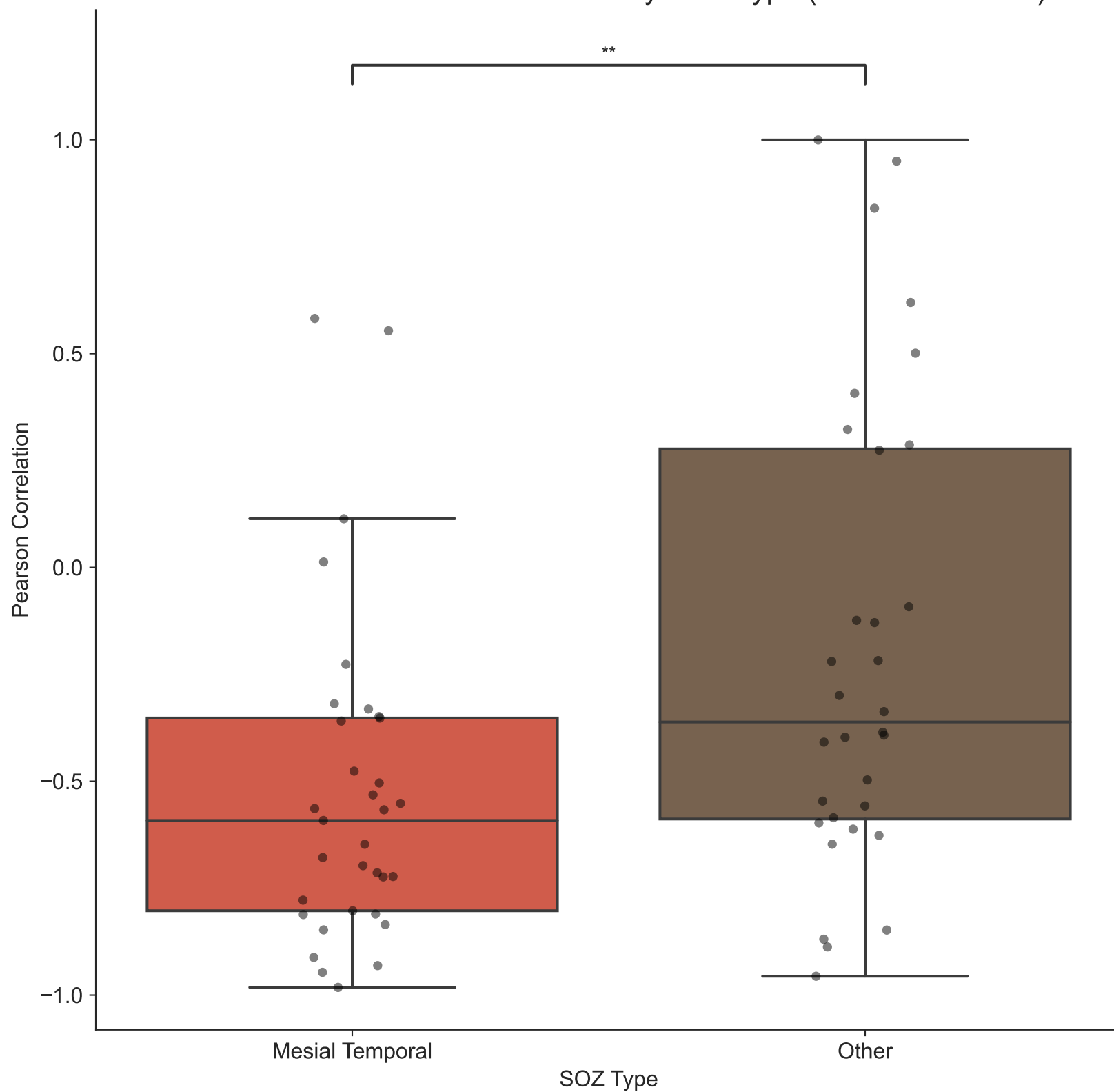
Distribution of Pearson Correlation by SOZ Type (Feature = linelen)
