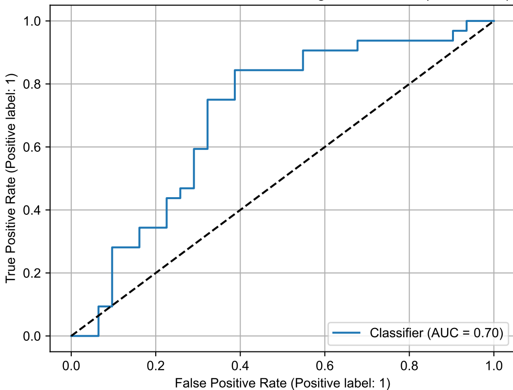
FPR vs. TPR ROC Curve of LR Testing Performance (all features)
