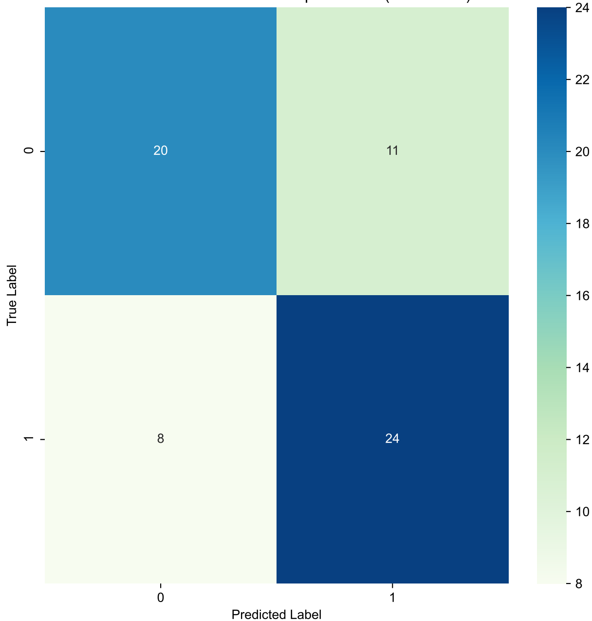
Confusion Matrix for LR test set predictions (all features)
