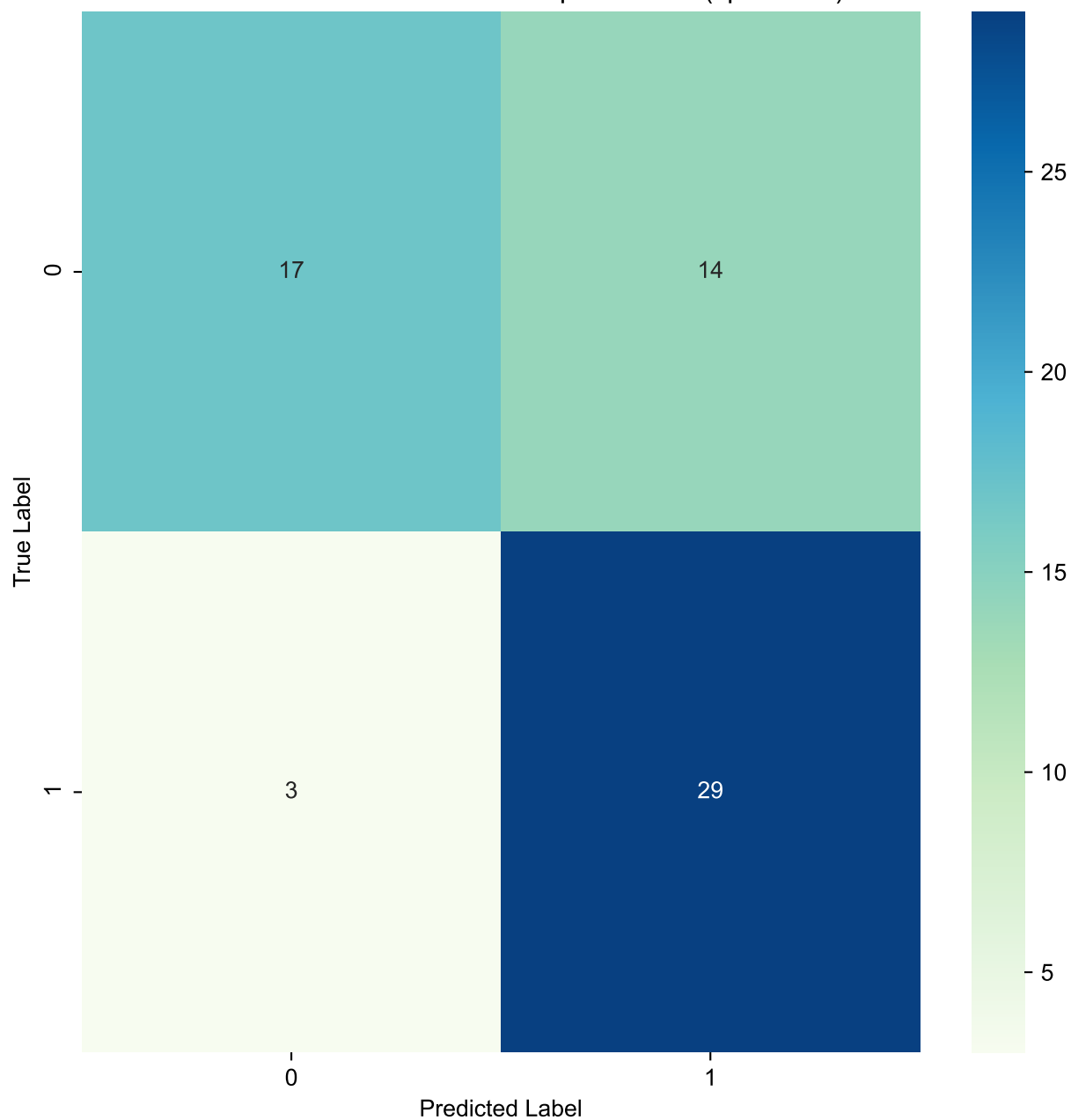
Confusion Matrix for LR test set predictions (spike rate)
