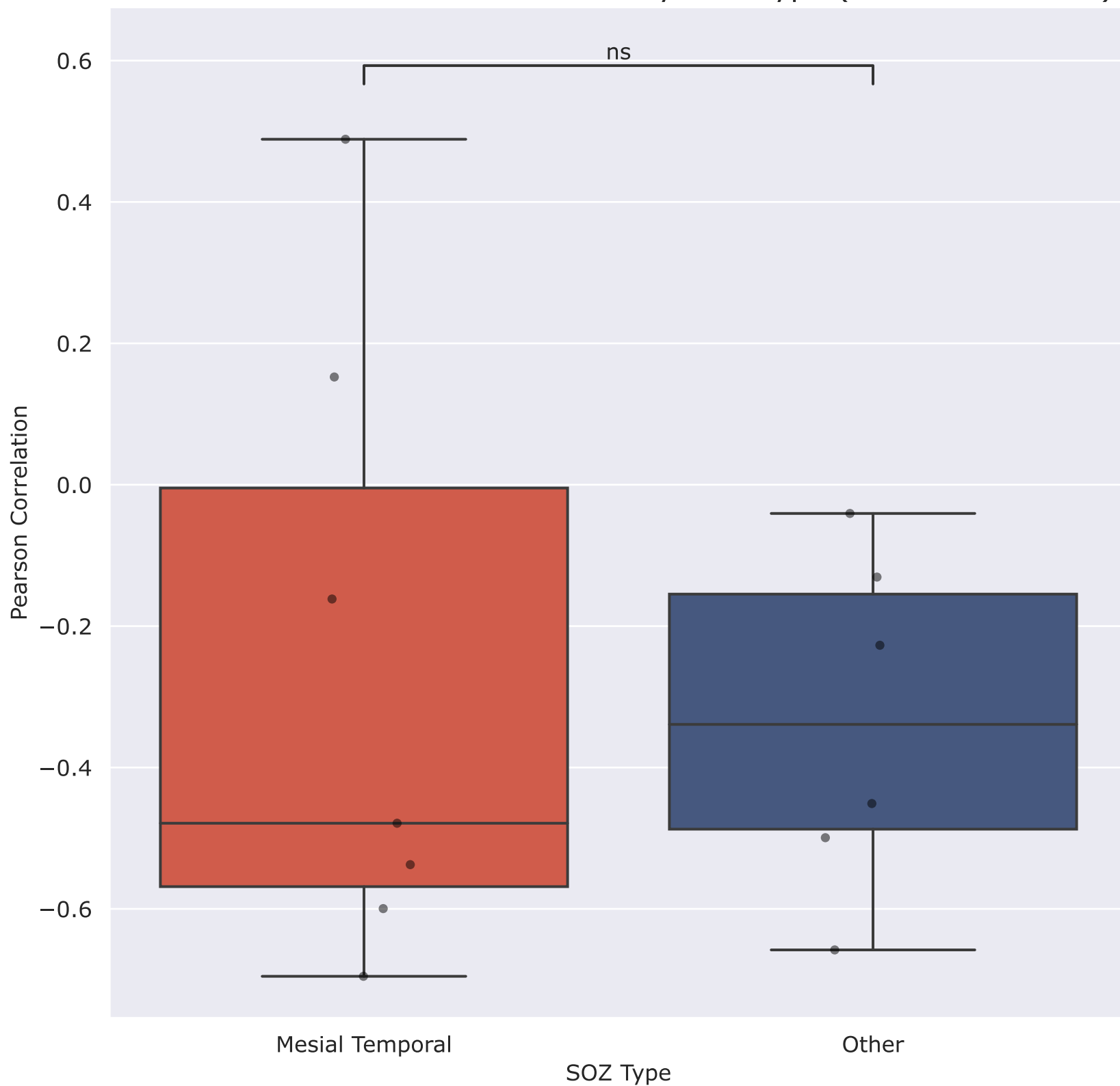
Distribution of Pearson Correlation by SOZ Type (Feature = linelen)
