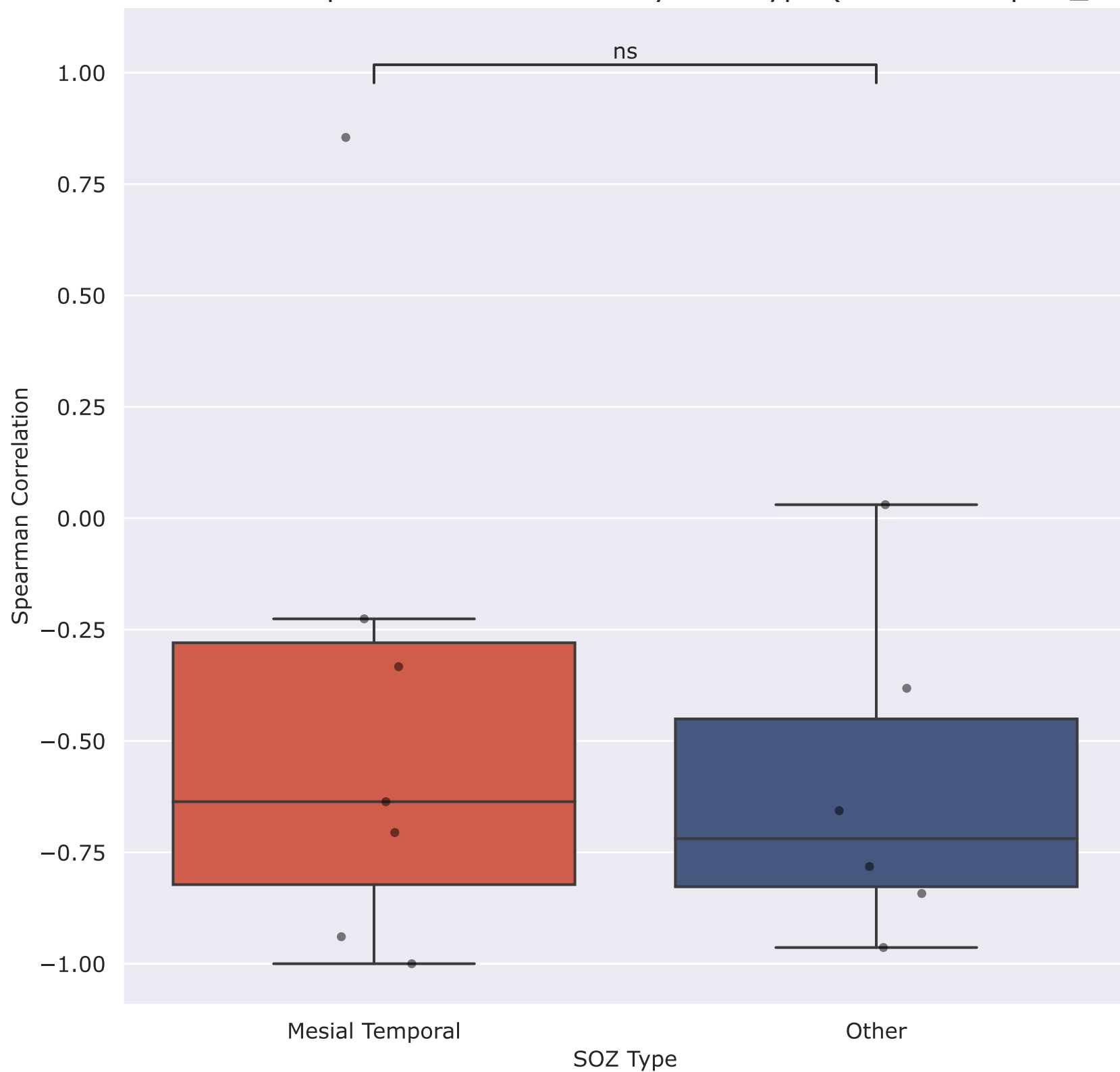
Distribution of Spearman Correlation by SOZ Type (Feature = spike_rate)
