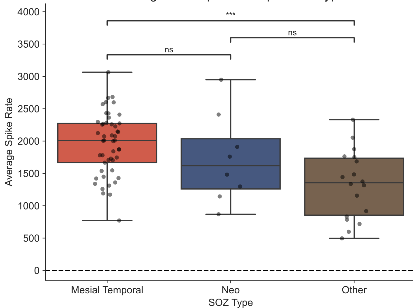
Average MTL Spike Rate per SOZ type
