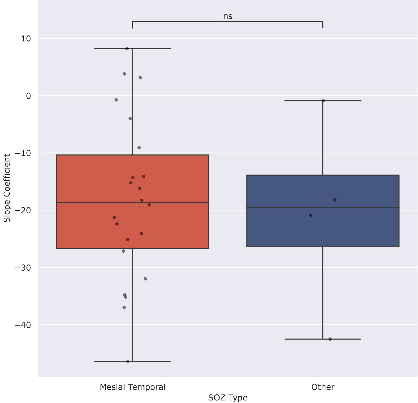
Distribution of Slope Coefficients (all contacts) by SOZ Type (Feature = slow_amp)
