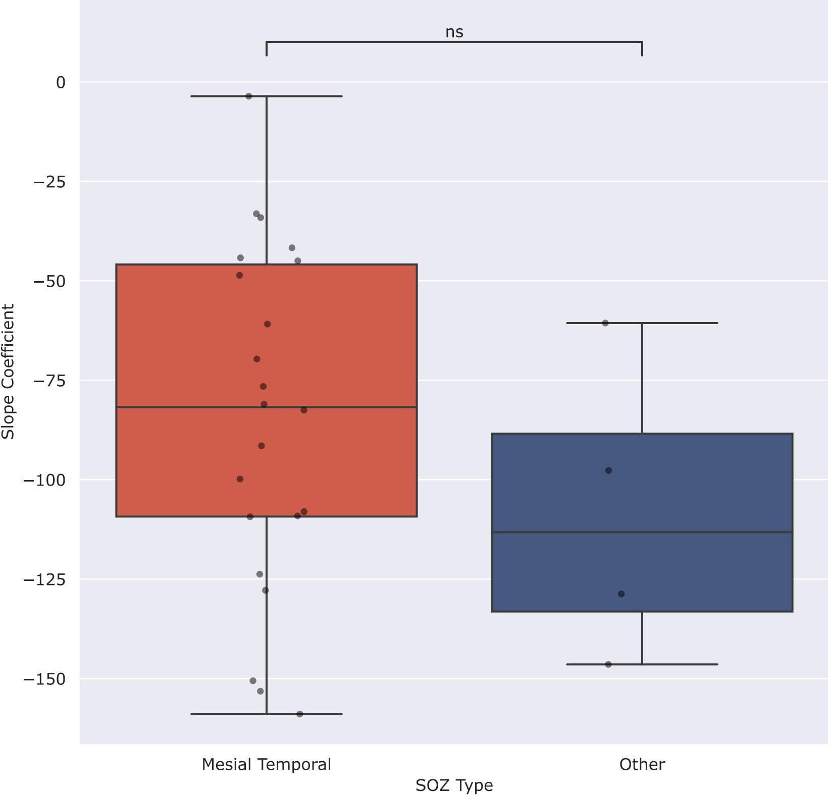
Distribution of Slope Coefficients (MTL contacts) by SOZ Type (Feature = rise_amp)
