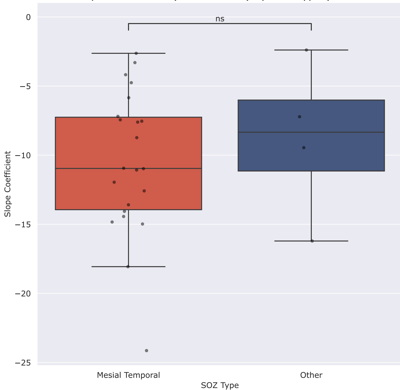
Distribution of Slope Coefficients (MTL contacts) by SOZ Type (Feature = sharpness)
