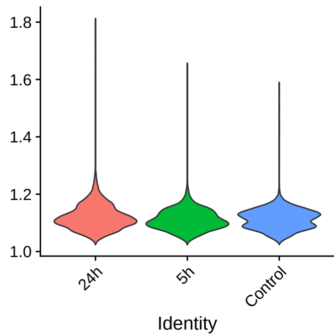
log10GenesPerUMI
