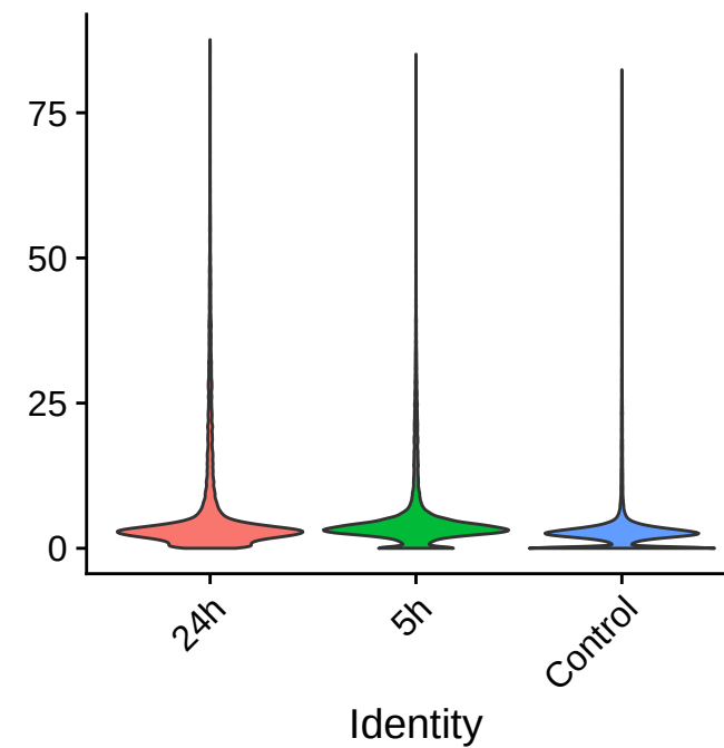
pMito
