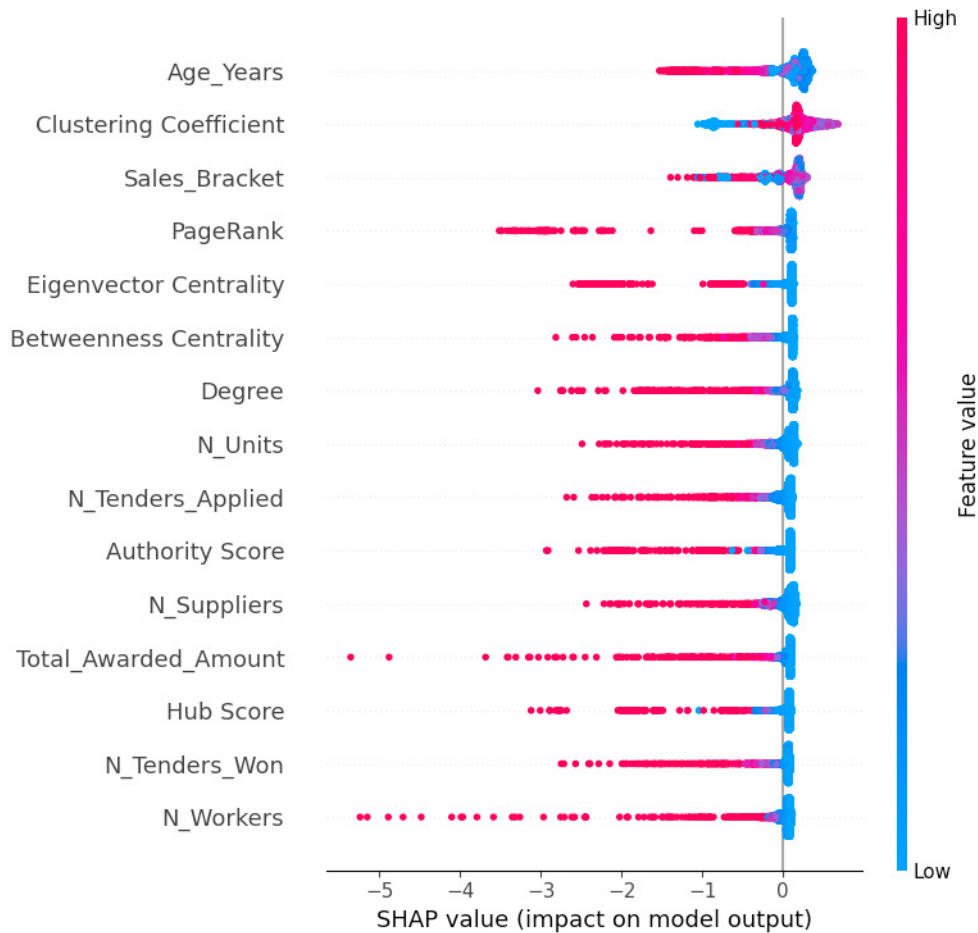
Fig. 1: Supplier Model Summary Plot: SHAP values analysis for the node level model, illustrating the impact of different features in detecting anomalous suppliers.
