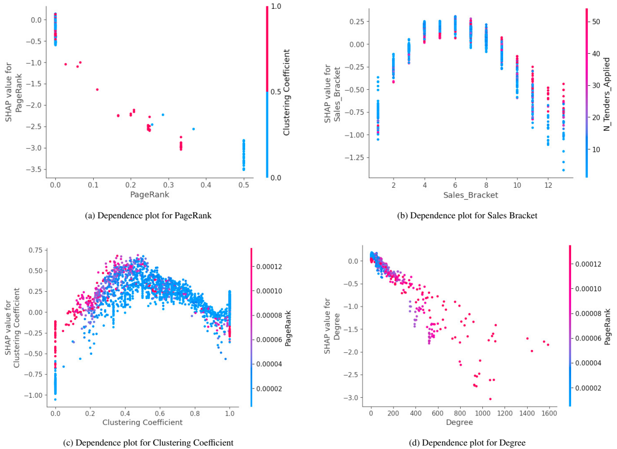
Fig. 2: SHAP dependence plots for key features in the supplier model.
