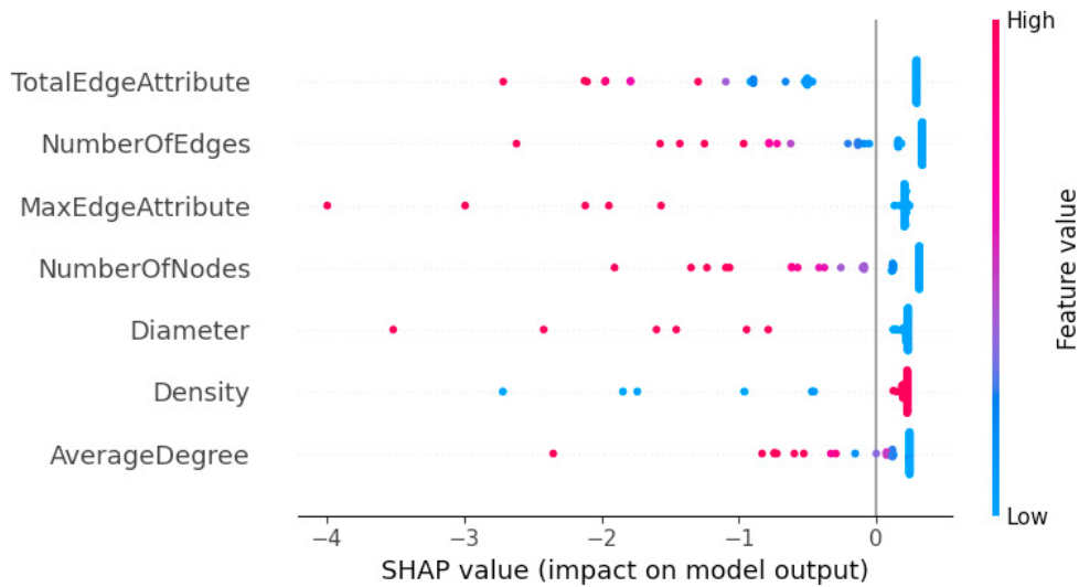
Fig. 3: Connected Components Model Summary Plot: SHAP values analysis for connected components level model, highlighting feature importance in anomaly detection.
